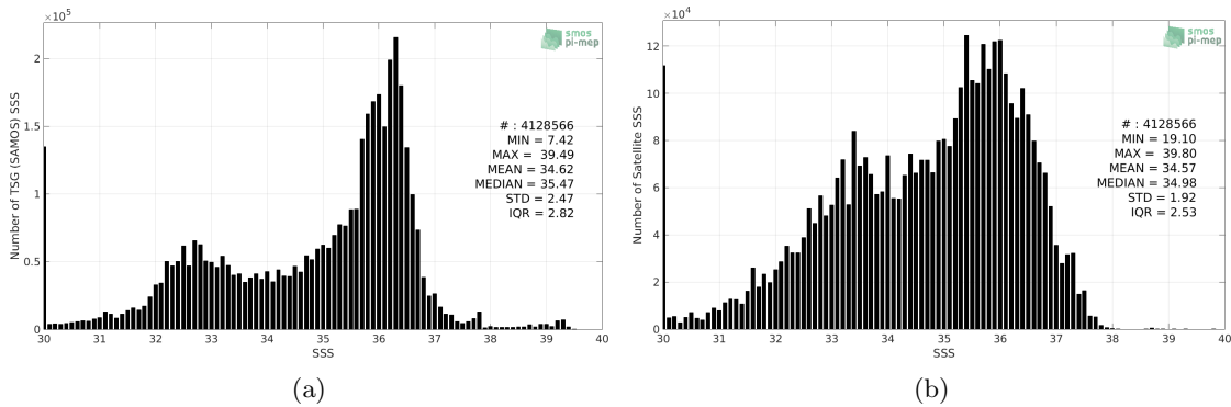
Figure 2: Histograms of SSS from TSG (SAMOS) (a) and SMOS SSS L3 v2 - Monthly - 0.25 Deg (CATDS-CECOS-IFREMER) (b) considering all match-up pairs per bins of 0.1 over the North Atlantic Ocean Pi-MEP region and for the full satellite product period.
