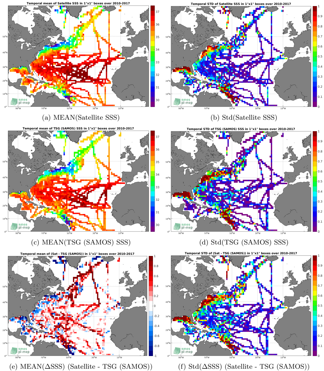
Figure 6: Temporal mean (left) and Std (right) of SSS from SMOS SSS L3 v2 - Monthly - 0.25 Deg (CATDS-CECOS-IFREMER) (top), TSG (SAMOS) (middle), and of \Delta SSS (Satellite - TSG (SAMOS)). Only match-up pairs are used to generate these maps.
