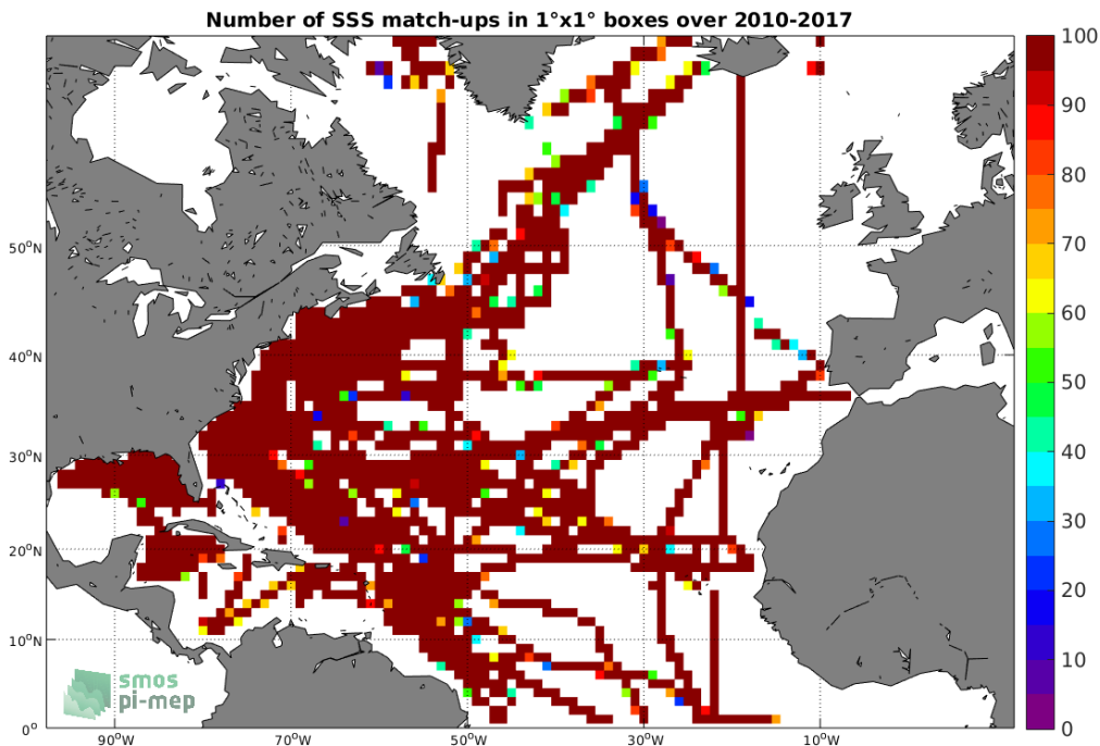
Figure 4: Number of SSS match-ups between TSG (SAMOS) SSS and the SMOS SSS L3 v2 - Monthly - 0.25 Deg (CATDS-CECOS-IFREMER) SSS product for the North Atlantic Ocean Pi-MEP region over 1^\circ \times 1^\circ boxes and for the full satellite product period.
