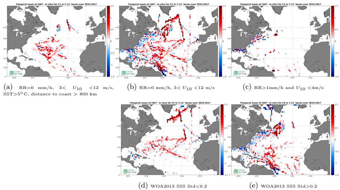
Figure 12: Temporal mean gridded over spatial boxes of size 1^\circ \times 1^\circ of \Delta\text{SSS} (SMOS SSS L3 v2 - Monthly - 0.25 Deg (CATDS-CECOS-IFREMER) - TSG (SAMOS)) for 5 different subdatasets corresponding to:RR=0 mm/h, 3 < U_{10} < 12 m/s, SST >5^\circ\text{C} , distance to coast > 800 km (a), RR=0 mm/h, 3 < U_{10} < 12 m/s (b), RR >1 mm/h and U_{10} < 4 m/s (c), WOA2013 SSS Std <0.2 (d), WOA2013 SSS Std >0.2 (e).
