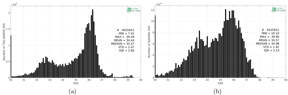
Figure 2: Histograms of SSS from TSG-SAMOS (a) and SMOS L3 v2 - Monthly - 0.25 Deg (CATDS-CECOS-IFREMER) (b) considering all match-up pairs per bins of 0.1 over the North Atlantic Ocean Pi-MEP region and for the full satellite product period.
