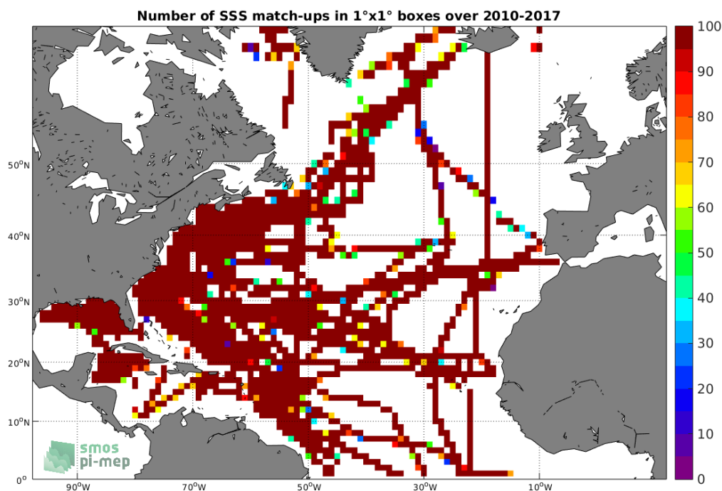
Figure 4: Number of SSS match-ups between TSG-SAMOS SSS and the SMOS L3 v2 - Monthly - 0.25 Deg (CATDS-CECOS-IFREMER) SSS product for the North Atlantic Ocean Pi-MEP region over 1^\circ \times 1^\circ boxes and for the full satellite product period.
