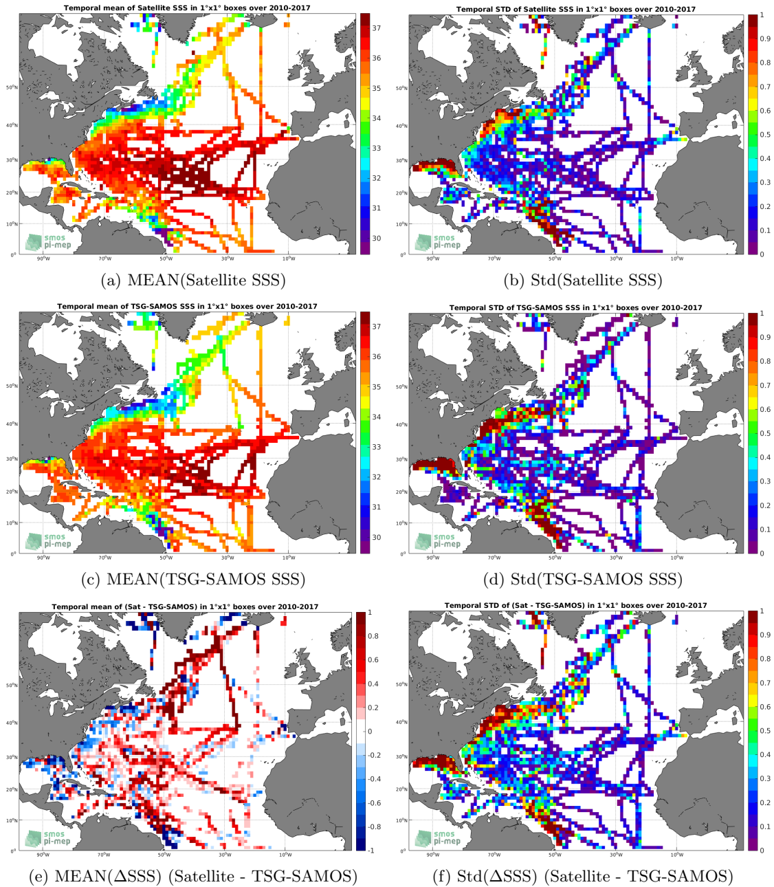
Figure 6: Temporal mean (left) and Std (right) of SSS from SMOS L3 v2 - Monthly - 0.25 Deg (CATDS-CECOS-IFREMER) (top), TSG-SAMOS (middle), and of \Delta SSS (Satellite - TSG-SAMOS). Only match-up pairs are used to generate these maps.
