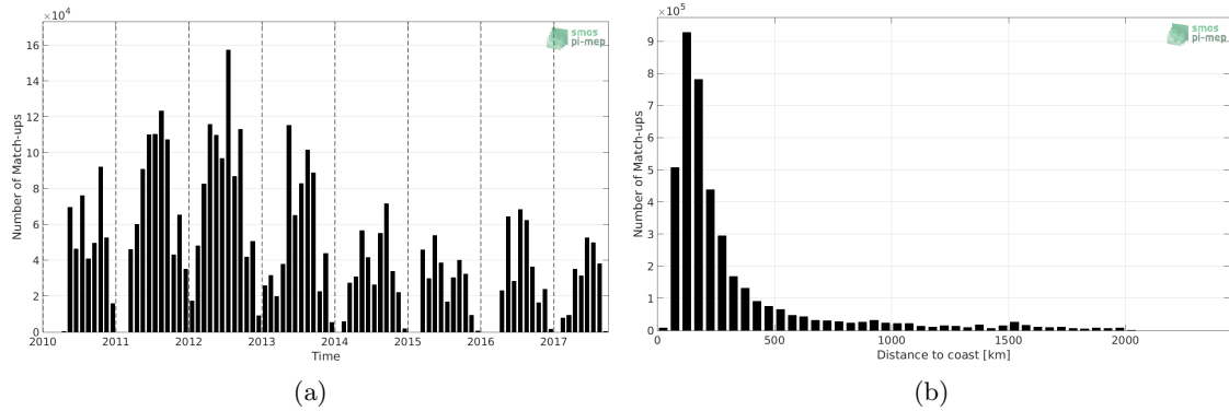
Figure 1: Number of match-ups between TSG-SAMOS and SMOS L3 v2 - Monthly - 0.25 Deg (CATDS-CECOS-IFREMER) SSS as a function of time (a) and as function of the distance to coast (b) over the North Atlantic Ocean Pi-MEP region and for the full satellite product period.
