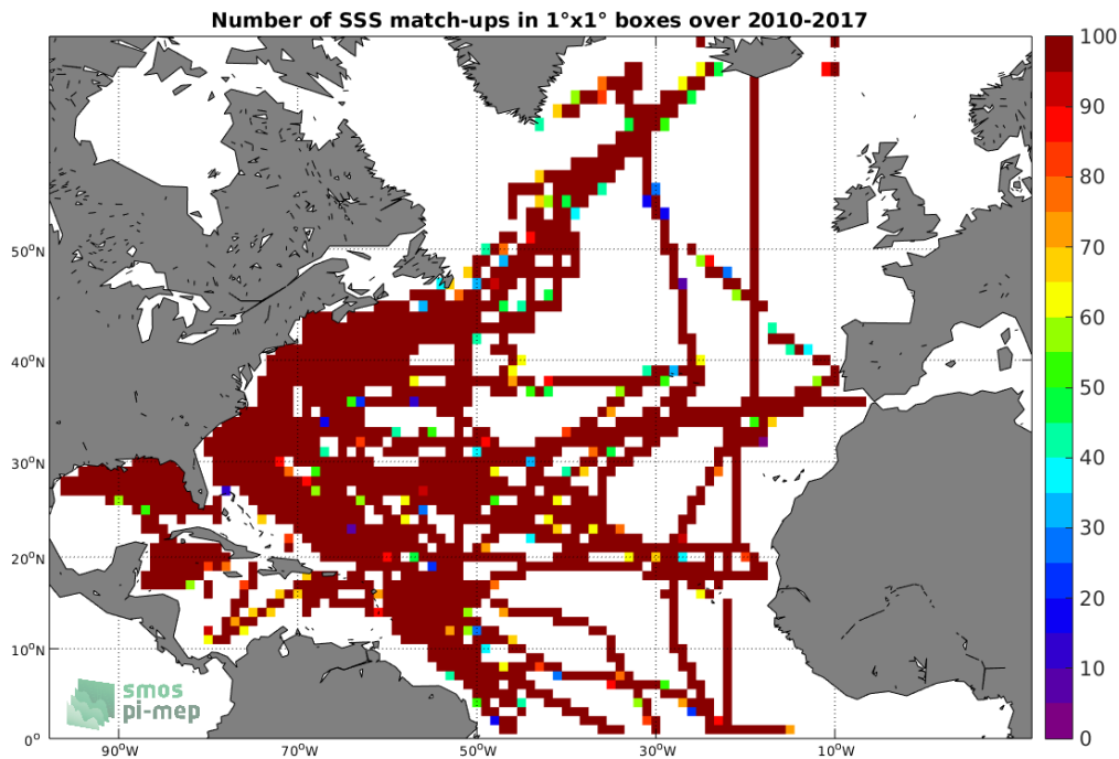
Figure 4: Number of SSS match-ups between TSG-SAMOS SSS and the SMOS-L3-CATDS-IFREMER-CECOS-V2-MONTHLY-0.25DEG SSS product for the North Atlantic Ocean Pi-MEP region over 1°x1° boxes and for the full satellite product period.
