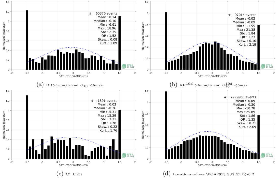
Figure 13: Normalized histogram of \Delta SSS (SMOS-L3-CATDS-IFREMER-CECOS-V2-MONTHLY-0.25DEG - TSG-SAMOS) for 6 different subdatasets corresponding to: RR > 1\text{mm/h} and U_{10} < 5\text{m/s} (a), RR^{10d} > 5\text{mm/h} and U_{10}^{10d} < 5\text{m/s} (b), C1 \cup C2 (c), Locations where WOA2013 SSS STD > 0.2 (d).
