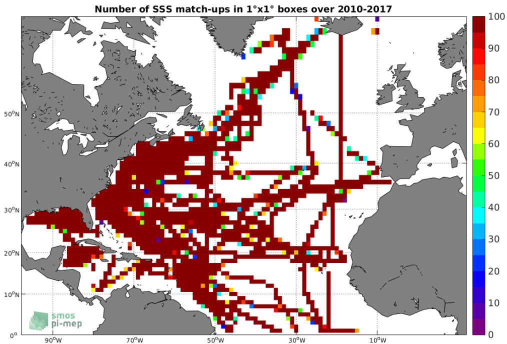
Figure 4: Number of SSS match-ups between TSG-SAMOS SSS and the SMOS-L3-CATDS-IFREMER-CECOS-V2-MONTHLY-0.25DEG SSS product for the North Atlantic Ocean Pi-MEP region over 1^\circ \times 1^\circ boxes and for the full satellite product period.
