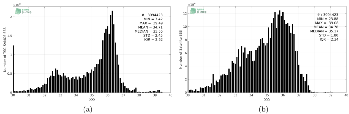
Figure 2: Histograms of SSS from TSG-SAMOS (a) and SMOS-L3-CATDS-IFREMER-CECOS-V2-MONTHLY-0.25DEG (b) considering all match-up pairs per bins of 0.1 over the North Atlantic Ocean Pi-MEP region and for the full satellite product period.
