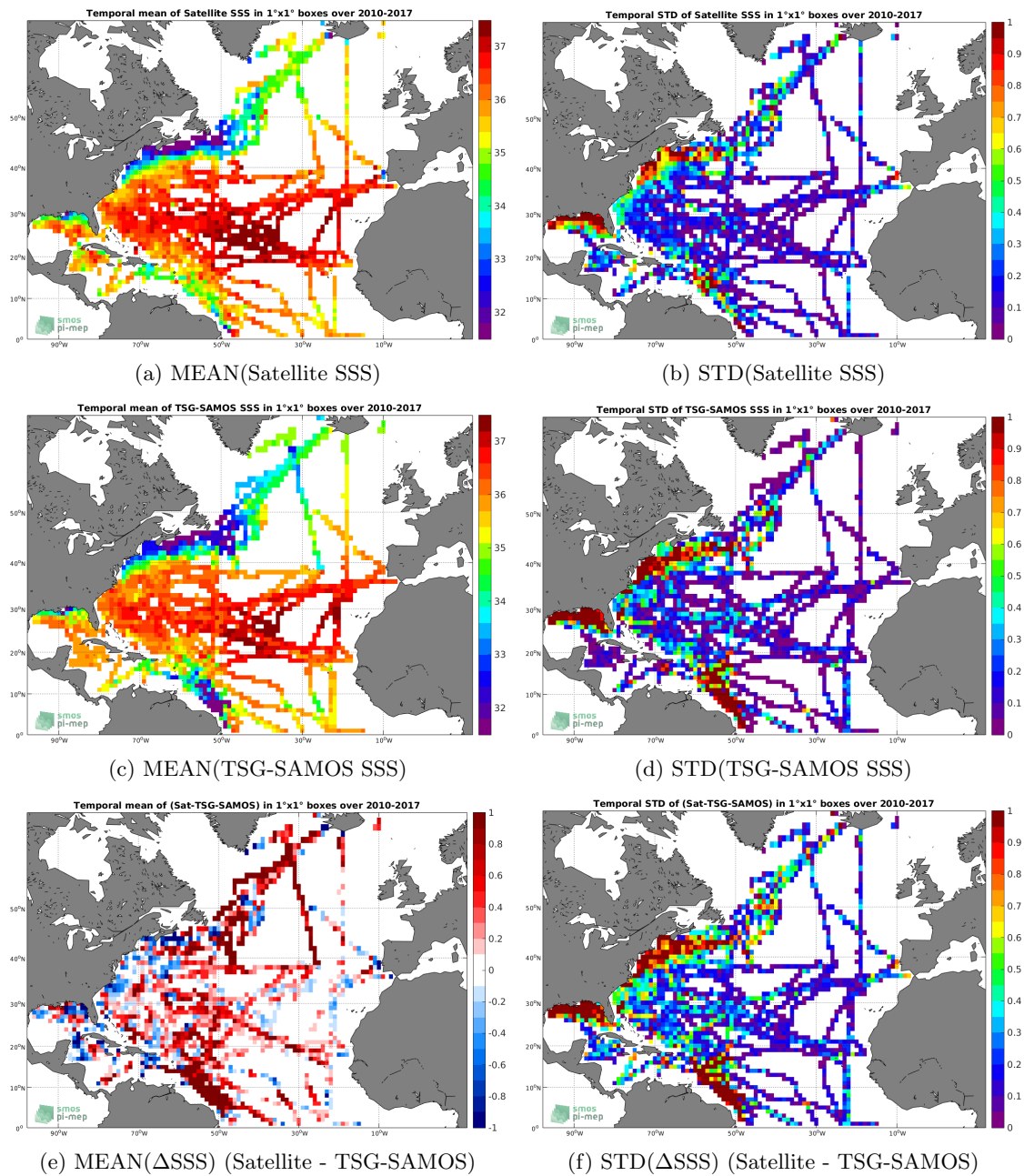
Figure 6: Temporal mean (left) and STD (right) of SSS from SMOS-L3-CATDS-IFREMER-CECOS-V2-MONTHLY-0.25DEG (top), TSG-SAMOS (middle), and of \Delta SSS (Satellite - TSG-SAMOS). Only match-up pairs are used to generate these maps.
