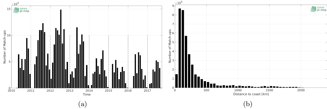
Figure 1: Number of match-ups between TSG-SAMOS and SMOS-L3-CATDS-IFREMER-CECOS-V2-MONTHLY-0.25DEG SSS as a function of time (a) and as function of the distance to coast (b) over the North Atlantic Ocean Pi-MEP region and for the full satellite product period.
