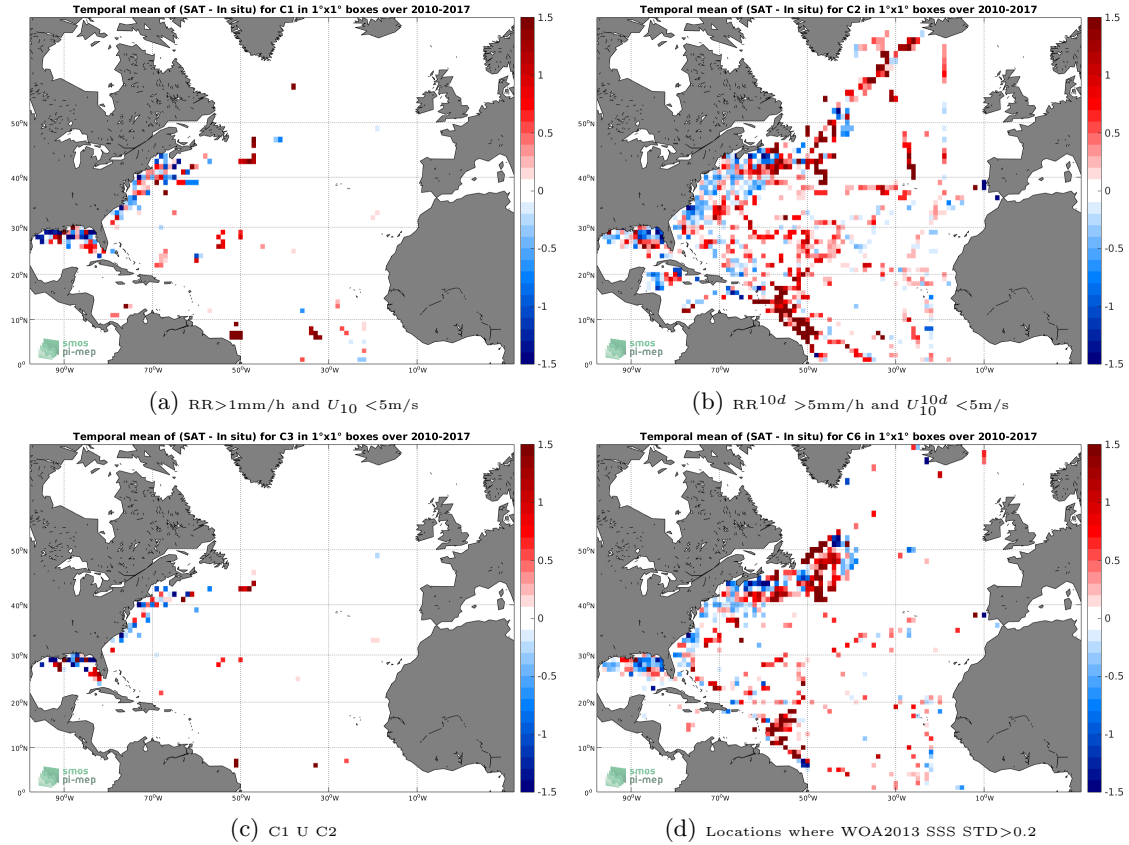
Figure 12: Temporal mean gridded over spatial boxes of size 1^\circ \times 1^\circ of \Delta SSS (SMOS-L3-CATDS-IFREMER-CECOS-V2-MONTHLY-0.25DEG - TSG-SAMOS) for 4 different subdatasets corresponding to: RR > 1\text{mm/h} and U_{10} < 5\text{m/s} (a), RR^{10d} > 5\text{mm/h} and U_{10}^{10d} < 5\text{m/s} (b), C1 U C2 (c), Locations where WOA2013 SSS STD > 0.2 (d).
