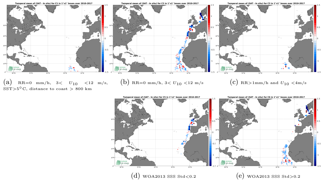
Figure 12: Temporal mean gridded over spatial boxes of size 1^\circ \times 1^\circ of \Delta SSS (SMOS SSS L3 v2 - Monthly - 0.25 Deg (CATDS-CECOS-IFREMER) - TSG (Polarstern)) for 5 different subdatasets corresponding to:RR=0 mm/h, 3 < U_{10} < 12 m/s, SST >5^\circ\text{C} , distance to coast > 800 km (a), RR=0 mm/h, 3 < U_{10} < 12 m/s (b), RR >1 mm/h and U_{10} < 4 m/s (c), WOA2013 SSS Std <0.2 (d), WOA2013 SSS Std >0.2 (e).
