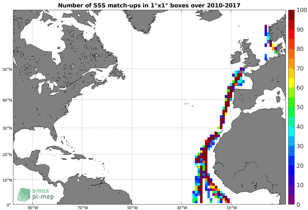
Figure 4: Number of SSS match-ups between TSG (Polarstern) SSS and the SMOS SSS L3 v2 - Monthly - 0.25 Deg (CATDS-CECOS-IFREMER) SSS product for the North Atlantic Ocean Pi-MEP region over 1^\circ \times 1^\circ boxes and for the full satellite product period.
