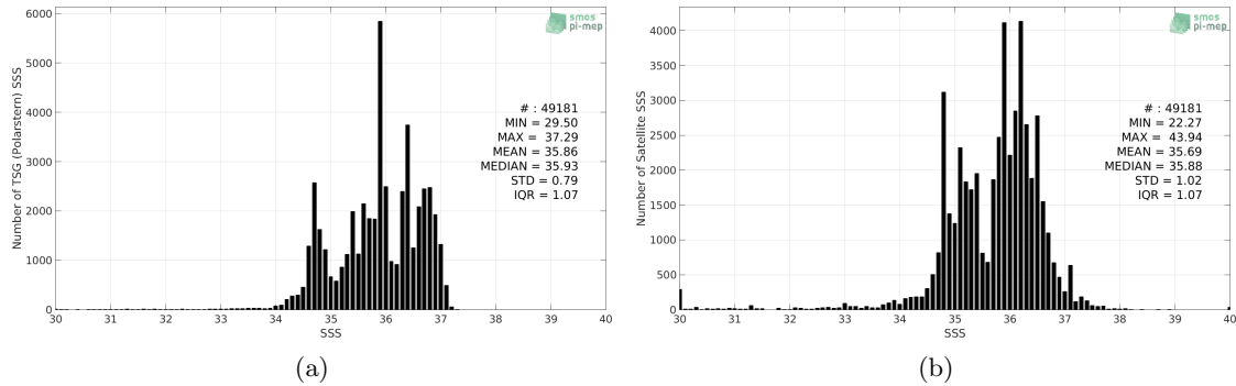
Figure 2: Histograms of SSS from TSG (Polarstern) (a) and SMOS SSS L3 v2 - Monthly - 0.25 Deg (CATDS-CECOS-IFREMER) (b) considering all match-up pairs per bins of 0.1 over the North Atlantic Ocean Pi-MEP region and for the full satellite product period.
