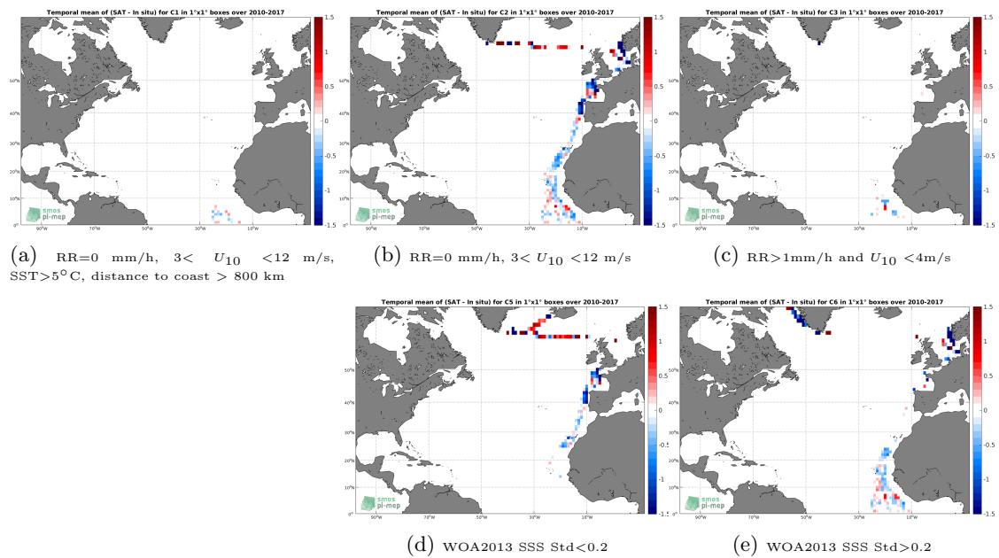
Figure 12: Temporal mean gridded over spatial boxes of size 1^\circ \times 1^\circ of \Delta\text{SSS} (SMOS SSS L3 v2 - Monthly - 0.25 Deg (CATDS-CECOS-IFREMER) - TSG (Polarstern)) for 5 different subdatasets corresponding to:RR=0 mm/h, 3 < U_{10} < 12 m/s, SST >5^\circ\text{C} , distance to coast > 800 km (a), RR=0 mm/h, 3 < U_{10} < 12 m/s (b), RR >1 mm/h and U_{10} < 4 m/s (c), WOA2013 SSS Std <0.2 (d), WOA2013 SSS Std >0.2 (e).
