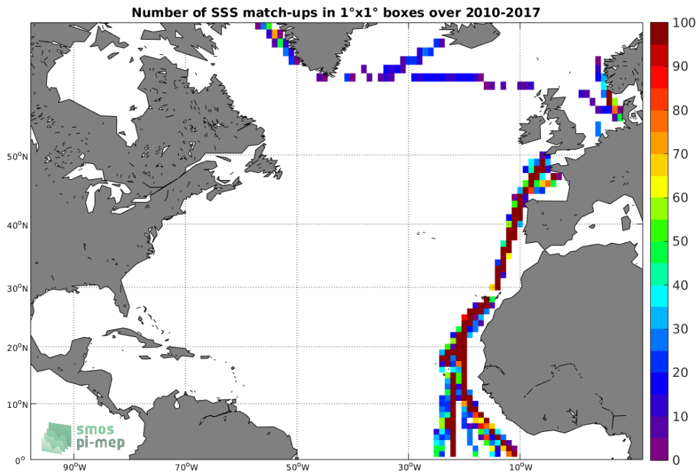
Figure 4: Number of SSS match-ups between TSG (Polarstern) SSS and the SMOS SSS L3 v2 - Monthly - 0.25 Deg (CATDS-CECOS-IFREMER) SSS product for the North Atlantic Ocean Pi-MEP region over 1°x1° boxes and for the full satellite product period.
