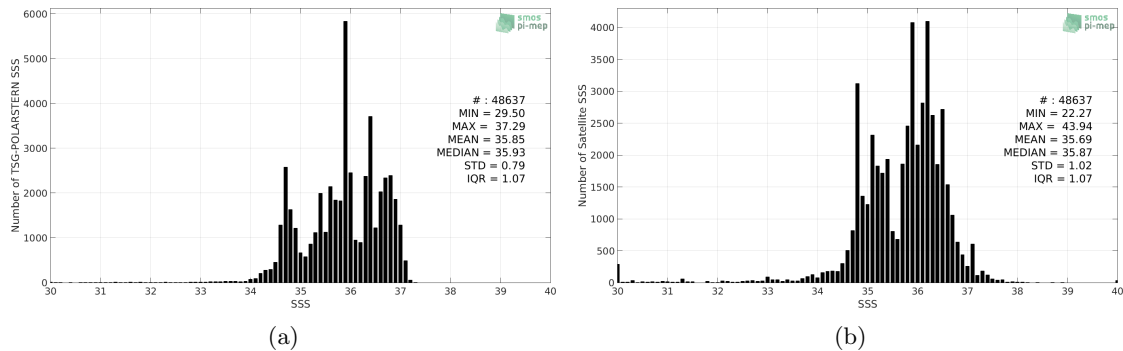
Figure 2: Histograms of SSS from TSG-POLARSTERN (a) and SMOS L3 v2 - Monthly - 0.25 Deg (CATDS-CECOS-IFREMER) (b) considering all match-up pairs per bins of 0.1 over the North Atlantic Ocean Pi-MEP region and for the full satellite product period.
