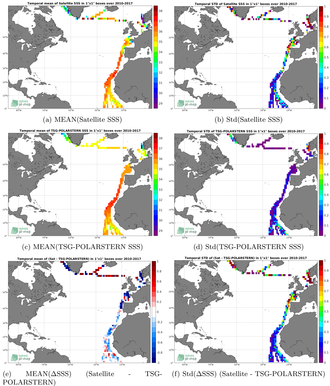
Figure 6: Temporal mean (left) and Std (right) of SSS from SMOS L3 v2 - Monthly - 0.25 Deg (CATDS-CECOS-IFREMER) (top), TSG-POLARSTERN (middle), and of ΔSSS (Satellite - TSG-POLARSTERN). Only match-up pairs are used to generate these maps.
