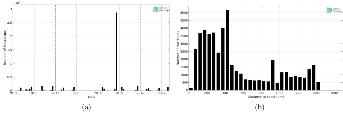
Figure 1: Number of match-ups between TSG-POLARSTERN and SMOS L3 v2 - Monthly - 0.25 Deg (CATDS-CECOS-IFREMER) SSS as a function of time (a) and as function of the distance to coast (b) over the North Atlantic Ocean Pi-MEP region and for the full satellite product period.
