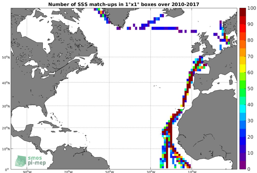
Figure 4: Number of SSS match-ups between TSG-POLARSTERN SSS and the SMOS L3 v2 - Monthly - 0.25 Deg (CATDS-CECOS-IFREMER) SSS product for the North Atlantic Ocean Pi-MEP region over 1°x1° boxes and for the full satellite product period.
