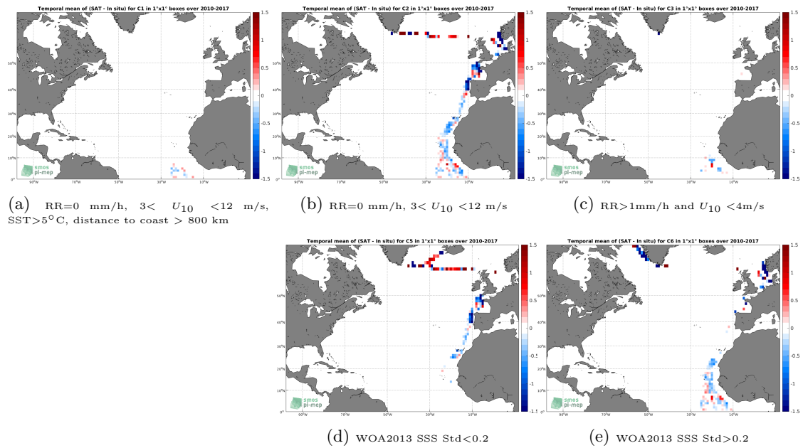
Figure 12: Temporal mean gridded over spatial boxes of size 1^\circ \times 1^\circ of \Delta SSS (SMOS L3 v2 - Monthly - 0.25 Deg (CATDS-CECOS-IFREMER) - TSG-POLARSTERN) for 5 different sub-datasets corresponding to:RR=0 mm/h, 3 < U_{10} < 12 m/s, SST >5^\circ\text{C} , distance to coast > 800 km (a), RR=0 mm/h, 3 < U_{10} < 12 m/s (b), RR >1 mm/h and U_{10} < 4 m/s (c), WOA2013 SSS Std <0.2 (d), WOA2013 SSS Std >0.2 (e).
