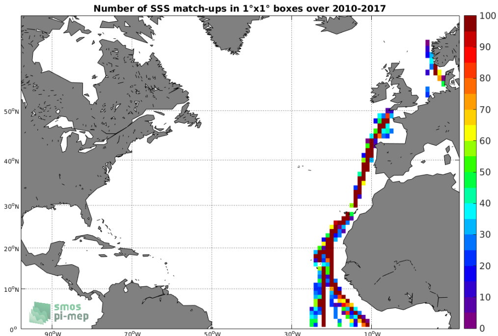
Figure 4: Number of SSS match-ups between TSG-POLARSTERN SSS and the SMOS-L3-CATDS-IFREMER-CECOS-V2-MONTHLY-0.25DEG SSS product for the North Atlantic Ocean Pi-MEP region over 1°x1° boxes and for the full satellite product period.
