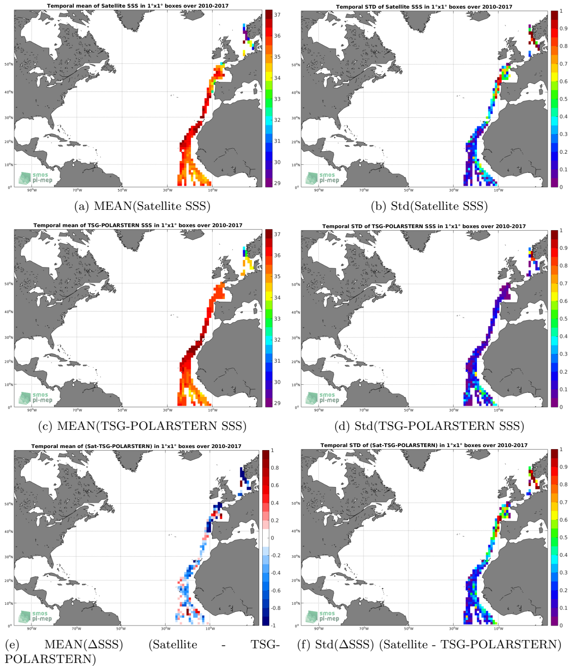
Figure 6: Temporal mean (left) and Std (right) of SSS from SMOS-L3-CATDS-IFREMER-CECOS-V2-MONTHLY-0.25DEG (top), TSG-POLARSTERN (middle), and of \Delta SSS (Satellite - TSG-POLARSTERN). Only match-up pairs are used to generate these maps.
