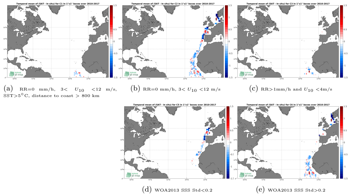
Figure 12: Temporal mean gridded over spatial boxes of size 1^\circ \times 1^\circ of \Delta SSS (SMOS-L3-CATDS-IFREMER-CECOS-V2-MONTHLY-0.25DEG - TSG-POLARSTERN) for 5 different subdatasets corresponding to:RR=0 mm/h, 3 < U_{10} < 12 m/s, SST > 5^\circ\text{C} , distance to coast > 800 km (a), RR=0 mm/h, 3 < U_{10} < 12 m/s (b), RR > 1 mm/h and U_{10} < 4 m/s (c), WOA2013 SSS Std < 0.2 (d), WOA2013 SSS Std > 0.2 (e).
