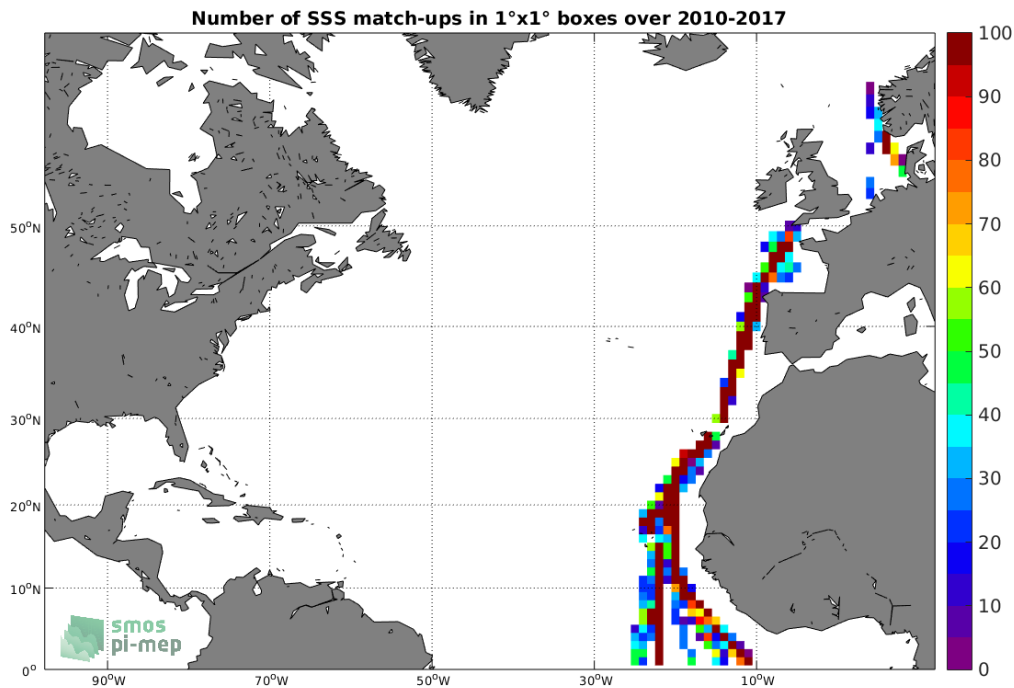
Figure 4: Number of SSS match-ups between TSG-POLARSTERN SSS and the SMOS-L3-CATDS-IFREMER-CECOS-V2-MONTHLY-0.25DEG SSS product for the North Atlantic Ocean Pi-MEP region over 1^\circ \times 1^\circ boxes and for the full satellite product period.
