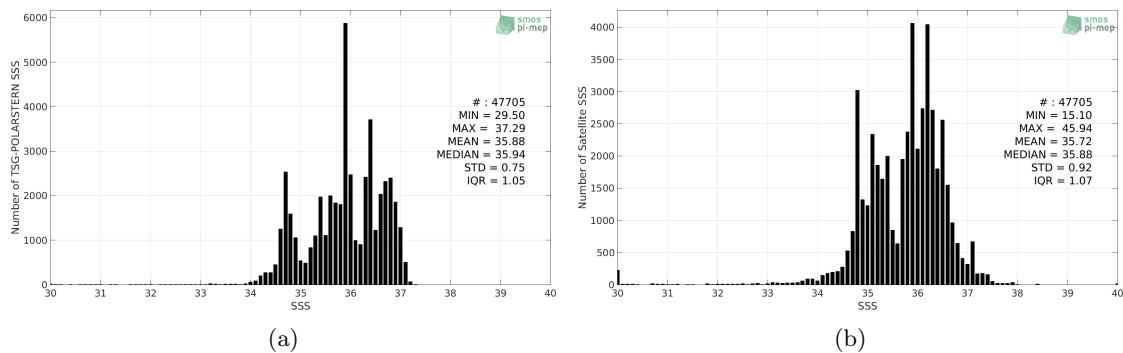
Figure 2: Histograms of SSS from TSG-POLARSTERN (a) and SMOS-L3-CATDS-IFREMER-CECOS-V2-MONTHLY-0.25DEG (b) considering all match-up pairs per bins of 0.1 over the North Atlantic Ocean Pi-MEP region and for the full satellite product period.
