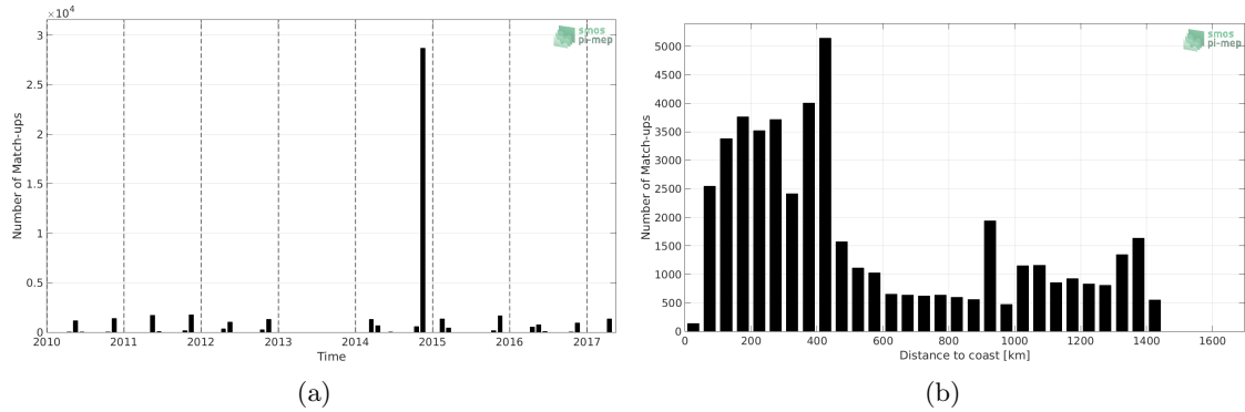
Figure 1: Number of match-ups between TSG-POLARSTERN and SMOS-L3-CATDS-IFREMER-CECOS-V2-MONTHLY-0.25DEG SSS as a function of time (a) and as function of the distance to coast (b) over the North Atlantic Ocean Pi-MEP region and for the full satellite product period.
