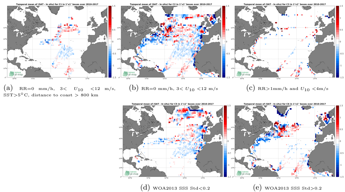
Figure 12: Temporal mean gridded over spatial boxes of size 1^\circ \times 1^\circ of \Delta\text{SSS} (SMOS SSS L3 v2 - Monthly - 0.25 Deg (CATDS-CECOS-IFREMER) - TSG (LEGOS-DM)) for 5 different subdatasets corresponding to:RR=0 mm/h, 3 < U_{10} < 12 m/s, SST > 5^\circ\text{C} , distance to coast > 800 km (a), RR=0 mm/h, 3 < U_{10} < 12 m/s (b), RR > 1 mm/h and U_{10} < 4 m/s (c), WOA2013 SSS Std < 0.2 (d), WOA2013 SSS Std > 0.2 (e).
