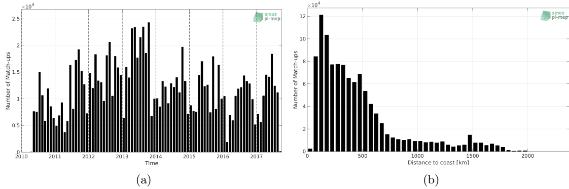
Figure 1: Number of match-ups between TSG-LEGOS-DM and SMOS L3 v2 - Monthly - 0.25 Deg (CATDS-CECOS-IFREMER) SSS as a function of time (a) and as function of the distance to coast (b) over the North Atlantic Ocean Pi-MEP region and for the full satellite product period.
