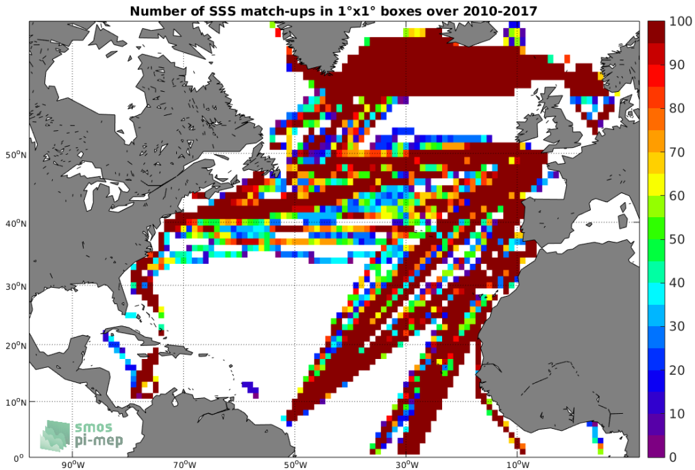
Figure 4: Number of SSS match-ups between TSG-LEGOS-DM SSS and the SMOS L3 v2 - Monthly - 0.25 Deg (CATDS-CECOS-IFREMER) SSS product for the North Atlantic Ocean Pi-MEP region over 1^\circ \times 1^\circ boxes and for the full satellite product period.
