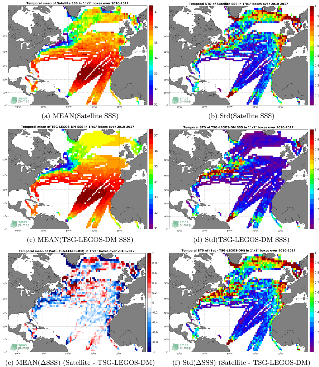
Figure 6: Temporal mean (left) and Std (right) of SSS from SMOS L3 v2 - Monthly - 0.25 Deg (CATDS-CECOS-IFREMER) (top), TSG-LEGOS-DM (middle), and of \Delta SSS (Satellite - TSG-LEGOS-DM). Only match-up pairs are used to generate these maps.
