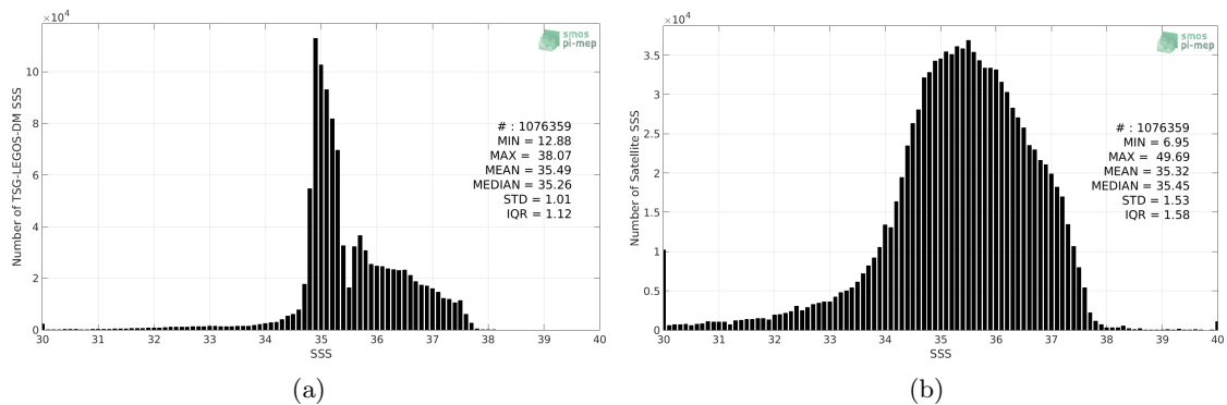
Figure 2: Histograms of SSS from TSG-LEGOS-DM (a) and SMOS L3 v2 - Monthly - 0.25 Deg (CATDS-CECOS-IFREMER) (b) considering all match-up pairs per bins of 0.1 over the North Atlantic Ocean Pi-MEP region and for the full satellite product period.
