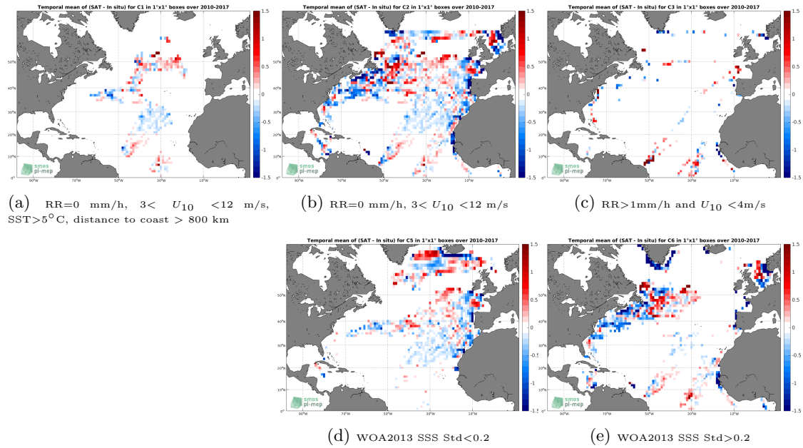
Figure 12: Temporal mean gridded over spatial boxes of size 1^\circ \times 1^\circ of \Delta SSS (SMOS-L3-CATDS-IFREMER-CECOS-V2-MONTHLY-0.25DEG - TSG-LEGOS-DM) for 5 different subdatasets corresponding to:RR=0 mm/h, 3 < U_{10} < 12 m/s, SST >5^\circ\text{C} , distance to coast > 800 km (a), RR=0 mm/h, 3 < U_{10} < 12 m/s (b), RR >1 mm/h and U_{10} < 4 m/s (c), WOA2013 SSS Std <0.2 (d), WOA2013 SSS Std >0.2 (e).
