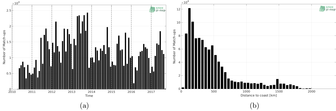
Figure 1: Number of match-ups between TSG-LEGOS-DM and SMOS-L3-CATDS-IFREMER-CECOS-V2-MONTHLY-0.25DEG SSS as a function of time (a) and as function of the distance to coast (b) over the North Atlantic Ocean Pi-MEP region and for the full satellite product period.
