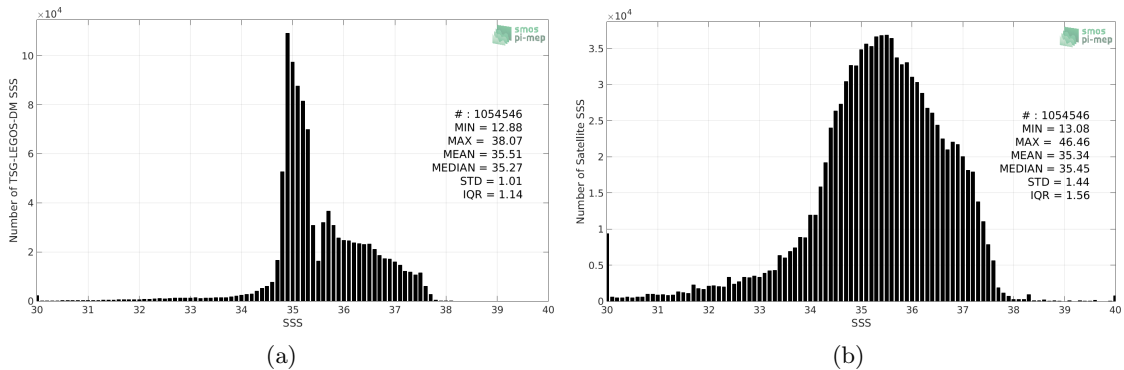
Figure 2: Histograms of SSS from TSG-LEGOS-DM (a) and SMOS-L3-CATDS-IFREMER-CECOS-V2-MONTHLY-0.25DEG (b) considering all match-up pairs per bins of 0.1 over the North Atlantic Ocean Pi-MEP region and for the full satellite product period.
