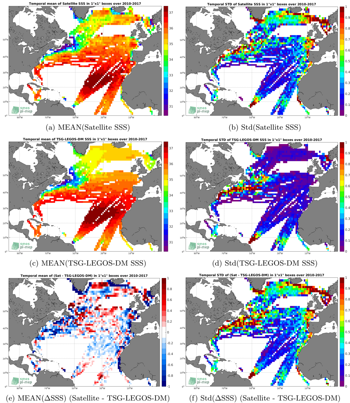
Figure 6: Temporal mean (left) and Std (right) of SSS from SMOS-L3-CATDS-IFREMER-CECOS-V2-MONTHLY-0.25DEG (top), TSG-LEGOS-DM (middle), and of \Delta SSS (Satellite - TSG-LEGOS-DM). Only match-up pairs are used to generate these maps.
