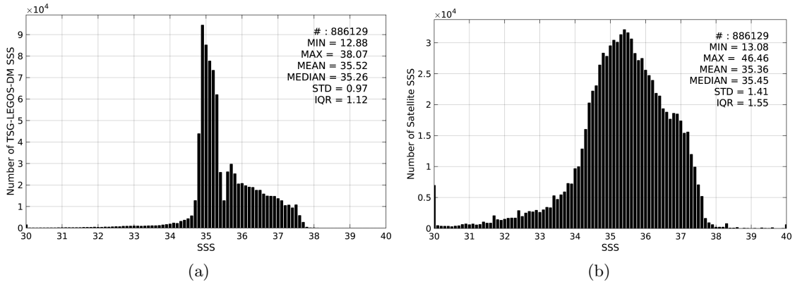
Figure 2: Histograms of SSS from TSG-LEGOS-DM (a) and SMOS-L3-CATDS-IFREMER-CECOS-V2-MONTHLY-0.25DEG (b) considering all match-up pairs per bins of 0.1 over the North Atlantic Ocean Pi-MEP region and for the full satellite product period.
