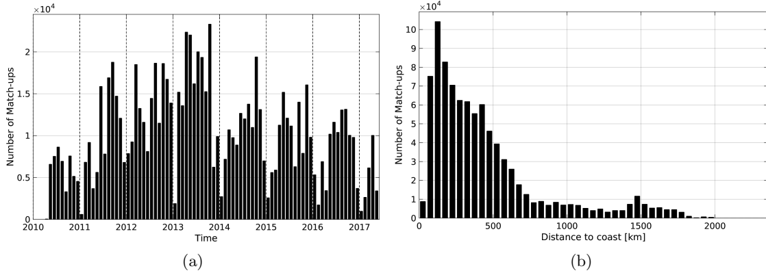
Figure 1: Number of match-ups between TSG-LEGOS-DM and SMOS-L3-CATDS-IFREMER-CECOS-V2-MONTHLY-0.25DEG SSS as a function of time (a) and as function of the distance to coast (b) over the North Atlantic Ocean Pi-MEP region and for the full satellite product period.
