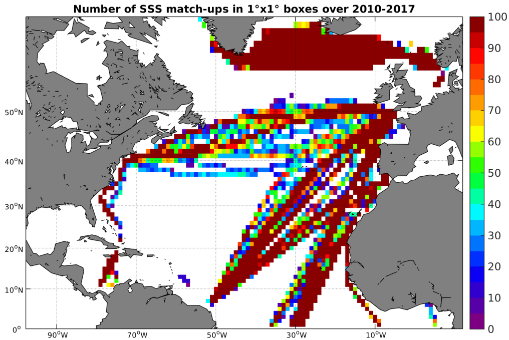
Figure 4: Number of SSS match-ups between TSG-LEGOS-DM SSS and the SMOS-L3-CATDS-IFREMER-CECOS-V2-MONTHLY-0.25DEG SSS product for the North Atlantic Ocean Pi-MEP region over 1^\circ \times 1^\circ boxes and for the full satellite product period.
