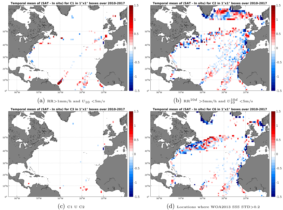
Figure 12: Temporal mean gridded over spatial boxes of size 1°x1° of \Delta SSS (SMOS-L3-CATDS-IFREMER-CECOS-V2-MONTHLY-0.25DEG - TSG-LEGOS-DM) for 4 different subdatasets corresponding to:RR>1mm/h and U_{10} < 5m/s (a), RR^{10d} > 5mm/h and U_{10}^{10d} < 5m/s (b), C1 U C2 (c),Locations where WOA2013 SSS STD>0.2 (d).
