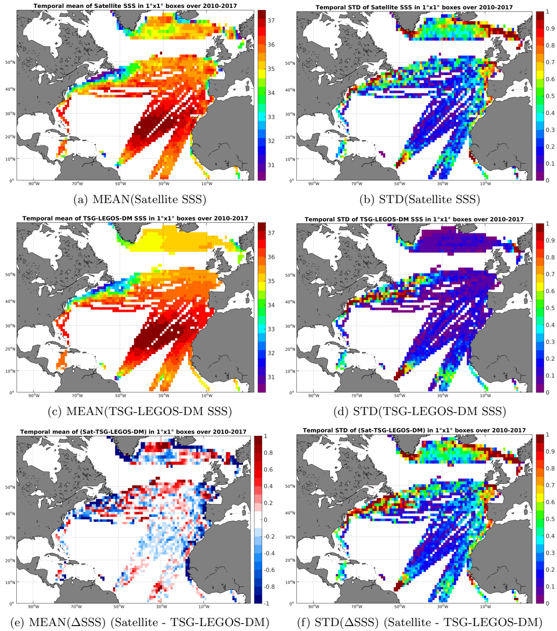
Figure 6: Temporal mean (left) and STD (right) of SSS from SMOS-L3-CATDS-IFREMER-CECOS-V2-MONTHLY-0.25DEG (top), TSG-LEGOS-DM (middle), and of \Delta SSS (Satellite - TSG-LEGOS-DM). Only match-up pairs are used to generate these maps.
