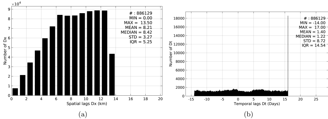
Figure 5: Histograms of the spatial (a) and temporal (b) lags between the time of the TSG-LEGOS-DM measurements and the date of the corresponding SMOS-L3-CATDS-IFREMER-CECOS-V2-MONTHLY-0.25DEG SSS product.
