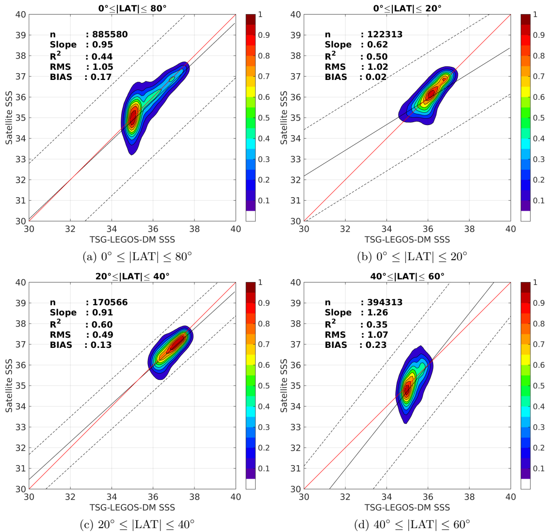
Figure 9: Contour maps of the concentration of SMOS-L3-CATDS-IFREMER-CECOS-V2-MONTHLY-0.25DEG SSS (y-axis) versus TSG-LEGOS-DM SSS (x-axis) at match-up pairs for different latitude bands. For each plot, the red line shows x=y . The black thin and dashed lines indicate a linear fit through the data cloud and the \pm 95\% confidence levels, respectively. The number match-up pairs n , the slope and R^2 coefficient of the linear fit, the root mean square (RMS) and the mean bias between satellite and in situ data are indicated for each latitude band in each plots.
