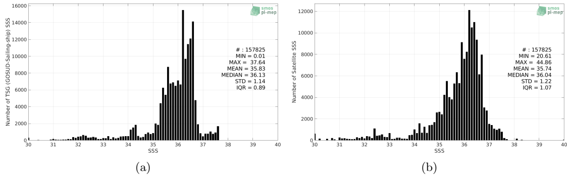
Figure 2: Histograms of SSS from TSG (GOSUD-Sailing-ship) (a) and SMOS SSS L3 v2 - Monthly - 0.25 Deg (CATDS-CECOS-IFREMER) (b) considering all match-up pairs per bins of 0.1 over the North Atlantic Ocean Pi-MEP region and for the full satellite product period.
