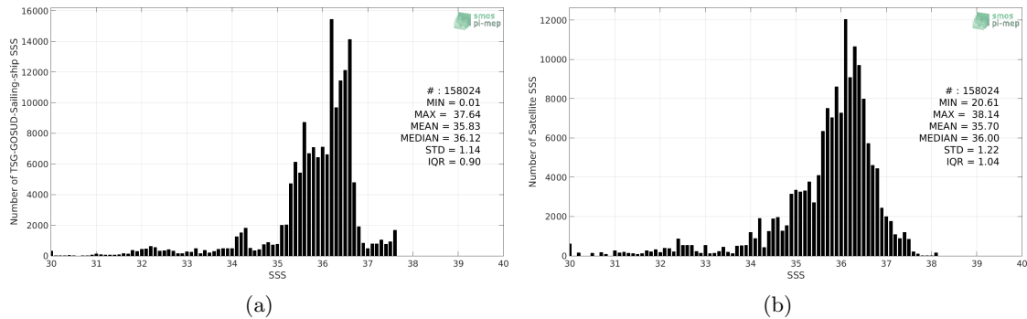
Figure 2: Histograms of SSS from TSG-GOSUD-Sailing-ship (a) and SMOS L3 v2 - Monthly - 0.25 Deg (CATDS-CECOS-IFREMER) (b) considering all match-up pairs per bins of 0.1 over the North Atlantic Ocean Pi-MEP region and for the full satellite product period.
