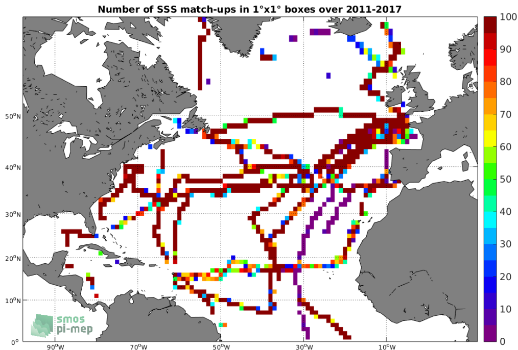
Figure 4: Number of SSS match-ups between TSG-GOSUD-Sailing-ship SSS and the SMOS L3 v2 - Monthly - 0.25 Deg (CATDS-CECOS-IFREMER) SSS product for the North Atlantic Ocean Pi-MEP region over 1^\circ \times 1^\circ boxes and for the full satellite product period.
