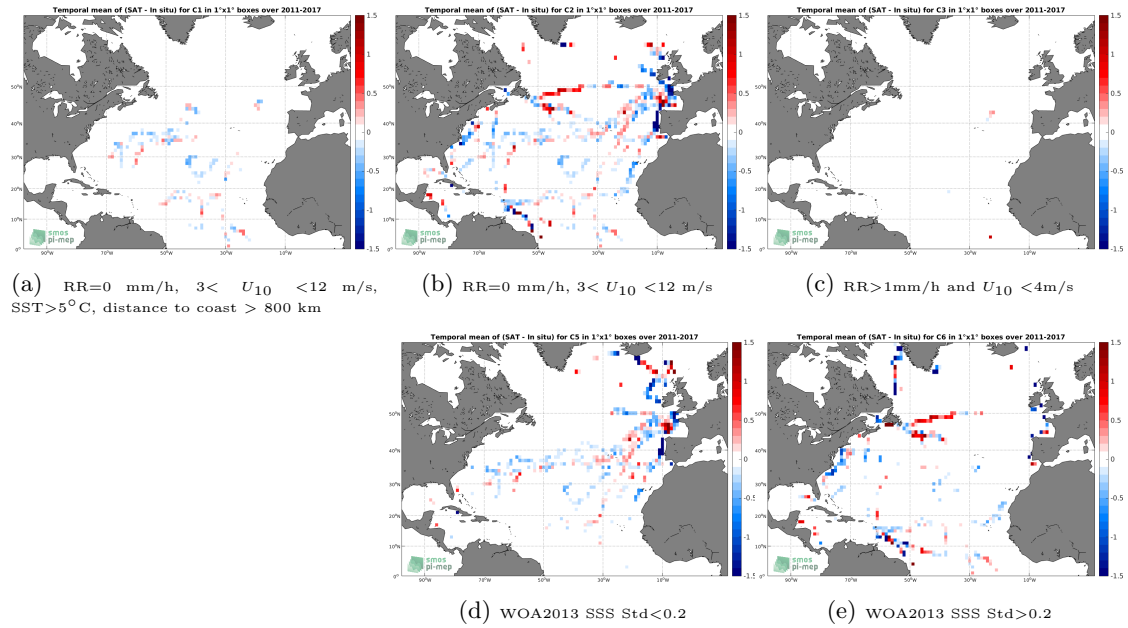
Figure 12: Temporal mean gridded over spatial boxes of size 1^\circ \times 1^\circ of \Delta SSS (SMOS-L3-CATDS-IFREMER-CECOS-V2-MONTHLY-0.25DEG - TSG-GOSUD-Sailing-ship) for 5 different sub-datasets corresponding to:RR=0 mm/h, 3 < U_{10} < 12 m/s, SST >5^\circ\text{C} , distance to coast > 800 km (a), RR=0 mm/h, 3 < U_{10} < 12 m/s (b), RR >1 mm/h and U_{10} < 4 m/s (c), WOA2013 SSS Std <0.2 (d), WOA2013 SSS Std >0.2 (e).
