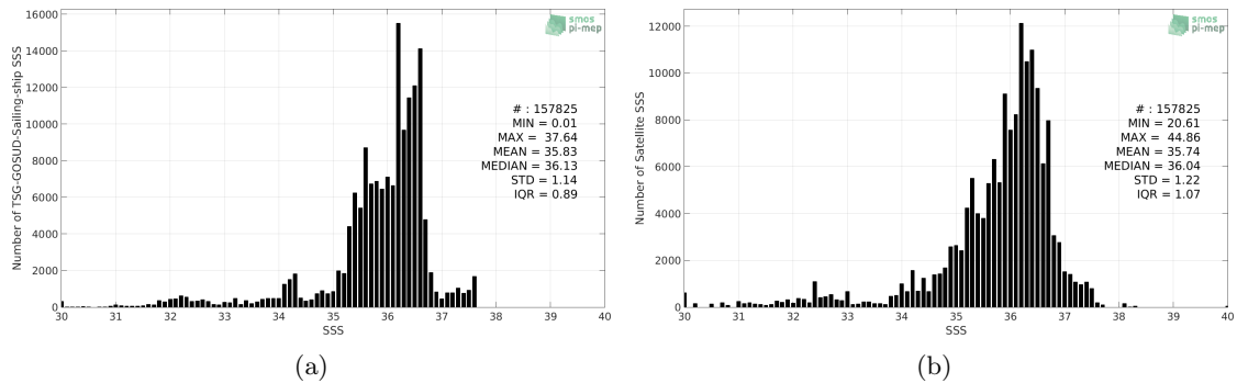
Figure 2: Histograms of SSS from TSG-GOSUD-Sailing-ship (a) and SMOS-L3-CATDS-IFREMER-CECOS-V2-MONTHLY-0.25DEG (b) considering all match-up pairs per bins of 0.1 over the North Atlantic Ocean Pi-MEP region and for the full satellite product period.
