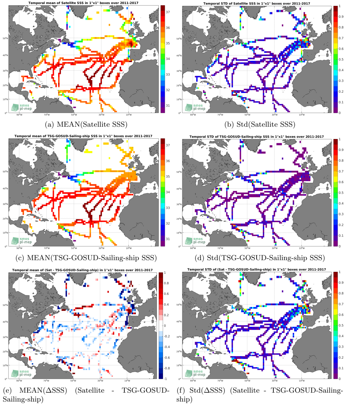
Figure 6: Temporal mean (left) and Std (right) of SSS from SMOS-L3-CATDS-IFREMER-CECOS-V2-MONTHLY-0.25DEG (top), TSG-GOSUD-Sailing-ship (middle), and of \Delta SSS (Satellite - TSG-GOSUD-Sailing-ship). Only match-up pairs are used to generate these maps.
