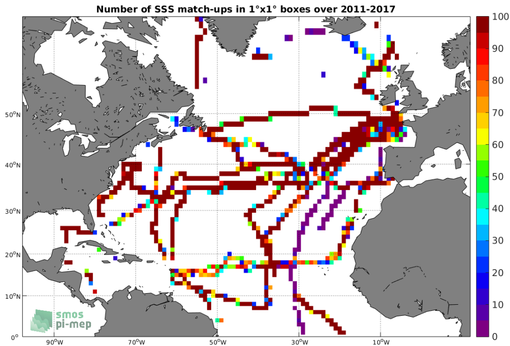
Figure 4: Number of SSS match-ups between TSG-GOSUD-Sailing-ship SSS and the SMOS-L3-CATDS-IFREMER-CECOS-V2-MONTHLY-0.25DEG SSS product for the North Atlantic Ocean Pi-MEP region over 1^\circ \times 1^\circ boxes and for the full satellite product period.
