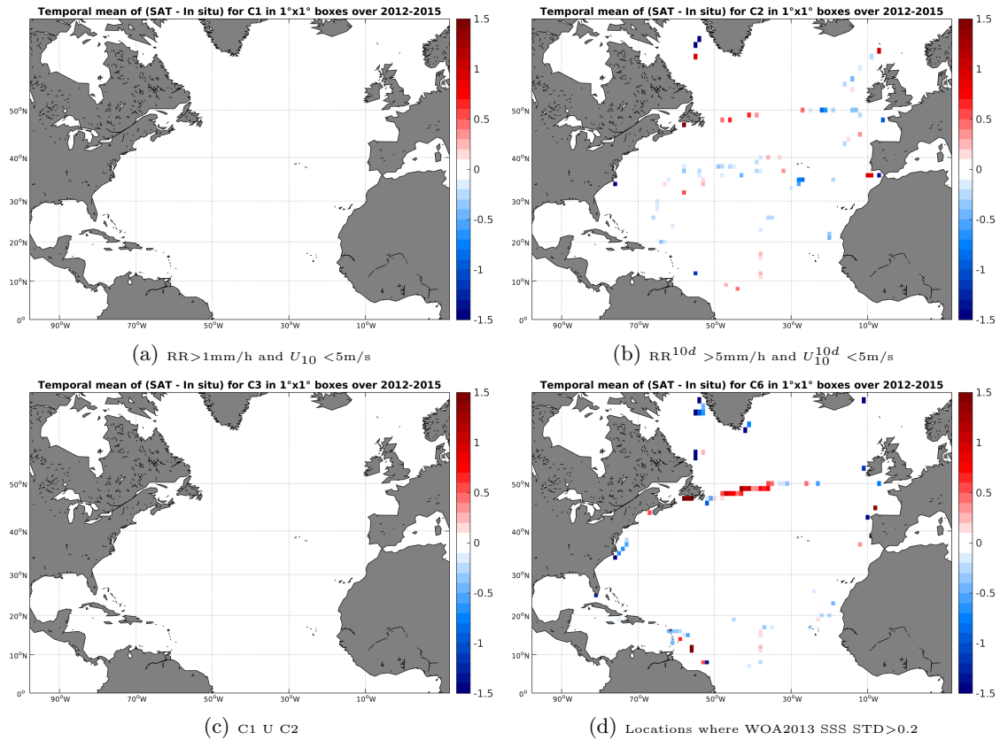
Figure 12: Temporal mean gridded over spatial boxes of size 1°x1° of \Delta SSS (SMOS-L3-CATDS-IFREMER-CECOS-V2-MONTHLY-0.25DEG - TSG-GOSUD-Sailing-ship) for 4 different sub-datasets corresponding to:RR>1mm/h and U_{10} < 5\text{m/s} (a), RR^{10d} > 5\text{mm/h} and U_{10}^{10d} < 5\text{m/s} (b), C1 U C2 (c),Locations where WOA2013 SSS STD>0.2 (d).
