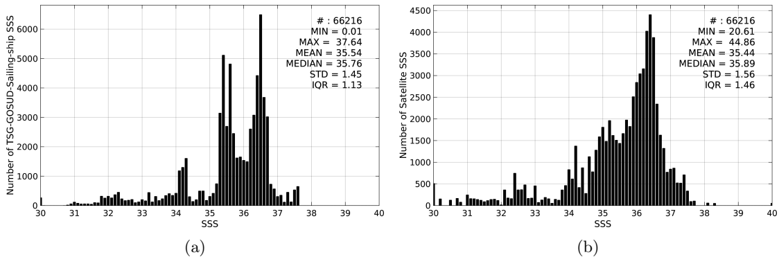
Figure 2: Histograms of SSS from TSG-GOSUD-Sailing-ship (a) and SMOS-L3-CATDS-IFREMER-CECOS-V2-MONTHLY-0.25DEG (b) considering all match-up pairs per bins of 0.1 over the North Atlantic Ocean Pi-MEP region and for the full satellite product period.
