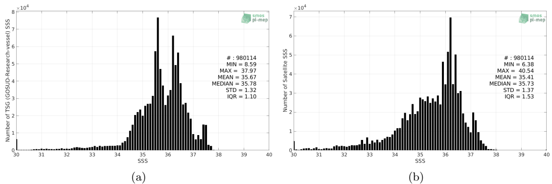
Figure 2: Histograms of SSS from TSG (GOSUD-Research-vessel) (a) and SMOS SSS L3 v2 - Monthly - 0.25 Deg (CATDS-CECOS-IFREMER) (b) considering all match-up pairs per bins of 0.1 over the North Atlantic Ocean Pi-MEP region and for the full satellite product period.
