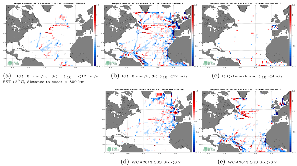
Figure 12: Temporal mean gridded over spatial boxes of size 1^\circ \times 1^\circ of \Delta SSS (SMOS SSS L3 v2 - Monthly - 0.25 Deg (CATDS-CECOS-IFREMER) - TSG (GOSUD-Research-vessel)) for 5 different subdatasets corresponding to:RR=0 mm/h, 3 < U_{10} < 12 m/s, SST > 5^\circ\text{C} , distance to coast > 800 km (a), RR=0 mm/h, 3 < U_{10} < 12 m/s (b), RR > 1 mm/h and U_{10} < 4 m/s (c), WOA2013 SSS Std < 0.2 (d), WOA2013 SSS Std > 0.2 (e).
