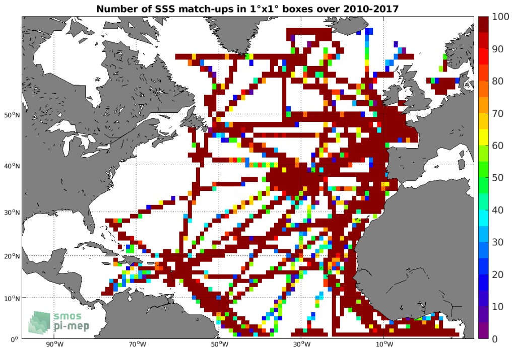
Figure 4: Number of SSS match-ups between TSG (GOSUD-Research-vessel) SSS and the SMOS SSS L3 v2 - Monthly - 0.25 Deg (CATDS-CECOS-IFREMER) SSS product for the North Atlantic Ocean Pi-MEP region over 1^{\circ} \times 1^{\circ} boxes and for the full satellite product period.
