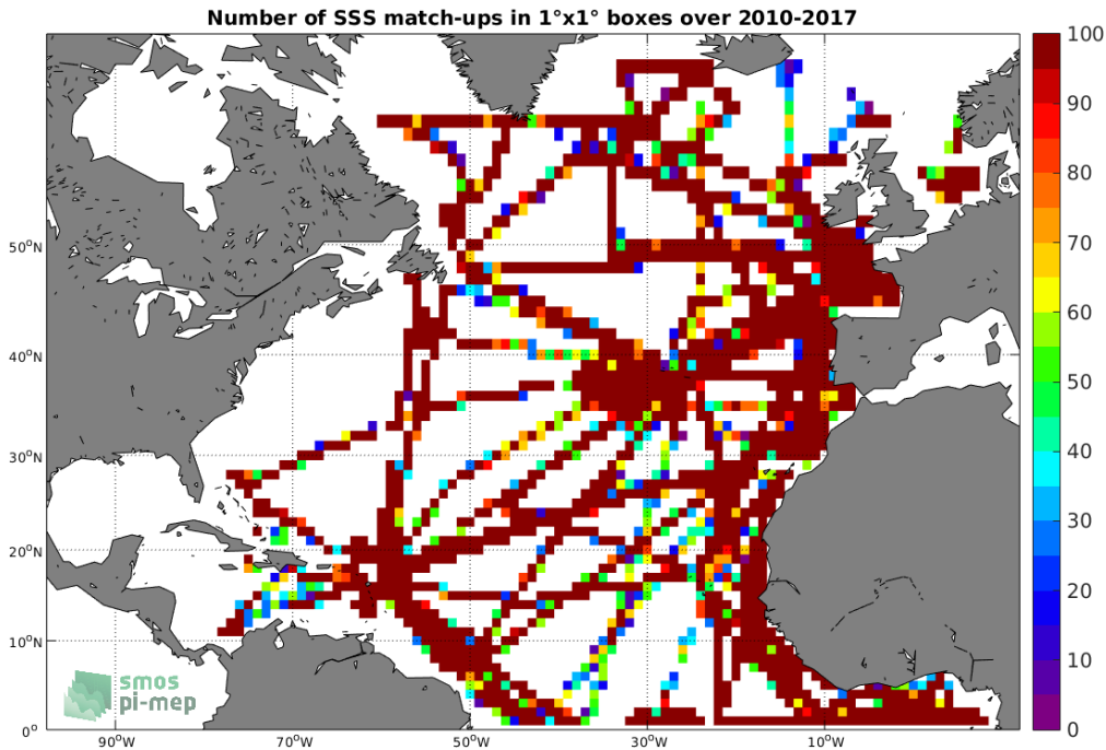
Figure 4: Number of SSS match-ups between TSG-GOSUD-Research-vessel SSS and the SMOS L3 v2 - Monthly - 0.25 Deg (CATDS-CECOS-IFREMER) SSS product for the North Atlantic Ocean Pi-MEP region over 1^\circ \times 1^\circ boxes and for the full satellite product period.
