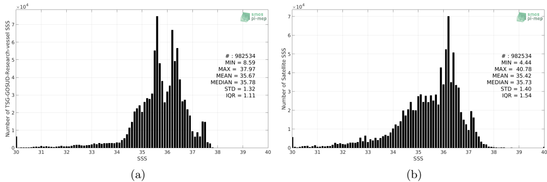
Figure 2: Histograms of SSS from TSG-GOSUD-Research-vessel (a) and SMOS L3 v2 - Monthly - 0.25 Deg (CATDS-CECOS-IFREMER) (b) considering all match-up pairs per bins of 0.1 over the North Atlantic Ocean Pi-MEP region and for the full satellite product period.
