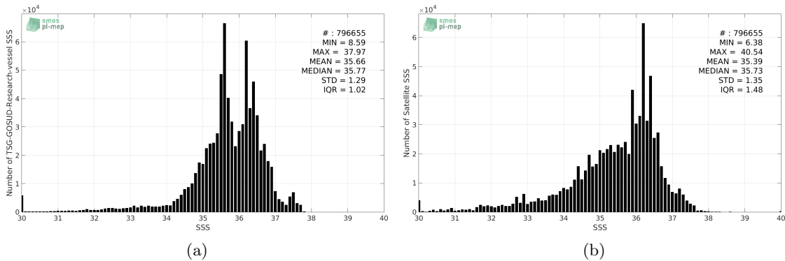
Figure 2: Histograms of SSS from TSG-GOSUD-Research-vessel (a) and SMOS-L3-CATDS-IFREMER-CECOS-V2-MONTHLY-0.25DEG (b) considering all match-up pairs per bins of 0.1 over the North Atlantic Ocean Pi-MEP region and for the full satellite product period.
