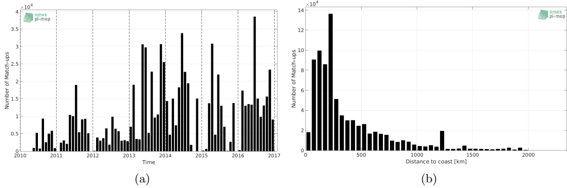
Figure 1: Number of match-ups between TSG-GOSUD-Research-vessel and SMOS-L3-CATDS-IFREMER-CECOS-V2-MONTHLY-0.25DEG SSS as a function of time (a) and as function of the distance to coast (b) over the North Atlantic Ocean Pi-MEP region and for the full satellite product period.
