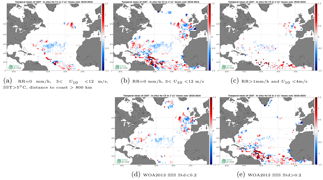
Figure 11: Temporal mean gridded over spatial boxes of size 1^\circ \times 1^\circ of \Delta SSS (SMOS SSS L3 v2 - Monthly - 0.25 Deg (CATDS-CECOS-IFREMER) - Surface drifters) for 5 different subdatasets corresponding to:RR=0 mm/h, 3 < U_{10} < 12 m/s, SST >5^\circ\text{C} , distance to coast > 800 km (a), RR=0 mm/h, 3 < U_{10} < 12 m/s (b), RR >1 mm/h and U_{10} < 4 m/s (c), WOA2013 SSS Std <0.2 (d), WOA2013 SSS Std >0.2 (e).
