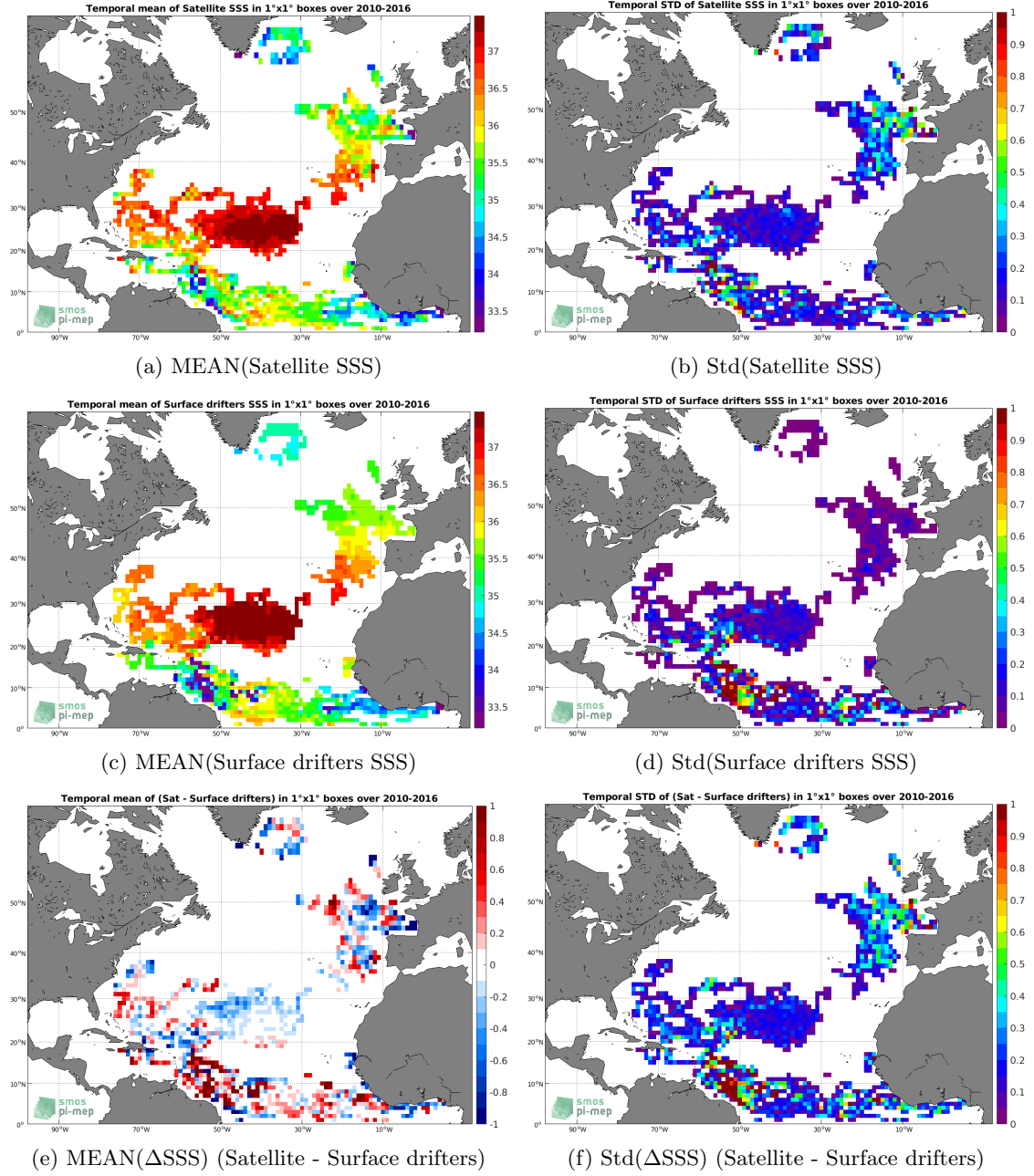
Figure 5: Temporal mean (left) and Std (right) of SSS from SMOS SSS L3 v2 - Monthly - 0.25 Deg (CATDS-CECOS-IFREMER) (top), Surface drifters (middle), and of \Delta SSS (Satellite - Surface drifters). Only match-up pairs are used to generate these maps.
