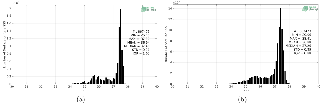
Figure 2: Histograms of SSS from Surface drifters (a) and SMOS SSS L3 v2 - Monthly - 0.25 Deg (CATDS-CECOS-IFREMER) (b) considering all match-up pairs per bins of 0.1 over the North Atlantic Ocean Pi-MEP region and for the full satellite product period.
