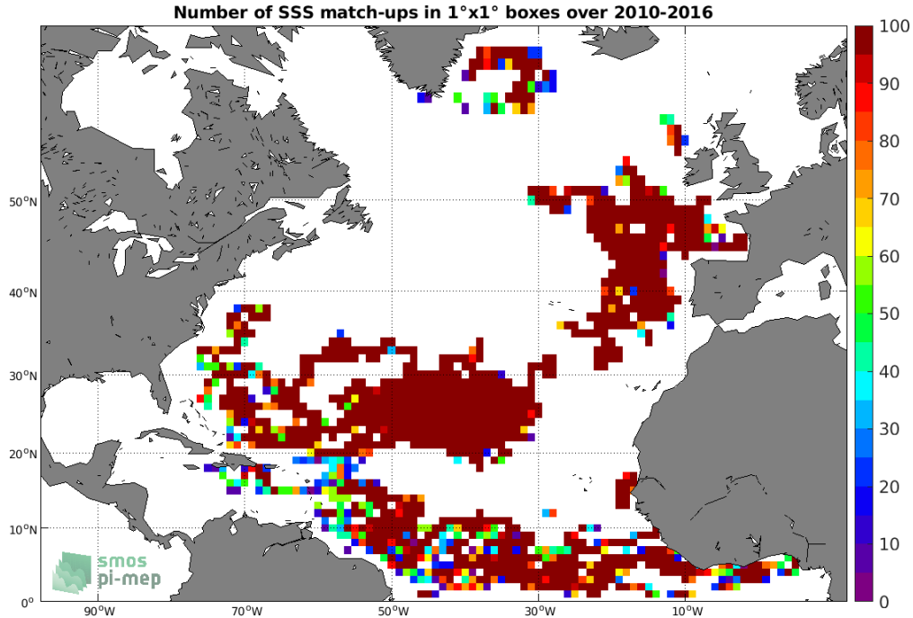
Figure 3: Number of SSS match-ups between Surface drifters SSS and the SMOS SSS L3 v2 - Monthly - 0.25 Deg (CATDS-CECOS-IFREMER) SSS product for the North Atlantic Ocean Pi-MEP region over 1^\circ \times 1^\circ boxes and for the full satellite product period.
