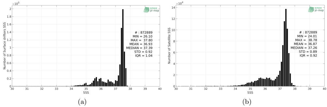
Figure 2: Histograms of SSS from Surface drifters (a) and SMOS L3 v2 - Monthly - 0.25 Deg (CATDS-CECOS-IFREMER) (b) considering all match-up pairs per bins of 0.1 over the North Atlantic Ocean Pi-MEP region and for the full satellite product period.
