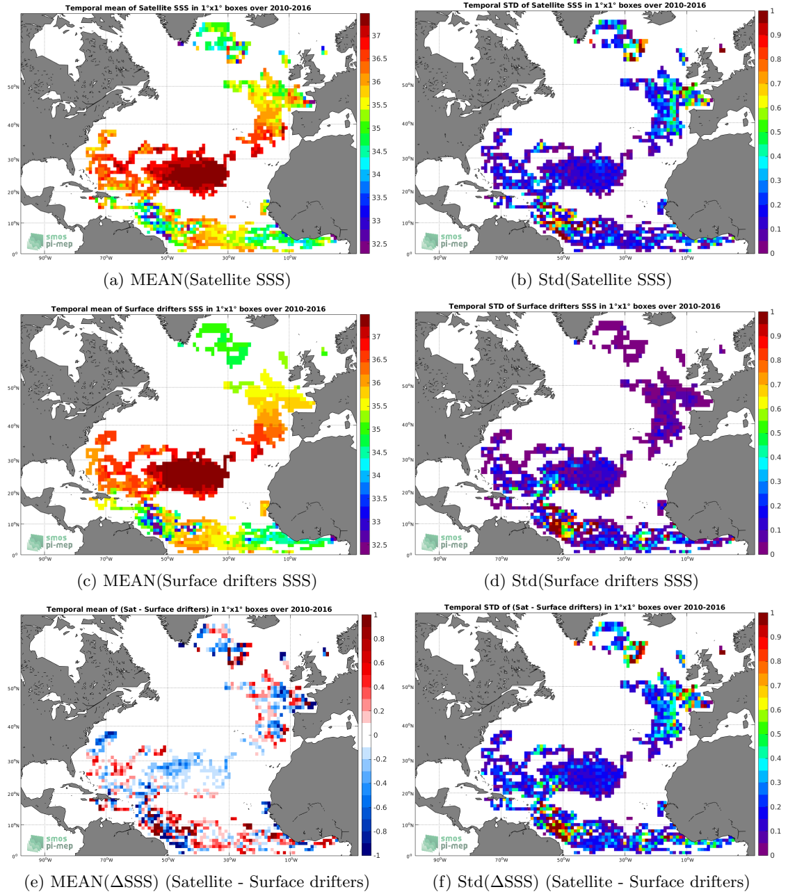
Figure 5: Temporal mean (left) and Std (right) of SSS from SMOS L3 v2 - Monthly - 0.25 Deg (CATDS-CECOS-IFREMER) (top), Surface drifters (middle), and of \Delta SSS (Satellite - Surface drifters). Only match-up pairs are used to generate these maps.
