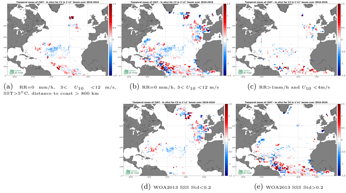
Figure 11: Temporal mean gridded over spatial boxes of size 1^\circ \times 1^\circ of \Delta SSS (SMOS L3 v2 - Monthly - 0.25^\circ Deg (CATDS-CECOS-IFREMER) - Surface drifters) for 5 different subdatasets corresponding to: RR=0 mm/h, 3 < U_{10} < 12 m/s, SST > 5^\circ\text{C} , distance to coast > 800 km (a), RR=0 mm/h, 3 < U_{10} < 12 m/s (b), RR > 1 mm/h and U_{10} < 4 m/s (c), WOA2013 SSS Std < 0.2 (d), WOA2013 SSS Std > 0.2 (e).
