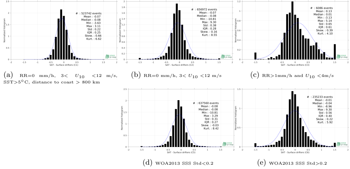
Figure 12: Normalized histogram of \Delta\text{SSS} (SMOS L3 v2 - Monthly - 0.25 Deg (CATDS-CECOS-IFREMER) - Surface drifters) for 5 different subdatasets corresponding to: RR=0 mm/h, 3 < U_{10} < 12 m/s, SST > 5^\circ\text{C} , distance to coast > 800 km (a), RR=0 mm/h, 3 < U_{10} < 12 m/s (b), RR > 1\text{mm/h} and U_{10} < 4\text{m/s} (c), WOA2013 SSS Std < 0.2 (d), WOA2013 SSS Std > 0.2 (e).
