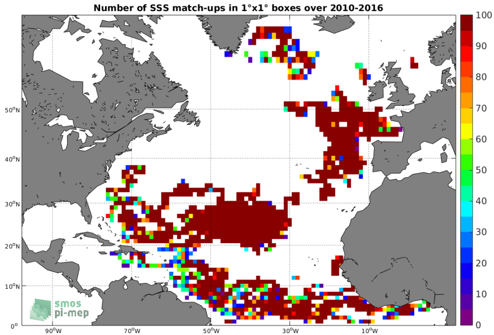
Figure 3: Number of SSS match-ups between Surface drifters SSS and the SMOS L3 v2 - Monthly - 0.25 Deg (CATDS-CECOS-IFREMER) SSS product for the North Atlantic Ocean Pi-MEP region over 1^\circ \times 1^\circ boxes and for the full satellite product period.
