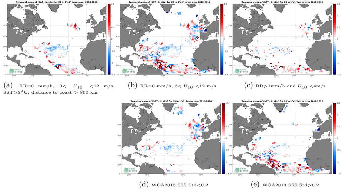
Figure 11: Temporal mean gridded over spatial boxes of size 1^\circ \times 1^\circ of \Delta SSS (SMOS-L3-CATDS-IFREMER-CECOS-V2-MONTHLY-0.25DEG - Surface drifters) for 5 different subdatasets corresponding to: RR=0 mm/h, 3 < U_{10} < 12 m/s, SST >5^\circ C, distance to coast > 800 km (a), RR=0 mm/h, 3 < U_{10} < 12 m/s (b), RR >1 mm/h and U_{10} < 4 m/s (c), WOA2013 SSS Std <0.2 (d), WOA2013 SSS Std >0.2 (e).
