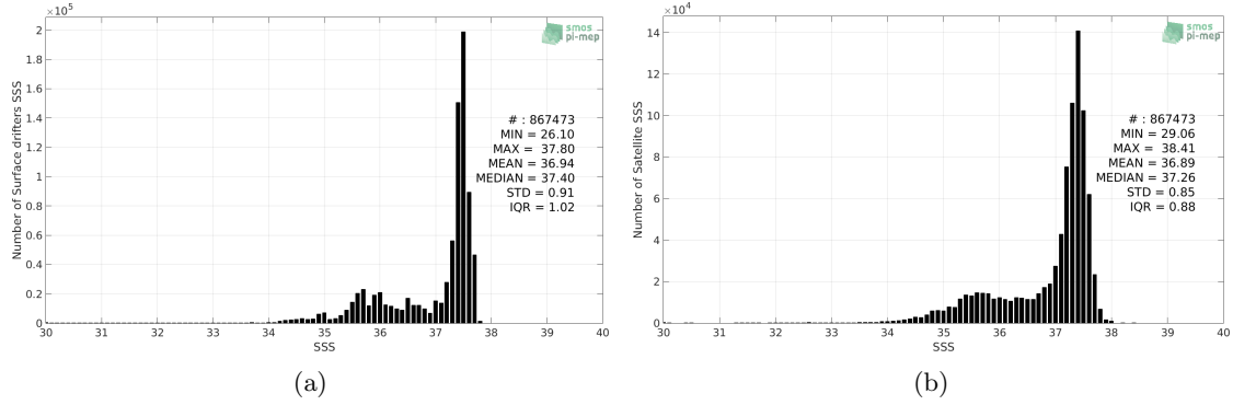
Figure 2: Histograms of SSS from Surface drifters (a) and SMOS-L3-CATDS-IFREMER-CECOS-V2-MONTHLY-0.25DEG (b) considering all match-up pairs per bins of 0.1 over the North Atlantic Ocean Pi-MEP region and for the full satellite product period.
