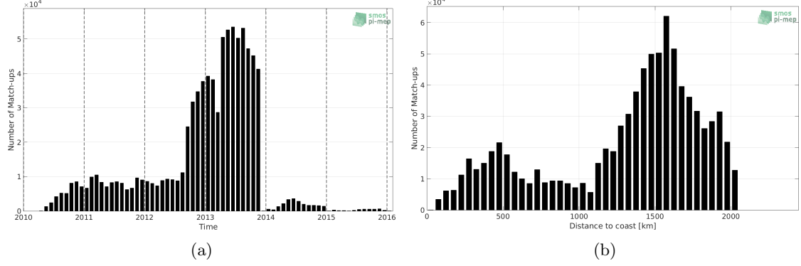
Figure 1: Number of match-ups between Surface drifters and SMOS-L3-CATDS-IFREMER-CECOS-V2-MONTHLY-0.25DEG SSS as a function of time (a) and as function of the distance to coast (b) over the North Atlantic Ocean Pi-MEP region and for the full satellite product period.
