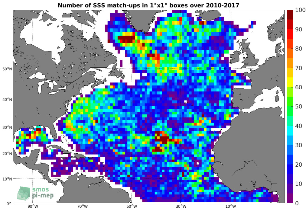
Figure 4: Number of SSS match-ups between Argo SSS and the SMOS SSS L3 v2 - Monthly - 0.25 Deg (CATDS-CECOS-IFREMER) SSS product for the North Atlantic Ocean Pi-MEP region over 1^\circ \times 1^\circ boxes and for the full satellite product period.
