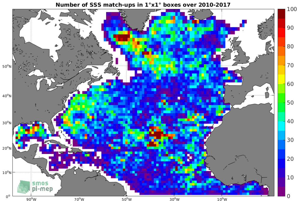
Figure 4: Number of SSS match-ups between Argo SSS and the SMOS-L3-CATDS-IFREMER-CECOS-V2-MONTHLY-0.25DEG SSS product for the North Atlantic Ocean Pi-MEP region over 1^\circ \times 1^\circ boxes and for the full satellite product period.
