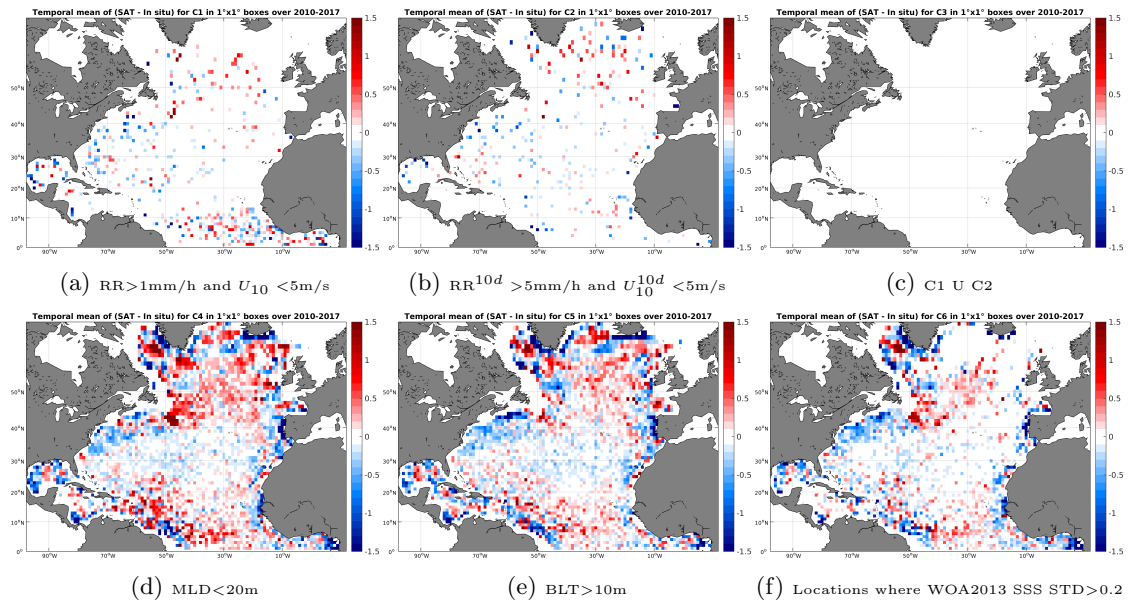
Figure 12: Temporal mean gridded over spatial boxes of size 1^\circ \times 1^\circ of \Delta SSS (SMOS-L3-CATDS-IFREMER-CECOS-V2-MONTHLY-0.25DEG - Argo) for 6 different subdatasets corresponding to: RR > 1\text{mm/h} and U_{10} < 5\text{m/s} (a), RR^{10d} > 5\text{mm/h} and U_{10}^{10d} < 5\text{m/s} (b), C1 U C2 (c), MLD < 20\text{m} (d), BLT > 10\text{m} (e), Locations where WOA2013 SSS STD > 0.2 (f).
