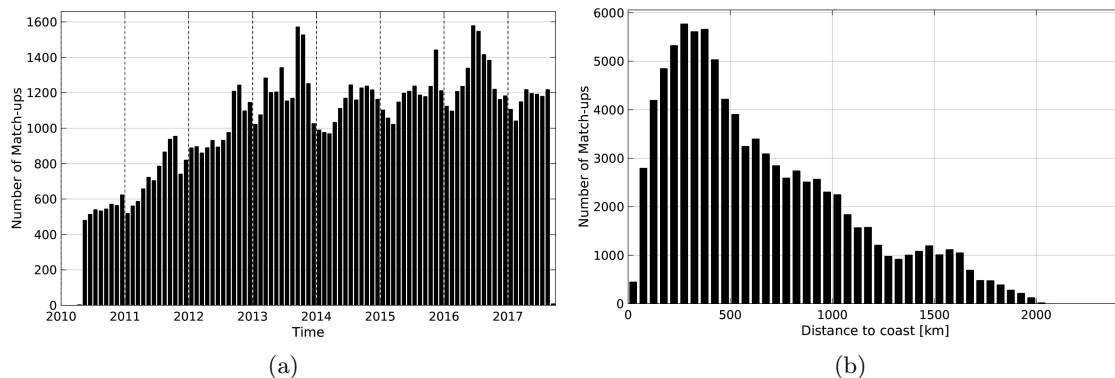
Figure 1: Number of match-ups between Argo and SMOS-L3-CATDS-IFREMER-CECOS-V2-MONTHLY-0.25DEG SSS as a function of time (a) and as function of the distance to coast (b) over the North Atlantic Ocean Pi-MEP region and for the full satellite product period.
