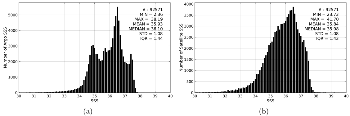
Figure 2: Histograms of SSS from Argo (a) and SMOS-L3-CATDS-IFREMER-CECOS-V2-MONTHLY-0.25DEG (b) considering all match-up pairs per bins of 0.1 over the North Atlantic Ocean Pi-MEP region and for the full satellite product period.
