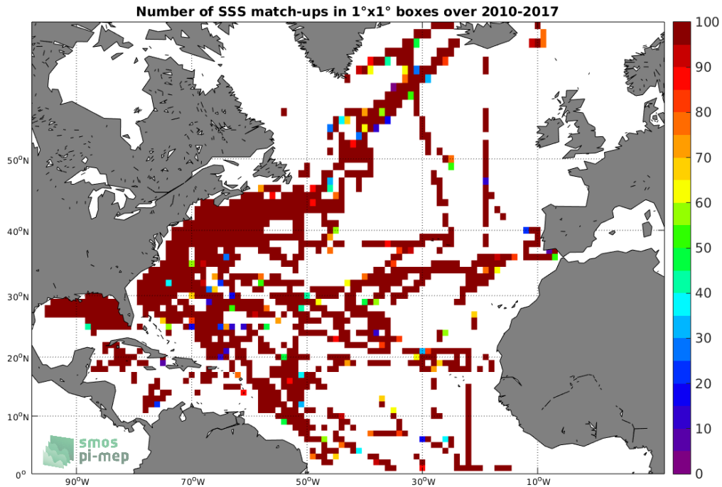
Figure 4: Number of SSS match-ups between TSG-SAMOS SSS and the SMOS L3 v2 - Daily - 0.5 Deg (CATDS-CECOS-IFREMER) SSS product for the North Atlantic Ocean Pi-MEP region over 1°x1° boxes and for the full satellite product period.
