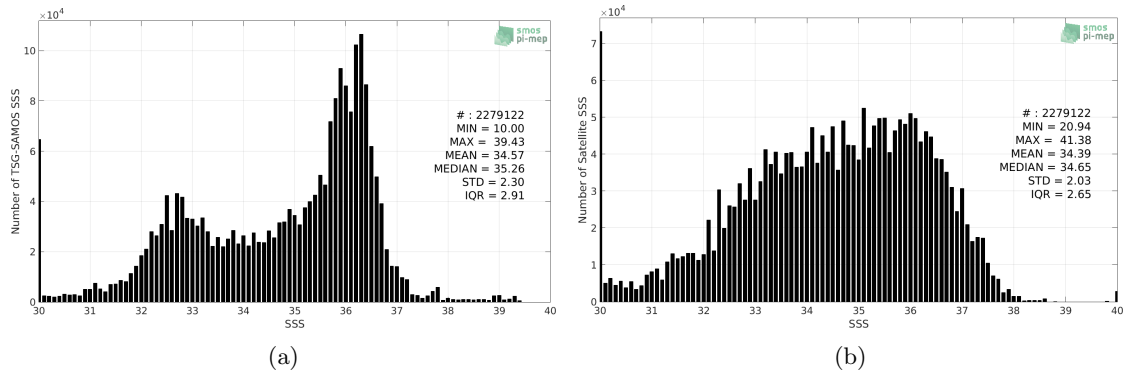
Figure 2: Histograms of SSS from TSG-SAMOS (a) and SMOS L3 v2 - Daily - 0.5 Deg (CATDS-CECOS-IFREMER) (b) considering all match-up pairs per bins of 0.1 over the North Atlantic Ocean Pi-MEP region and for the full satellite product period.
