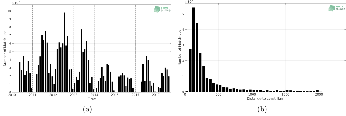
Figure 1: Number of match-ups between TSG-SAMOS and SMOS L3 v2 - Daily - 0.5 Deg (CATDS-CECOS-IFREMER) SSS as a function of time (a) and as function of the distance to coast (b) over the North Atlantic Ocean Pi-MEP region and for the full satellite product period.
