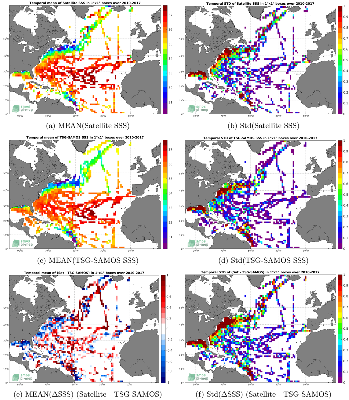
Figure 6: Temporal mean (left) and Std (right) of SSS from SMOS L3 v2 - Daily - 0.5 Deg (CATDS-CECOS-IFREMER) (top), TSG-SAMOS (middle), and of \Delta SSS (Satellite - TSG-SAMOS). Only match-up pairs are used to generate these maps.
