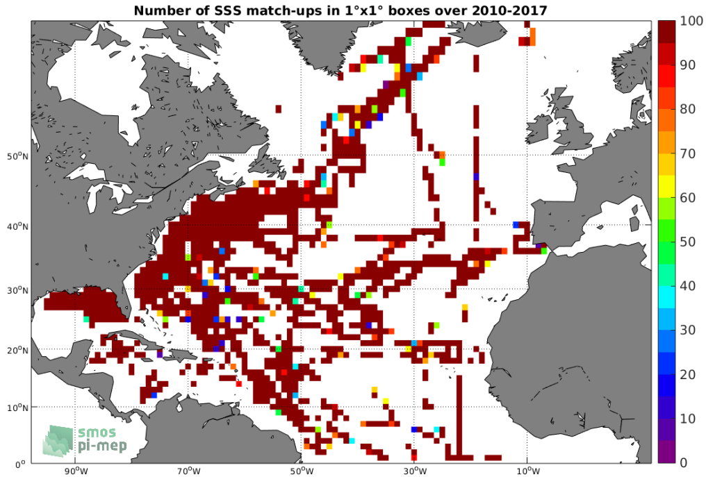
Figure 4: Number of SSS match-ups between TSG-SAMOS SSS and the SMOS-L3-CATDS-CECOS-IFREMER-V2-1DAY-0.5DEG SSS product for the North Atlantic Ocean Pi-MEP region over 1°x1° boxes and for the full satellite product period.
