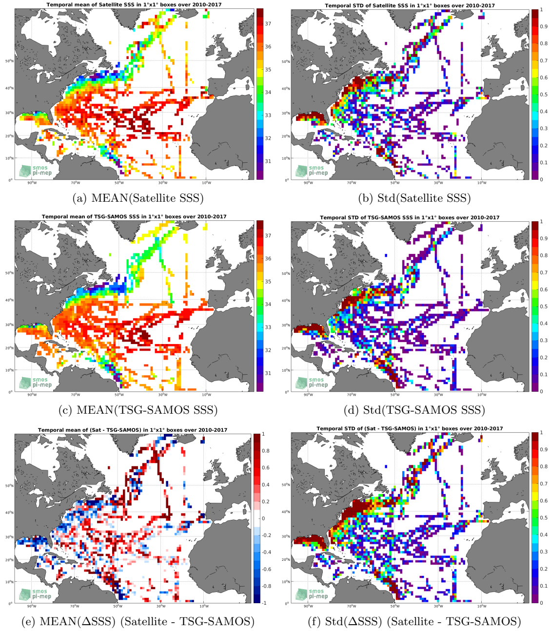
Figure 6: Temporal mean (left) and Std (right) of SSS from SMOS-L3-CATDS-CECOS-IFREMER-V2-1DAY-0.5DEG (top), TSG-SAMOS (middle), and of \Delta SSS (Satellite - TSG-SAMOS). Only match-up pairs are used to generate these maps.
