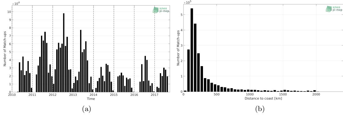
Figure 1: Number of match-ups between TSG-SAMOS and SMOS-L3-CATDS-CECOS-IFREMER-V2-1DAY-0.5DEG SSS as a function of time (a) and as function of the distance to coast (b) over the North Atlantic Ocean Pi-MEP region and for the full satellite product period.
