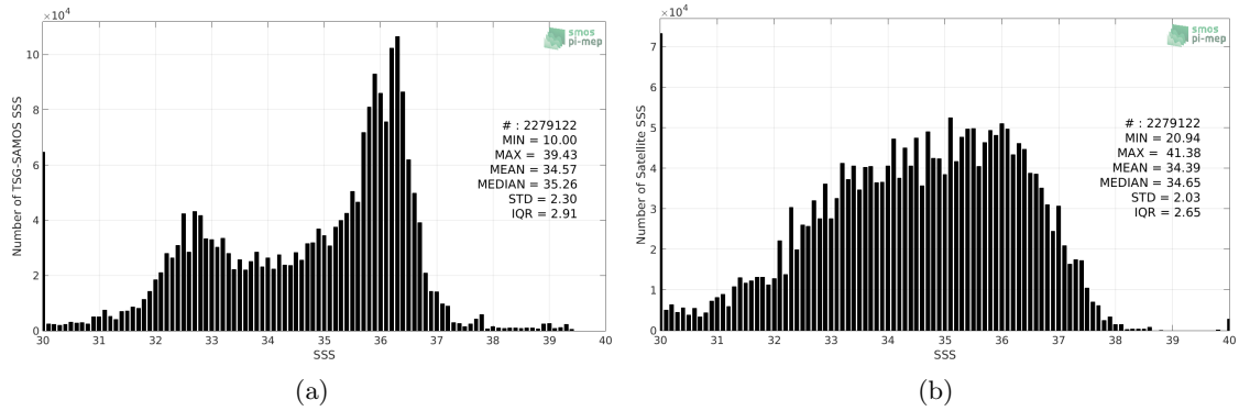
Figure 2: Histograms of SSS from TSG-SAMOS (a) and SMOS-L3-CATDS-CECOS-IFREMER-V2-1DAY-0.5DEG (b) considering all match-up pairs per bins of 0.1 over the North Atlantic Ocean Pi-MEP region and for the full satellite product period.
