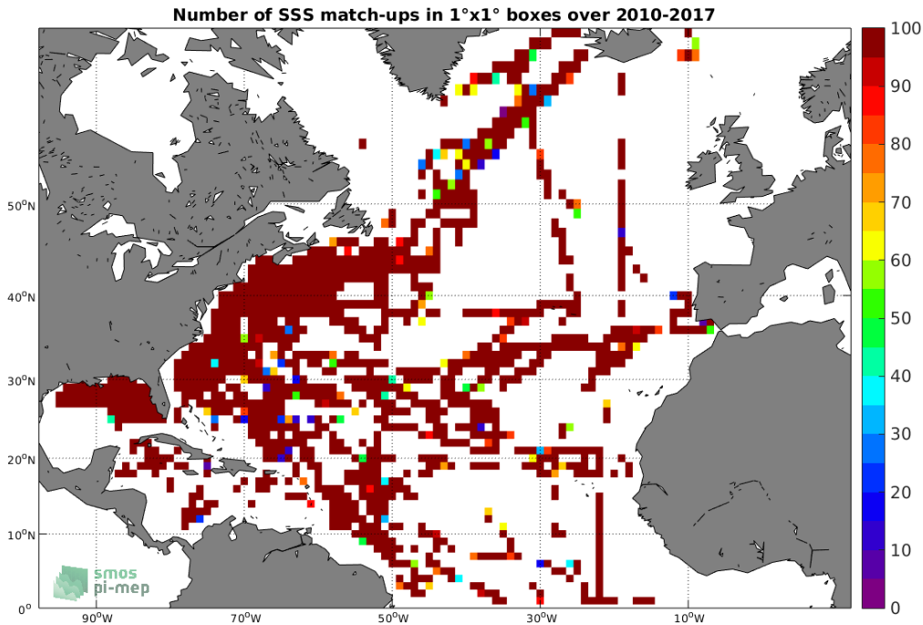
Figure 4: Number of SSS match-ups between TSG-SAMOS SSS and the SMOS-L3-CATDS-CECOS-IFREMER-V2-1DAY-0.5DEG SSS product for the North Atlantic Ocean Pi-MEP region over 1^\circ \times 1^\circ boxes and for the full satellite product period.
