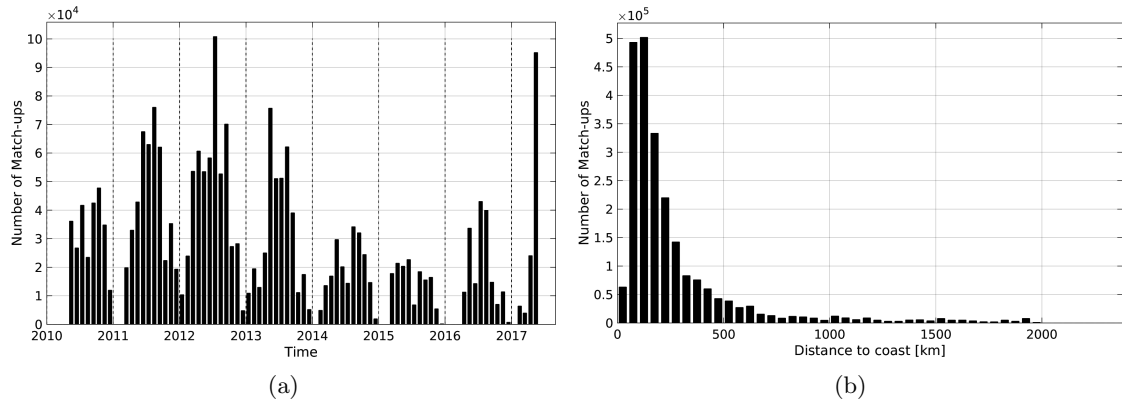
Figure 1: Number of match-ups between TSG-SAMOS and SMOS-L3-CATDS-CECOS-IFREMER-V2-1DAY-0.5deg SSS as a function of time (a) and as function of the distance to coast (b) over the North Atlantic Ocean Pi-MEP region and for the full satellite product period.
