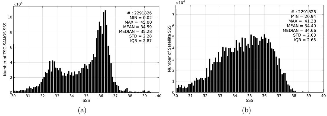
Figure 2: Histograms of SSS from TSG-SAMOS (a) and SMOS-L3-CATDS-CECOS-IFREMER-V2-1DAY-0.5deg (b) considering all match-up pairs per bins of 0.1 over the North Atlantic Ocean Pi-MEP region and for the full satellite product period.
