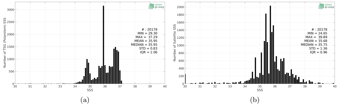
Figure 2: Histograms of SSS from TSG (Polarstern) (a) and SMOS SSS L3 v2 - Daily - 0.5 Deg (CATDS-CECOS-IFREMER) (b) considering all match-up pairs per bins of 0.1 over the North Atlantic Ocean Pi-MEP region and for the full satellite product period.
