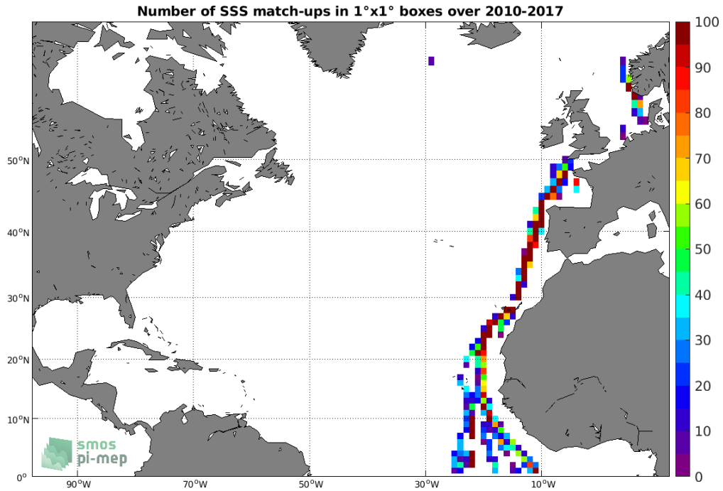
Figure 4: Number of SSS match-ups between TSG (Polarstern) SSS and the SMOS SSS L3 v2 - Daily - 0.5 Deg (CATDS-CECOS-IFREMER) SSS product for the North Atlantic Ocean Pi-MEP region over 1^\circ \times 1^\circ boxes and for the full satellite product period.
