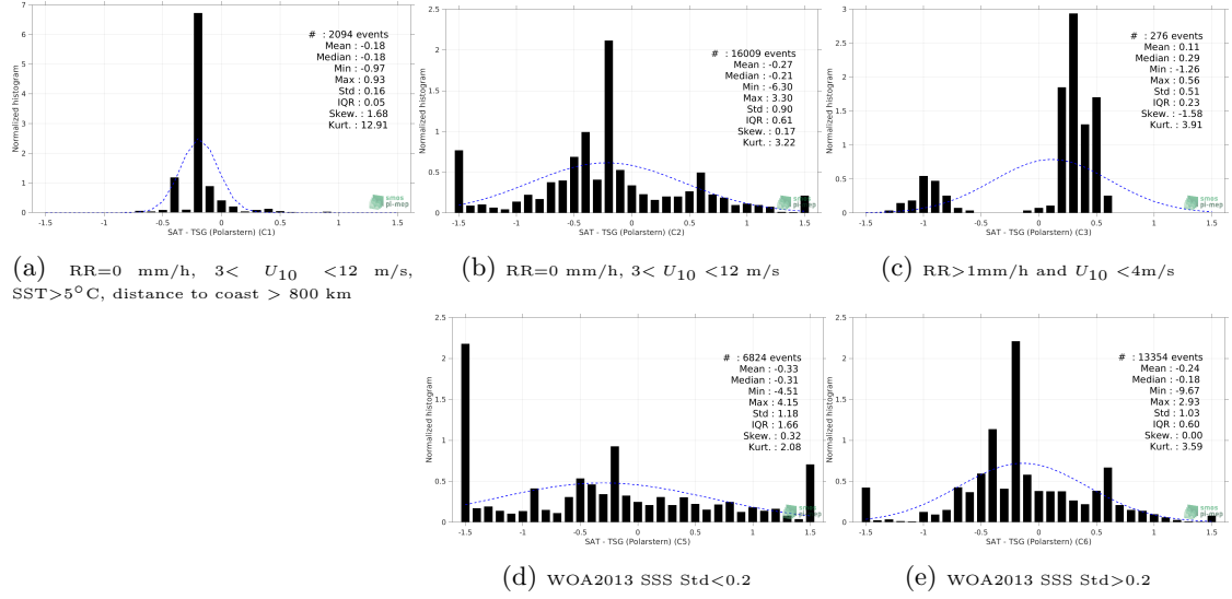
Figure 13: Normalized histogram of \Delta SSS (SMOS SSS L3 v2 - Daily - 0.5 Deg (CATDS-CECOS-IFREMER) - TSG (Polarstern)) for 5 different subdatasets corresponding to: RR=0 mm/h, 3 < U_{10} < 12 m/s, SST>5°C, distance to coast > 800 km (a), RR=0 mm/h, 3 < U_{10} < 12 m/s (b), RR>1mm/h and U_{10} < 4 m/s (c), WOA2013 SSS Std<0.2 (d), WOA2013 SSS Std>0.2 (e).
