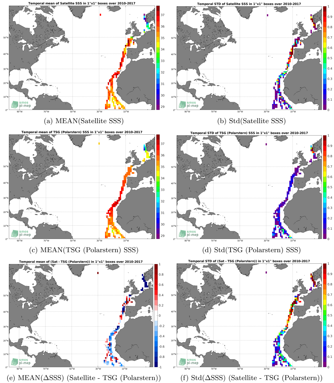
Figure 6: Temporal mean (left) and Std (right) of SSS from SMOS SSS L3 v2 - Daily - 0.5 Deg (CATDS-CECOS-IFREMER) (top), TSG (Polarstern) (middle), and of \Delta SSS (Satellite - TSG (Polarstern)). Only match-up pairs are used to generate these maps.
