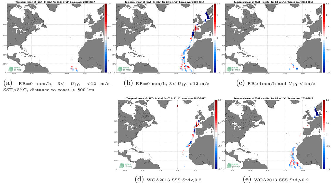
Figure 12: Temporal mean gridded over spatial boxes of size 1^\circ \times 1^\circ of \Delta SSS (SMOS SSS L3 v2 - Daily - 0.5 Deg (CATDS-CECOS-IFREMER) - TSG (Polarstern)) for 5 different subdatasets corresponding to:RR=0 mm/h, 3 < U_{10} < 12 m/s, SST >5^\circ\text{C} , distance to coast > 800 km (a), RR=0 mm/h, 3 < U_{10} < 12 m/s (b), RR >1 mm/h and U_{10} < 4 m/s (c), WOA2013 SSS Std <0.2 (d), WOA2013 SSS Std >0.2 (e).
