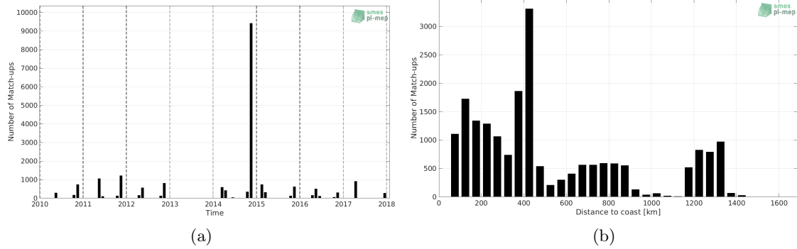
Figure 1: Number of match-ups between TSG (Polarstern) and SMOS SSS L3 v2 - Daily - 0.5 Deg (CATDS-CECOS-IFREMER) SSS as a function of time (a) and as function of the distance to coast (b) over the North Atlantic Ocean Pi-MEP region and for the full satellite product period.
