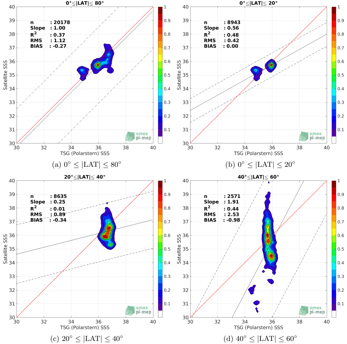
Figure 9: Contour maps of the concentration of SMOS SSS L3 v2 - Daily - 0.5 Deg (CATDS-CECOS-IFREMER) SSS (y-axis) versus TSG (Polarstern) SSS (x-axis) at match-up pairs for different latitude bands. For each plot, the red line shows x=y . The black thin and dashed lines indicate a linear fit through the data cloud and the \pm 95\% confidence levels, respectively. The number match-up pairs n , the slope and R^2 coefficient of the linear fit, the root mean square (RMS) and the mean bias between satellite and in situ data are indicated for each latitude band in each plots.
