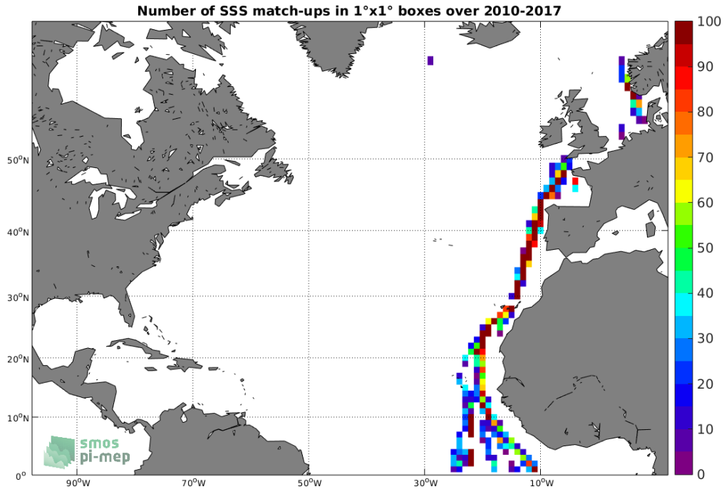
Figure 4: Number of SSS match-ups between TSG-POLARSTERN SSS and the SMOS L3 v2 - Daily - 0.5 Deg (CATDS-CECOS-IFREMER) SSS product for the North Atlantic Ocean Pi-MEP region over 1^\circ \times 1^\circ boxes and for the full satellite product period.
