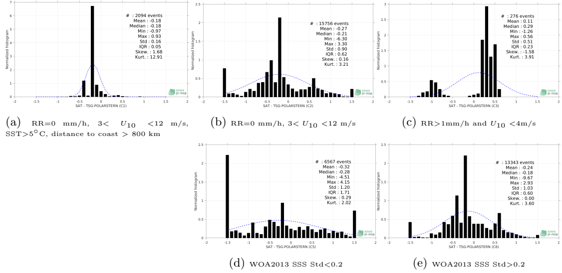
Figure 13: Normalized histogram of \Delta SSS (SMOS L3 v2 - Daily - 0.5 Deg (CATDS-CECOS-IFREMER) - TSG-POLARSTERN) for 5 different subdatasets corresponding to: RR=0 mm/h, 3 < U_{10} < 12 m/s, SST>5°C, distance to coast > 800 km (a), RR=0 mm/h, 3 < U_{10} < 12 m/s (b), RR>1mm/h and U_{10} < 4 m/s (c), WOA2013 SSS Std<0.2 (d), WOA2013 SSS Std>0.2 (e).
