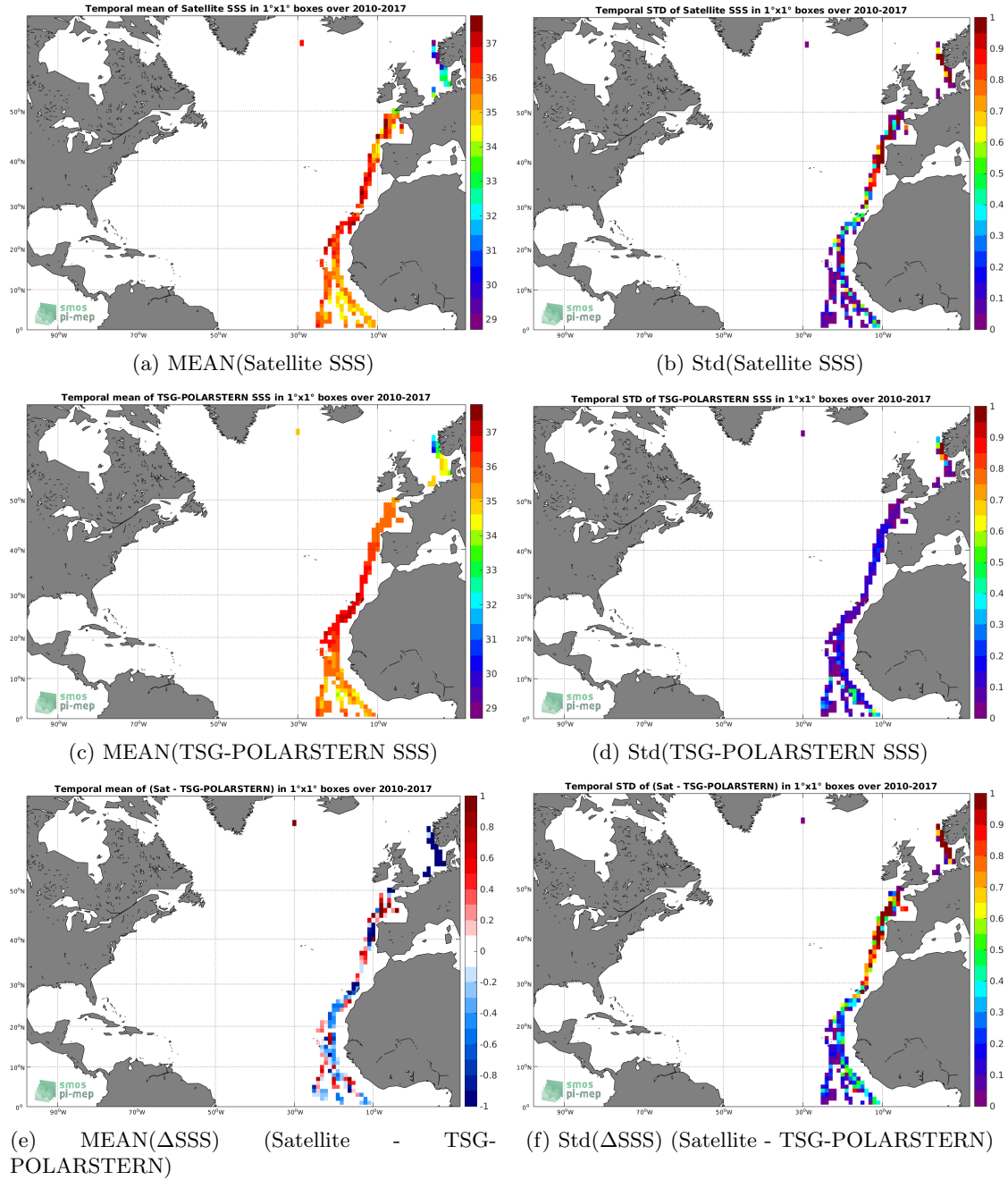
Figure 6: Temporal mean (left) and Std (right) of SSS from SMOS L3 v2 - Daily - 0.5 Deg (CATDS-CECOS-IFREMER) (top), TSG-POLARSTERN (middle), and of \Delta SSS (Satellite - TSG-POLARSTERN). Only match-up pairs are used to generate these maps.
