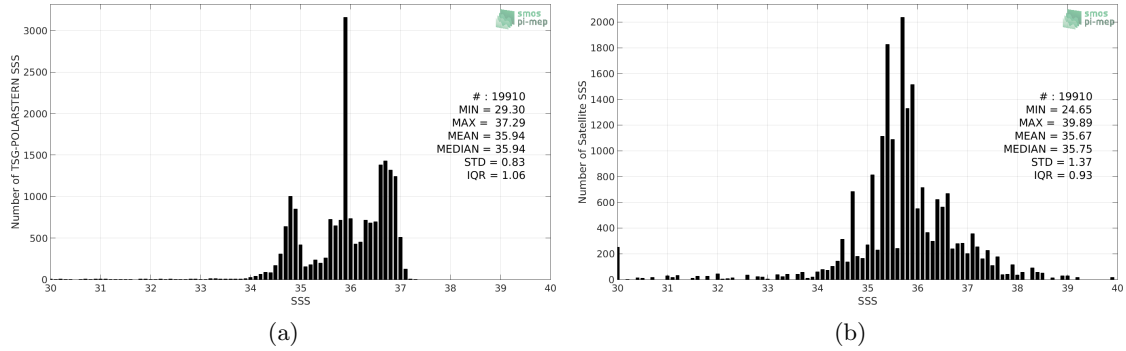
Figure 2: Histograms of SSS from TSG-POLARSTERN (a) and SMOS L3 v2 - Daily - 0.5 Deg (CATDS-CECOS-IFREMER) (b) considering all match-up pairs per bins of 0.1 over the North Atlantic Ocean Pi-MEP region and for the full satellite product period.
