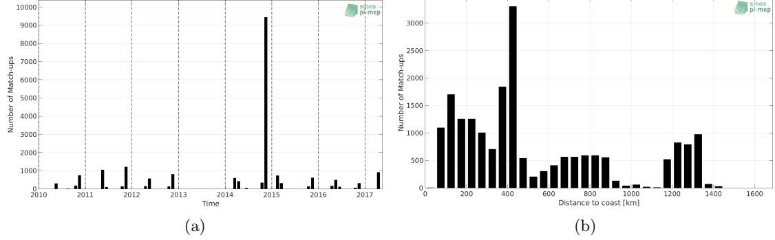
Figure 1: Number of match-ups between TSG-POLARSTERN and SMOS L3 v2 - Daily - 0.5 Deg (CATDS-CECOS-IFREMER) SSS as a function of time (a) and as function of the distance to coast (b) over the North Atlantic Ocean Pi-MEP region and for the full satellite product period.
