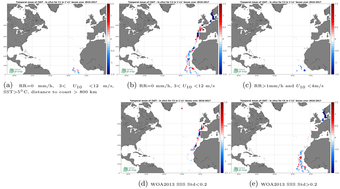
Figure 12: Temporal mean gridded over spatial boxes of size 1^\circ \times 1^\circ of \Delta SSS (SMOS L3 v2 - Daily - 0.5 Deg (CATDS-CECOS-IFREMER) - TSG-POLARSTERN) for 5 different subdatasets corresponding to: RR=0 mm/h, 3 < U_{10} < 12 m/s, SST > 5^\circ C , distance to coast > 800 km (a), RR=0 mm/h, 3 < U_{10} < 12 m/s (b), RR > 1 mm/h and U_{10} < 4 m/s (c), WOA2013 SSS Std < 0.2 (d), WOA2013 SSS Std > 0.2 (e).
