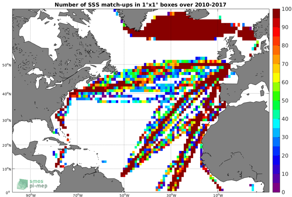
Figure 4: Number of SSS match-ups between TSG-LEGOS-DM SSS and the SMOS-L3-CATDS-CECOS-IFREMER-V2-1DAY-0.5DEG SSS product for the North Atlantic Ocean Pi-MEP region over 1^\circ \times 1^\circ boxes and for the full satellite product period.
