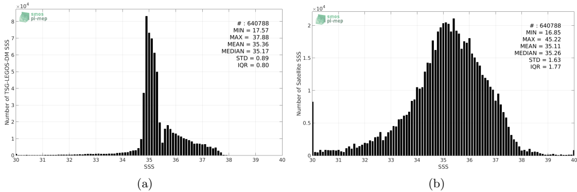
Figure 2: Histograms of SSS from TSG-LEGOS-DM (a) and SMOS-L3-CATDS-CECOS-IFREMER-V2-1DAY-0.5DEG (b) considering all match-up pairs per bins of 0.1 over the North Atlantic Ocean Pi-MEP region and for the full satellite product period.
