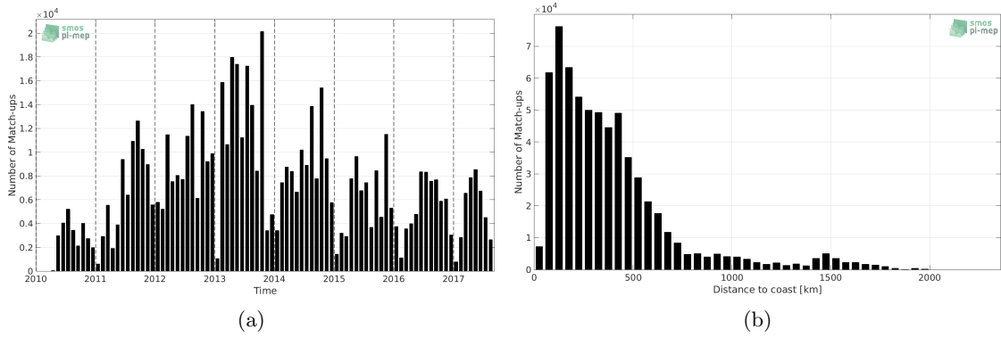
Figure 1: Number of match-ups between TSG-LEGOS-DM and SMOS-L3-CATDS-CECOS-IFREMER-V2-1DAY-0.5DEG SSS as a function of time (a) and as function of the distance to coast (b) over the North Atlantic Ocean Pi-MEP region and for the full satellite product period.
