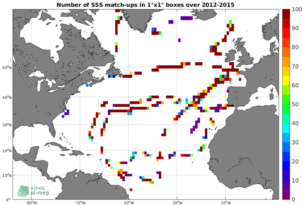
Figure 4: Number of SSS match-ups between TSG-GOSUD-Sailing-ship SSS and the SMOS-L3-CATDS-CECOS-IFREMER-V2-1DAY-0.5DEG SSS product for the North Atlantic Ocean Pi-MEP region over 1^\circ \times 1^\circ boxes and for the full satellite product period.
