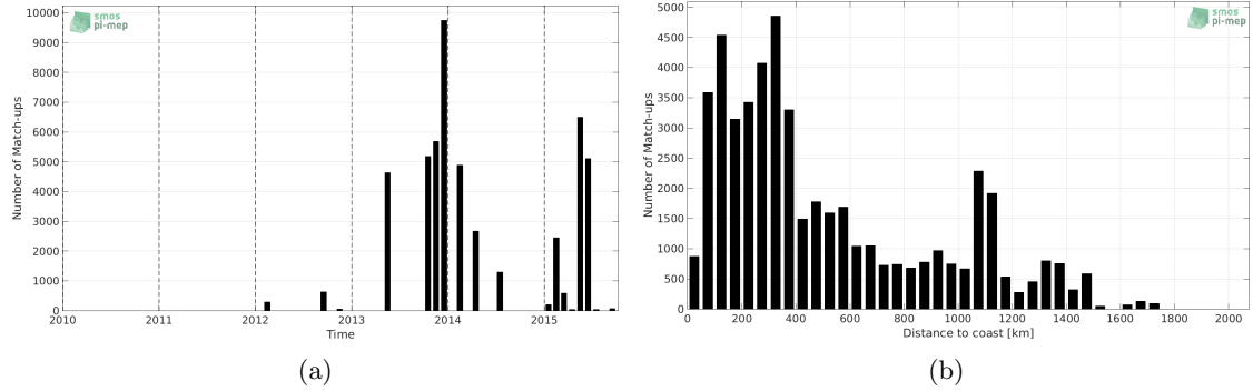
Figure 1: Number of match-ups between TSG-GOSUD-Sailing-ship and SMOS-L3-CATDS-CECOS-IFREMER-V2-1DAY-0.5DEG SSS as a function of time (a) and as function of the distance to coast (b) over the North Atlantic Ocean Pi-MEP region and for the full satellite product period.
