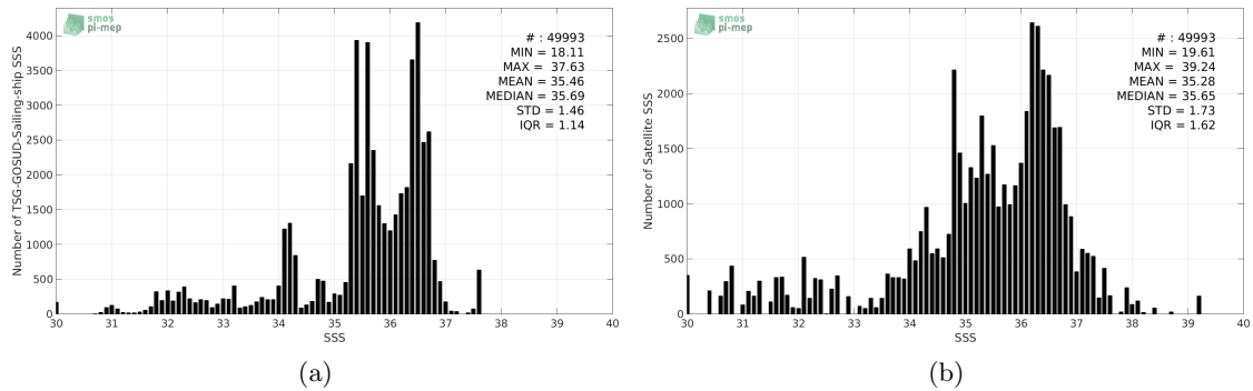
Figure 2: Histograms of SSS from TSG-GOSUD-Sailing-ship (a) and SMOS-L3-CATDS-CECOS-IFREMER-V2-1DAY-0.5DEG (b) considering all match-up pairs per bins of 0.1 over the North Atlantic Ocean Pi-MEP region and for the full satellite product period.
