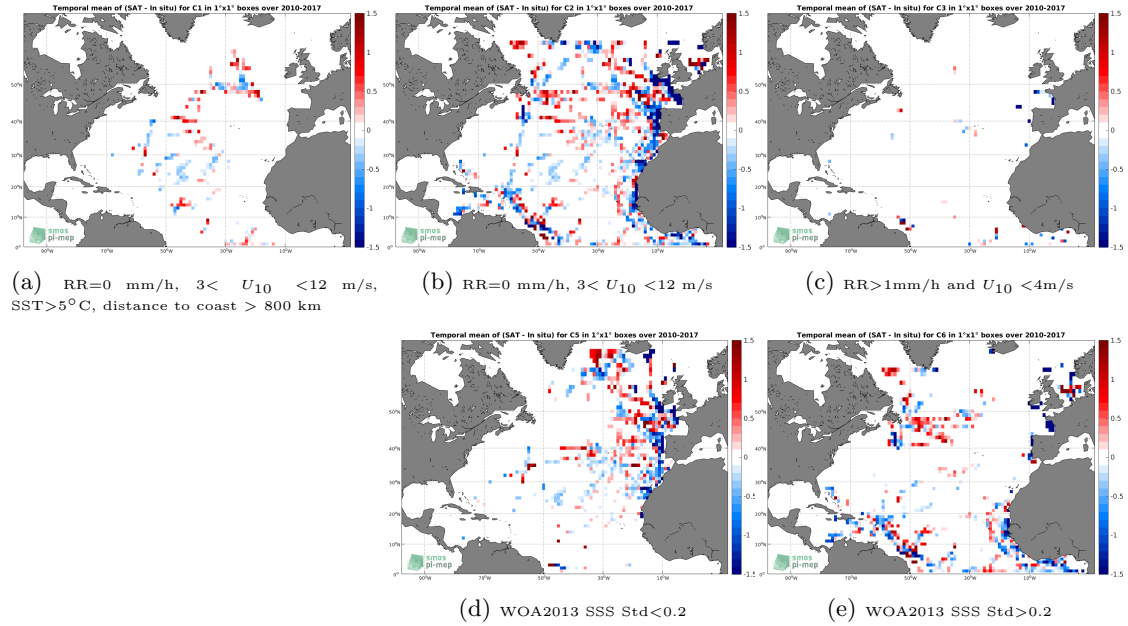
Figure 12: Temporal mean gridded over spatial boxes of size 1^\circ \times 1^\circ of \Delta SSS (SMOS SSS L3 v2 - Daily - 0.5 Deg (CATDS-CECOS-IFREMER) - TSG (GOSUD-Research-vessel)) for 5 different subdatasets corresponding to:RR=0 mm/h, 3 < U_{10} < 12 m/s, SST >5^\circ\text{C} , distance to coast > 800 km (a), RR=0 mm/h, 3 < U_{10} < 12 m/s (b), RR >1 mm/h and U_{10} < 4 m/s (c), WOA2013 SSS Std <0.2 (d), WOA2013 SSS Std >0.2 (e).
