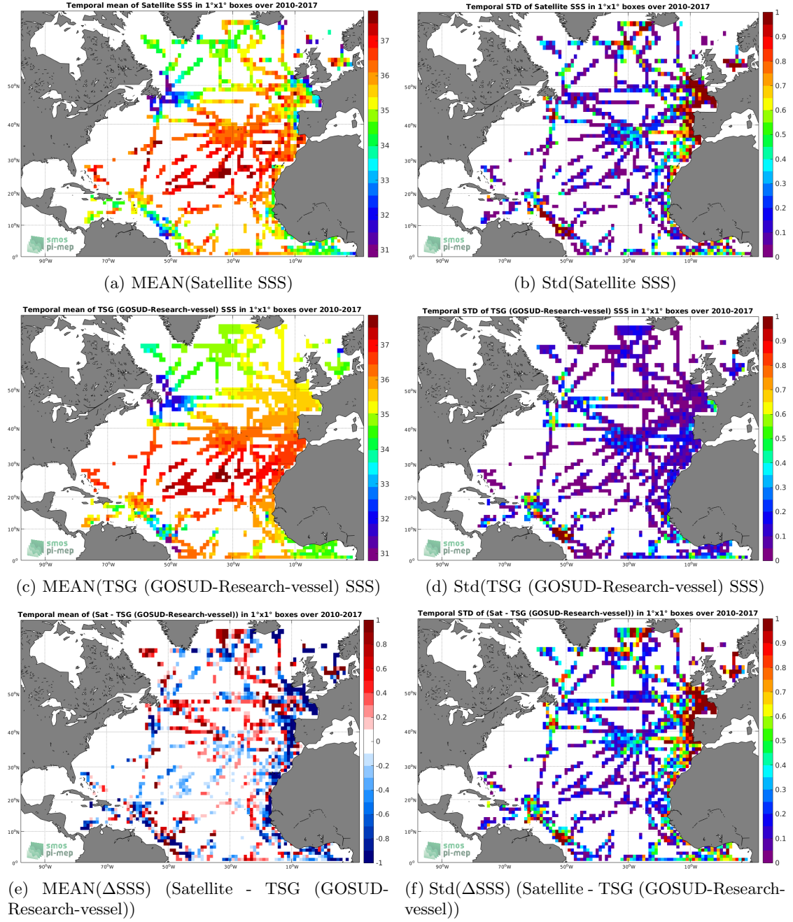
Figure 6: Temporal mean (left) and Std (right) of SSS from SMOS SSS L3 v2 - Daily - 0.5 Deg (CATDS-CECOS-IFREMER) (top), TSG (GOSUD-Research-vessel) (middle), and of \Delta SSS (Satellite - TSG (GOSUD-Research-vessel)). Only match-up pairs are used to generate these maps.
