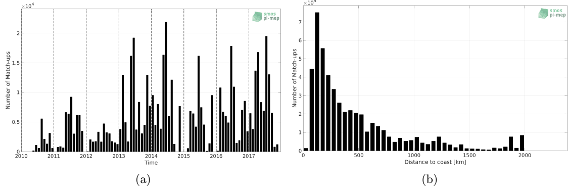
Figure 1: Number of match-ups between TSG (GOSUD-Research-vessel) and SMOS SSS L3 v2 - Daily - 0.5 Deg (CATDS-CECOS-IFREMER) SSS as a function of time (a) and as function of the distance to coast (b) over the North Atlantic Ocean Pi-MEP region and for the full satellite product period.
