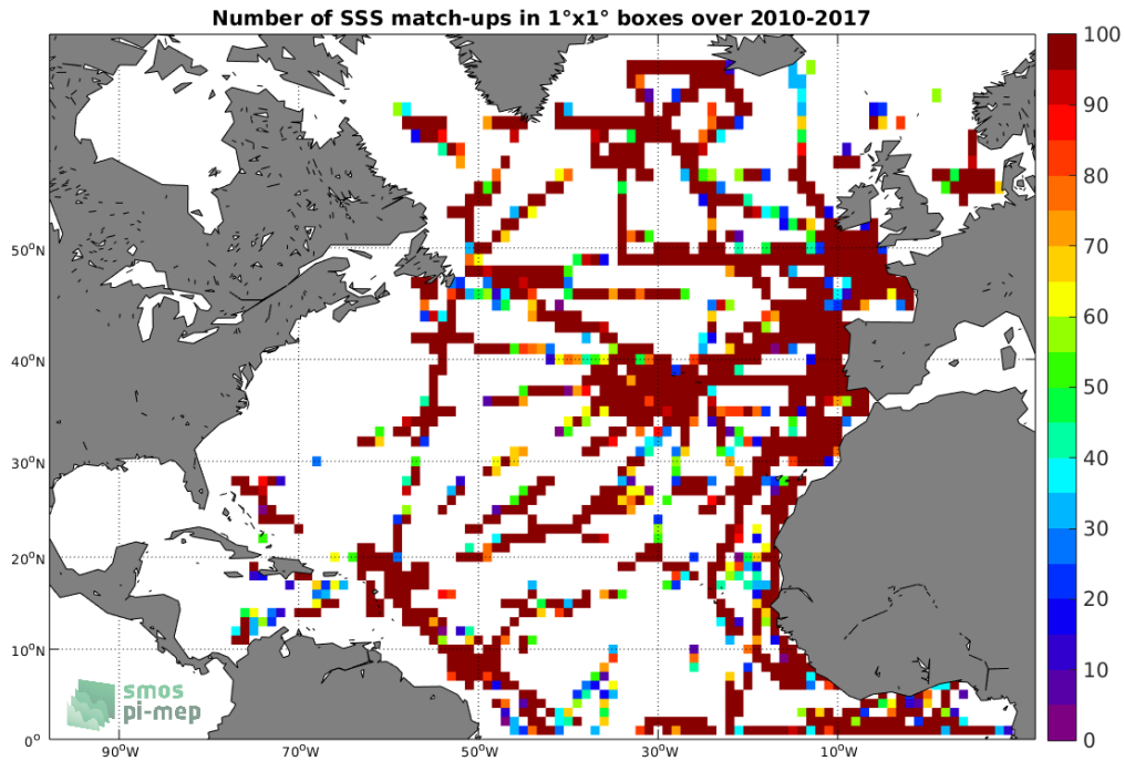
Figure 4: Number of SSS match-ups between TSG (GOSUD-Research-vessel) SSS and the SMOS SSS L3 v2 - Daily - 0.5 Deg (CATDS-CECOS-IFREMER) SSS product for the North Atlantic Ocean Pi-MEP region over 1°x1° boxes and for the full satellite product period.
