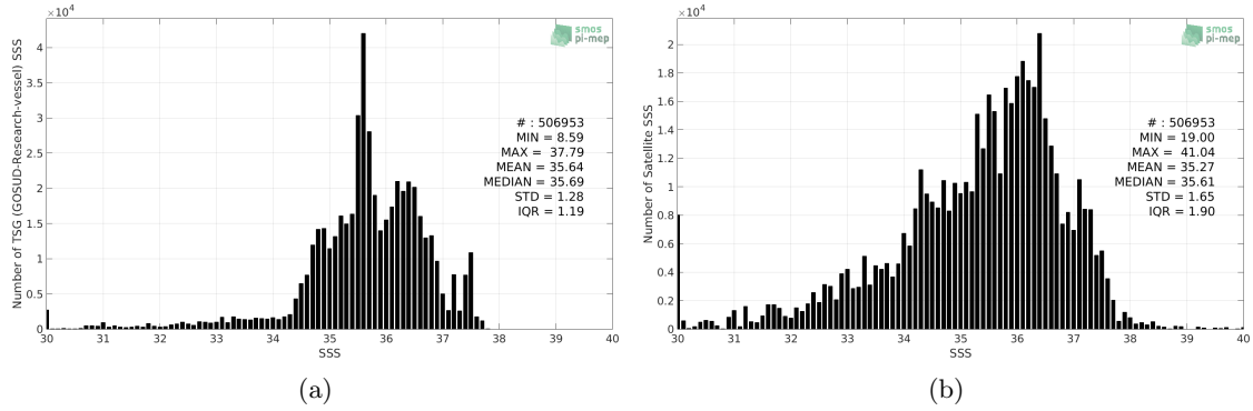
Figure 2: Histograms of SSS from TSG (GOSUD-Research-vessel) (a) and SMOS SSS L3 v2 - Daily - 0.5 Deg (CATDS-CECOS-IFREMER) (b) considering all match-up pairs per bins of 0.1 over the North Atlantic Ocean Pi-MEP region and for the full satellite product period.
