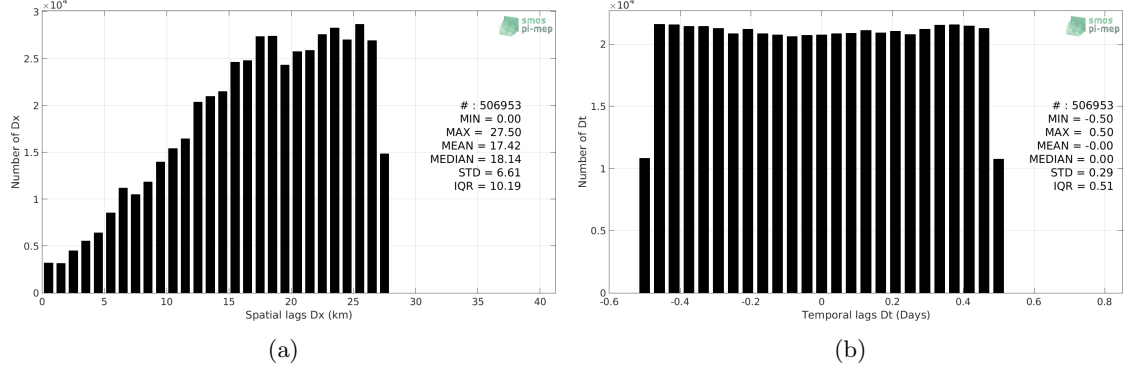
Figure 5: Histograms of the spatial (a) and temporal (b) lags between the time of the TSG (GOSUD-Research-vessel) measurements and the date of the corresponding SMOS SSS L3 v2 - Daily - 0.5 Deg (CATDS-CECOS-IFREMER) SSS product.
