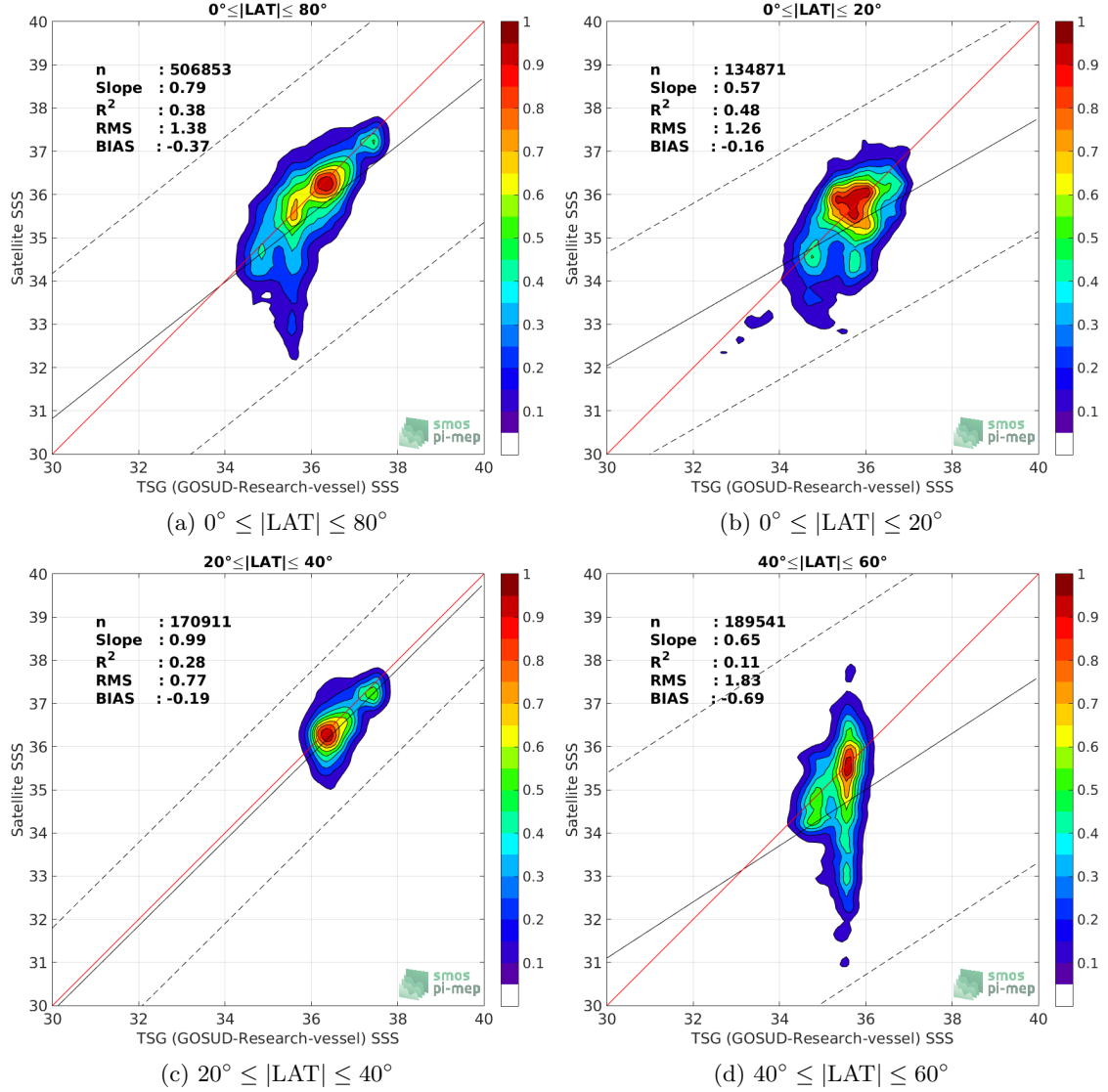
Figure 9: Contour maps of the concentration of SMOS SSS v2 - Daily - 0.5 Deg (CATDS-CECOS-IFREMER) SSS (y-axis) versus TSG (GOSUD-Research-vessel) SSS (x-axis) at match-up pairs for different latitude bands. For each plot, the red line shows x=y . The black thin and dashed lines indicate a linear fit through the data cloud and the \pm 95\% confidence levels, respectively. The number match-up pairs n , the slope and R^2 coefficient of the linear fit, the root mean square (RMS) and the mean bias between satellite and in situ data are indicated for each latitude band in each plots.
