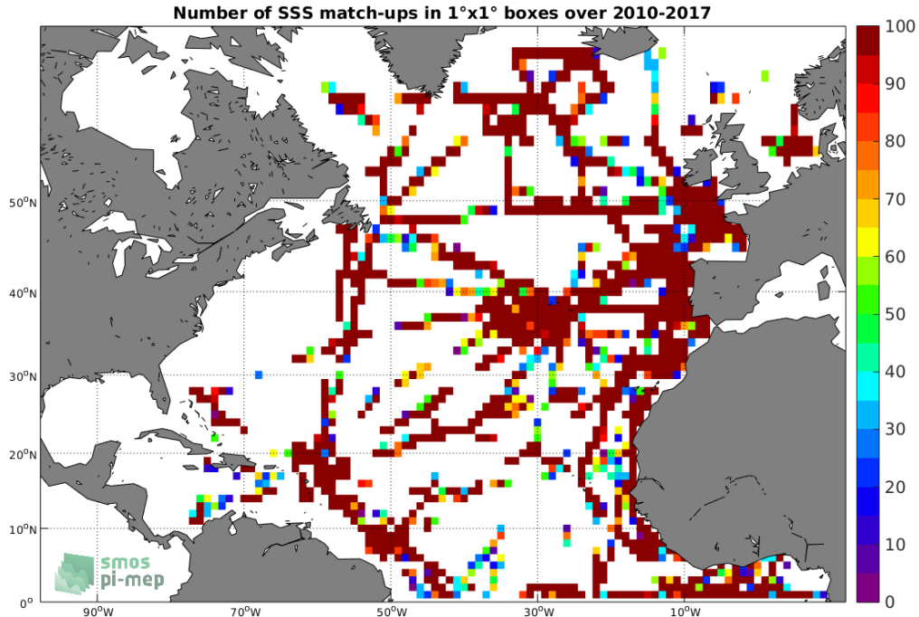
Figure 4: Number of SSS match-ups between TSG-GOSUD-Research-vessel SSS and the SMOS-L3-CATDS-CECOS-IFREMER-V2-1DAY-0.5DEG SSS product for the North Atlantic Ocean Pi-MEP region over 1^\circ \times 1^\circ boxes and for the full satellite product period.
