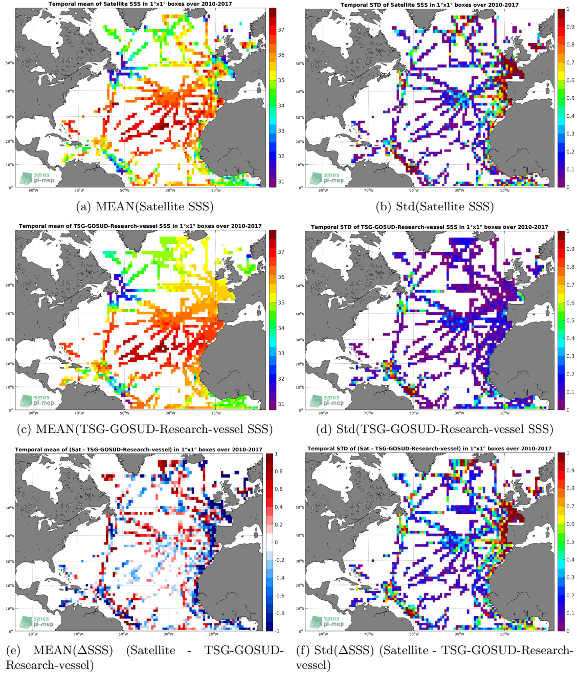
Figure 6: Temporal mean (left) and Std (right) of SSS from SMOS-L3-CATDS-CECOS-IFREMER-V2-1DAY-0.5DEG (top), TSG-GOSUD-Research-vessel (middle), and of \Delta SSS (Satellite - TSG-GOSUD-Research-vessel). Only match-up pairs are used to generate these maps.
