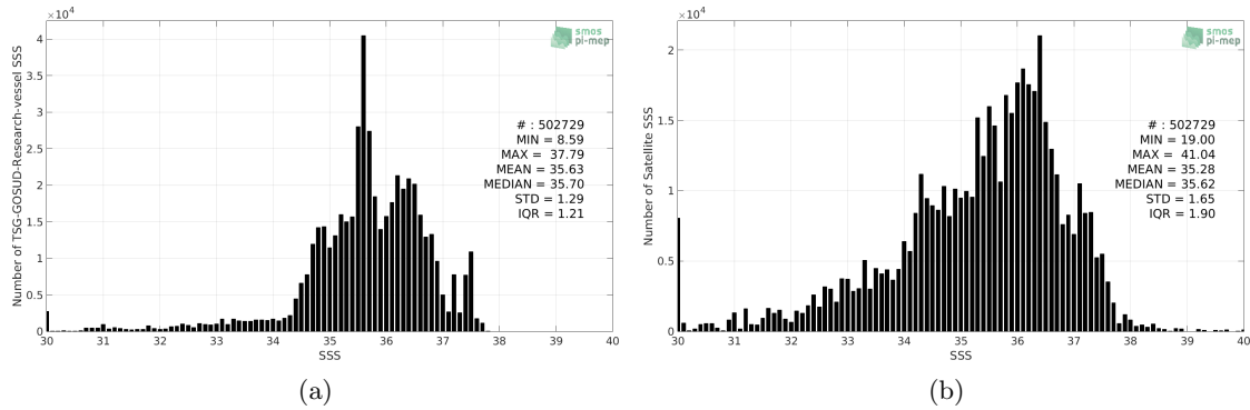
Figure 2: Histograms of SSS from TSG-GOSUD-Research-vessel (a) and SMOS-L3-CATDS-CECOS-IFREMER-V2-1DAY-0.5DEG (b) considering all match-up pairs per bins of 0.1 over the North Atlantic Ocean Pi-MEP region and for the full satellite product period.
