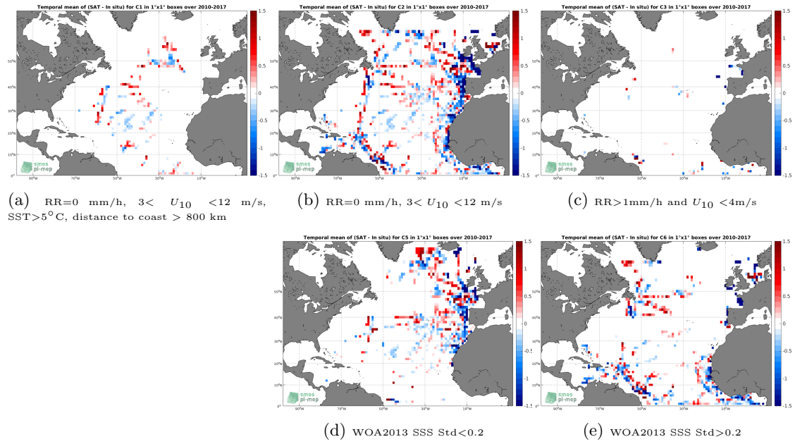
Figure 12: Temporal mean gridded over spatial boxes of size 1^\circ \times 1^\circ of \Delta SSS (SMOS-L3-CATDS-CECOS-IFREMER-V2-1DAY-0.5DEG - TSG-GOSUD-Research-vessel) for 5 different subdatasets corresponding to: RR=0 mm/h, 3 < U_{10} < 12 m/s, SST >5^\circ C, distance to coast > 800 km (a), RR=0 mm/h, 3 < U_{10} < 12 m/s (b), RR >1 mm/h and U_{10} < 4 m/s (c), WOA2013 SSS Std <0.2 (d), WOA2013 SSS Std >0.2 (e).
