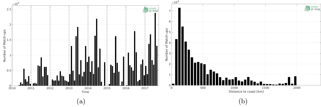
Figure 1: Number of match-ups between TSG-GOSUD-Research-vessel and SMOS-L3-CATDS-CECOS-IFREMER-V2-1DAY-0.5DEG SSS as a function of time (a) and as function of the distance to coast (b) over the North Atlantic Ocean Pi-MEP region and for the full satellite product period.
