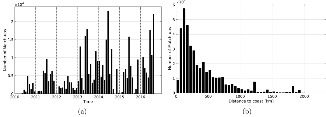
Figure 1: Number of match-ups between TSG-GOSUD-Research-vessel and SMOS-L3-CATDS-CECOS-IFREMER-V2-1DAY-0.5deg SSS as a function of time (a) and as function of the distance to coast (b) over the North Atlantic Ocean Pi-MEP region and for the full satellite product period.
