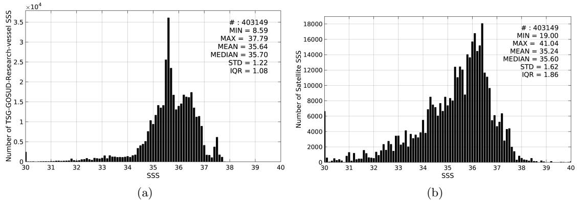
Figure 2: Histograms of SSS from TSG-GOSUD-Research-vessel (a) and SMOS-L3-CATDS-CECOS-IFREMER-V2-1DAY-0.5deg (b) considering all match-up pairs per bins of 0.1 over the North Atlantic Ocean Pi-MEP region and for the full satellite product period.
