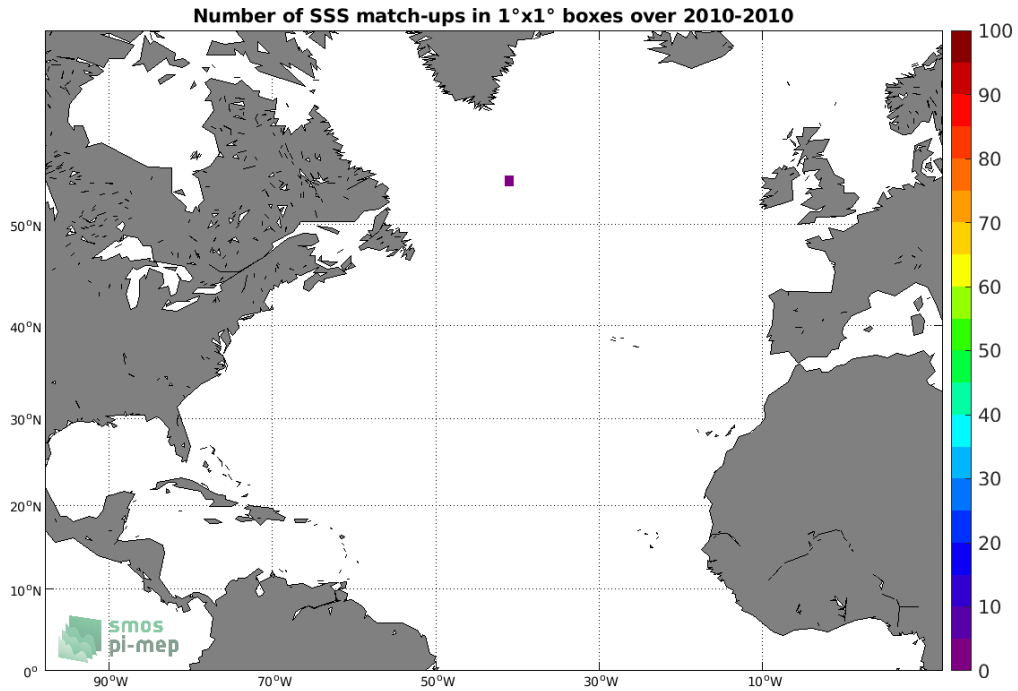
Figure 4: Number of SSS match-ups between Sea mammals SSS and the SMOS SSS L3 v2 - Daily - 0.5 Deg (CATDS-CECOS-IFREMER) SSS product for the North Atlantic Ocean Pi-MEP region over 1^\circ \times 1^\circ boxes and for the full satellite product period.
