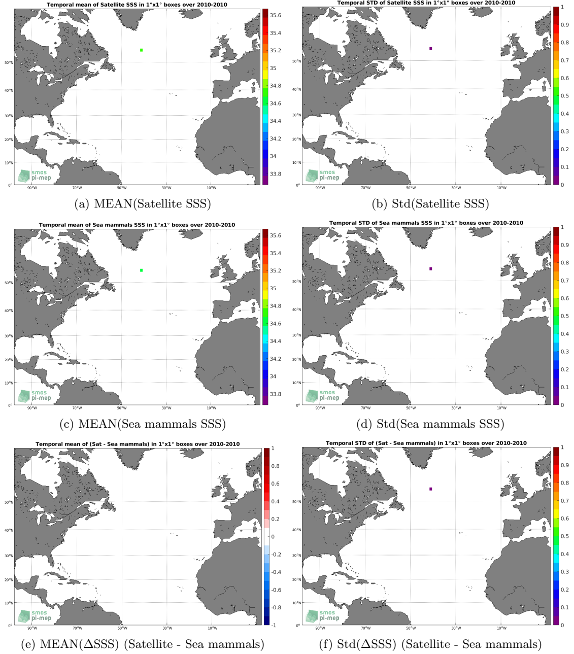
Figure 6: Temporal mean (left) and Std (right) of SSS from SMOS SSS L3 v2 - Daily - 0.5 Deg (CATDS-CECOS-IFREMER) (top), Sea mammals (middle), and of \Delta SSS (Satellite - Sea mammals). Only match-up pairs are used to generate these maps.
