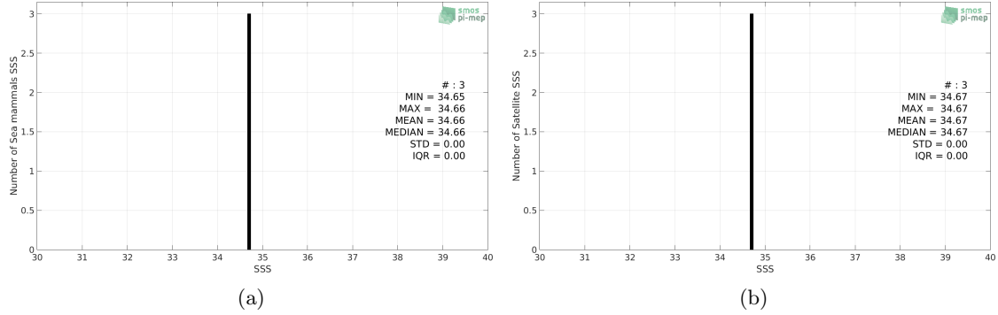
Figure 2: Histograms of SSS from Sea mammals (a) and SMOS L3 v2 - Daily - 0.5 Deg (CATDS-CECOS-IFREMER) (b) considering all match-up pairs per bins of 0.1 over the North Atlantic Ocean Pi-MEP region and for the full satellite product period.
