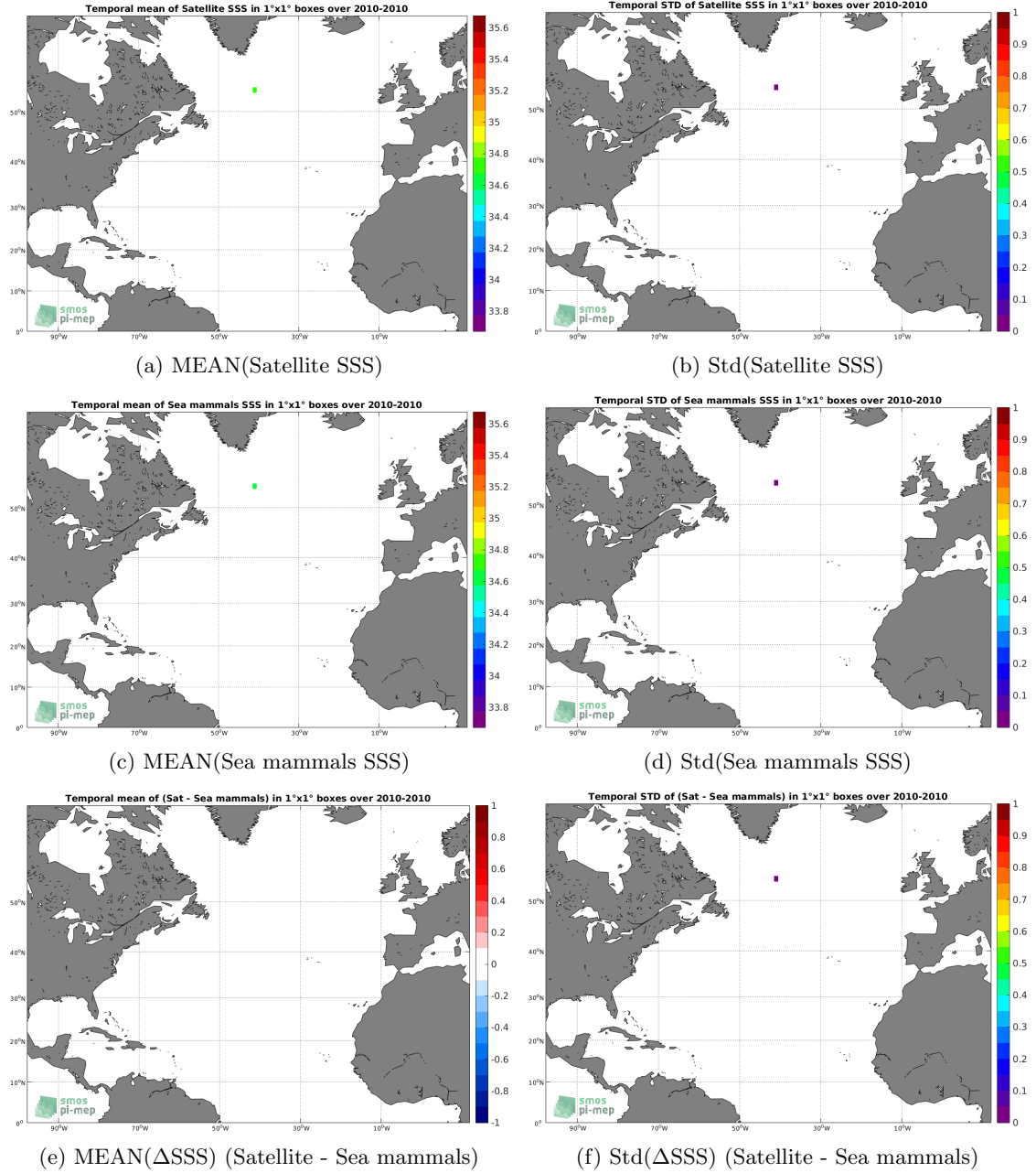
Figure 6: Temporal mean (left) and Std (right) of SSS from SMOS L3 v2 - Daily - 0.5 Deg (CATDS-CECOS-IFREMER) (top), Sea mammals (middle), and of \Delta SSS (Satellite - Sea mammals). Only match-up pairs are used to generate these maps.
