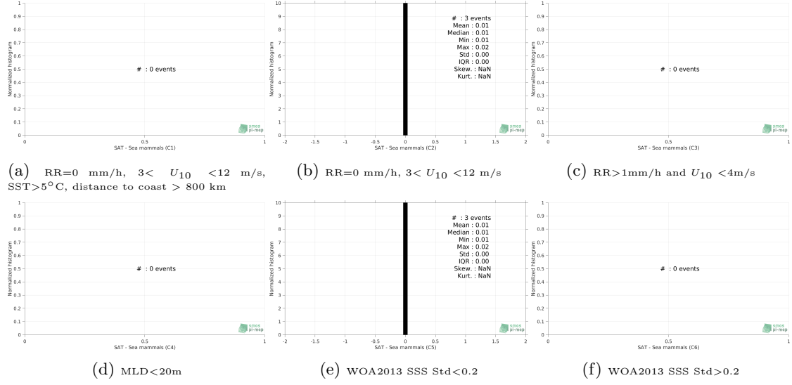
Figure 13: Normalized histogram of \Delta SSS (SMOS L3 v2 - Daily - 0.5 Deg (CATDS-CECOS-IFREMER) - Sea mammals) for 6 different subdatasets corresponding to: RR=0 mm/h, 3 < U_{10} < 12 m/s, SST > 5^{\circ}C , distance to coast > 800 km (a), RR=0 mm/h, 3 < U_{10} < 12 m/s (b), RR > 1 mm/h and U_{10} < 4 m/s (c), MLD < 20 m (d), WOA2013 SSS Std < 0.2 (e), WOA2013 SSS Std > 0.2 (f).
