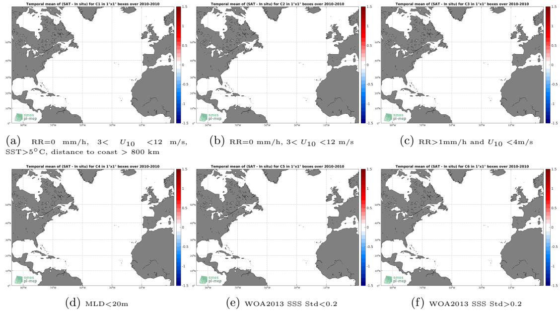
Figure 12: Temporal mean gridded over spatial boxes of size 1^{\circ}\times 1^{\circ} of \Delta\text{SSS} (SMOS L3 v2 - Daily - 0.5 Deg (CATDS-CECOS-IFREMER) - Sea mammals) for 6 different subdatasets corresponding to:RR=0 mm/h, 3 < U_{10} < 12 m/s, SST >5^{\circ}\text{C} , distance to coast > 800 km (a), RR=0 mm/h, 3 < U_{10} < 12 m/s (b), RR >1\text{mm/h} and U_{10} < 4\text{m/s} (c),MLD <20\text{m} (d),WOA2013 SSS Std <0.2 (e),WOA2013 SSS Std >0.2 (f).
