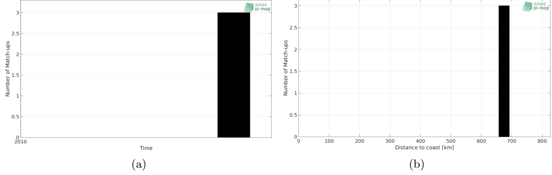
Figure 1: Number of match-ups between Sea mammals and SMOS L3 v2 - Daily - 0.5 Deg (CATDS-CECOS-IFREMER) SSS as a function of time (a) and as function of the distance to coast (b) over the North Atlantic Ocean Pi-MEP region and for the full satellite product period.
