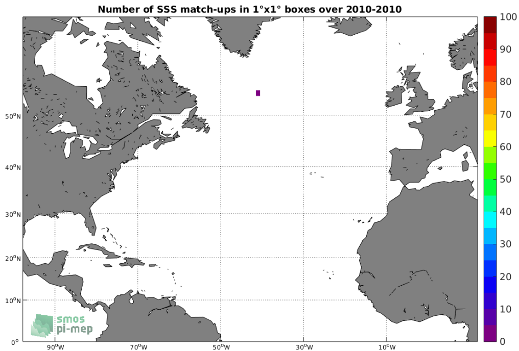
Figure 4: Number of SSS match-ups between Sea mammals SSS and the SMOS L3 v2 - Daily - 0.5 Deg (CATDS-CECOS-IFREMER) SSS product for the North Atlantic Ocean Pi-MEP region over 1^\circ \times 1^\circ boxes and for the full satellite product period.
