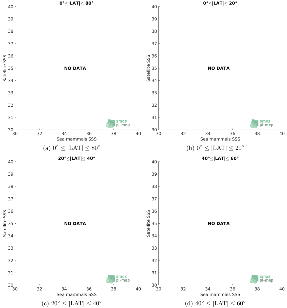
Figure 9: Contour maps of the concentration of SMOS-L3-CATDS-CECOS-IFREMER-V2-1DAY-0.5DEG SSS (y-axis) versus Sea mammals SSS (x-axis) at match-up pairs for different latitude bands. For each plot, the red line shows x=y . The black thin and dashed lines indicate a linear fit through the data cloud and the \pm 95\% confidence levels, respectively. The number match-up pairs n , the slope and R^2 coefficient of the linear fit, the root mean square (RMS) and the mean bias between satellite and in situ data are indicated for each latitude band in each plots.
