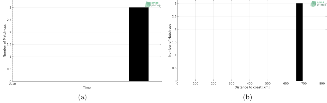
Figure 1: Number of match-ups between Sea mammals and SMOS-L3-CATDS-CECOS-IFREMER-V2-1DAY-0.5DEG SSS as a function of time (a) and as function of the distance to coast (b) over the North Atlantic Ocean Pi-MEP region and for the full satellite product period.
