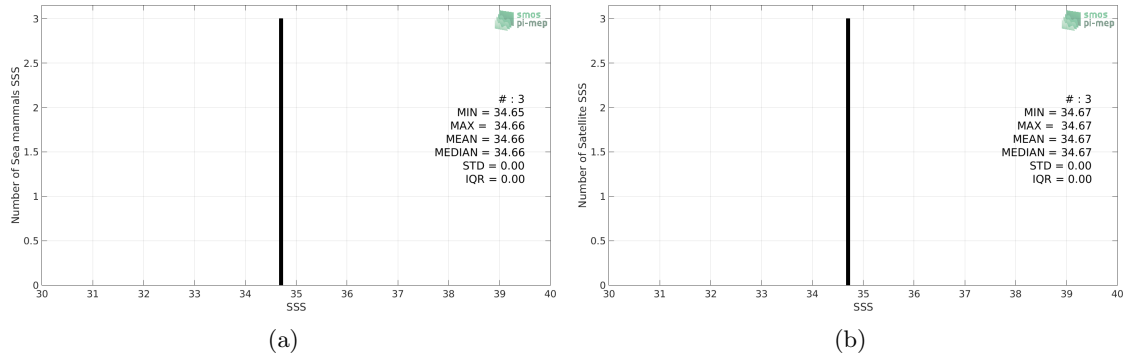
Figure 2: Histograms of SSS from Sea mammals (a) and SMOS-L3-CATDS-CECOS-IFREMER-V2-1DAY-0.5DEG (b) considering all match-up pairs per bins of 0.1 over the North Atlantic Ocean Pi-MEP region and for the full satellite product period.
