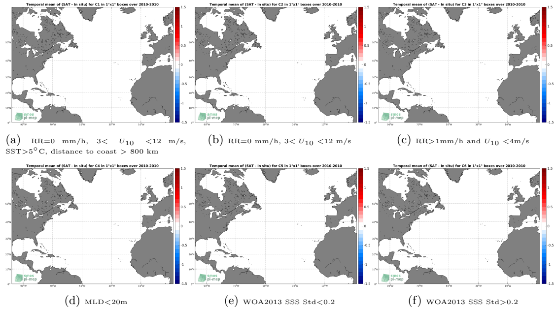
Figure 12: Temporal mean gridded over spatial boxes of size 1^\circ \times 1^\circ of \Delta SSS (SMOS-L3-CATDS-CECOS-IFREMER-V2-1DAY-0.5DEG - Sea mammals) for 6 different subdatasets corresponding to: RR=0 mm/h, 3 < U_{10} < 12 m/s, SST > 5^\circ C , distance to coast > 800 km (a), RR=0 mm/h, 3 < U_{10} < 12 m/s (b), RR > 1 mm/h and U_{10} < 4 m/s (c), MLD < 20 m (d), WOA2013 SSS Std < 0.2 (e), WOA2013 SSS Std > 0.2 (f).
