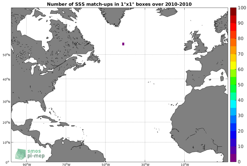
Figure 4: Number of SSS match-ups between Sea mammals SSS and the SMOS-L3-CATDS-CECOS-IFREMER-V2-1DAY-0.5DEG SSS product for the North Atlantic Ocean Pi-MEP region over 1°x1° boxes and for the full satellite product period.
