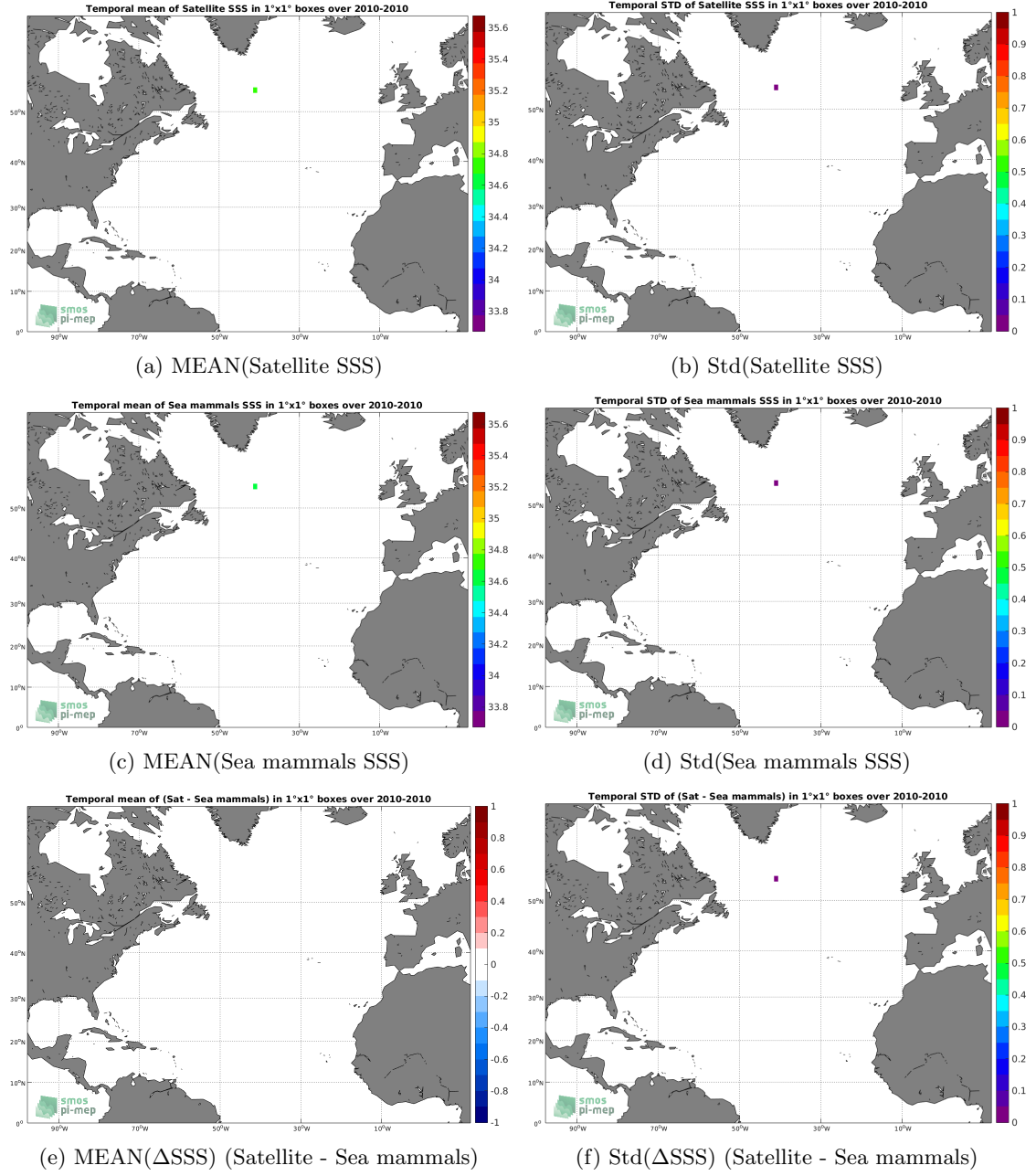
Figure 6: Temporal mean (left) and Std (right) of SSS from SMOS-L3-CATDS-CECOS-IFREMER-V2-1DAY-0.5DEG (top), Sea mammals (middle), and of \Delta SSS (Satellite - Sea mammals). Only match-up pairs are used to generate these maps.
