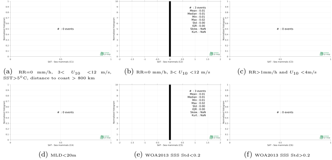
Figure 13: Normalized histogram of \Delta\text{SSS} (SMOS-L3-CATDS-CECOS-IFREMER-V2-1DAY-0.5DEG - Sea mammals) for 6 different subdatasets corresponding to: RR=0 mm/h, 3 < U_{10} < 12 m/s, SST >5^{\circ}\text{C} , distance to coast > 800 km (a), RR=0 mm/h, 3 < U_{10} < 12 m/s (b), RR>1 mm/h and U_{10} < 4 m/s (c), MLD <20 m (d), WOA2013 SSS Std <0.2 (e), WOA2013 SSS Std >0.2 (f).
