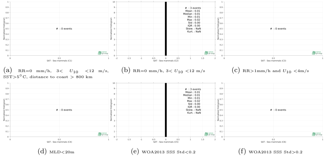
Figure 13: Normalized histogram of \Delta\text{SSS} (SMOS-L3-CATDS-CECOS-IFREMER-V2-1DAY-0.5DEG - Sea mammals) for 6 different subdatasets corresponding to: RR=0 mm/h, 3 < U_{10} < 12 m/s, SST > 5^{\circ}\text{C} , distance to coast > 800 km (a), RR=0 mm/h, 3 < U_{10} < 12 m/s (b), RR > 1 mm/h and U_{10} < 4 m/s (c), MLD < 20 m (d), WOA2013 SSS Std < 0.2 (e), WOA2013 SSS Std > 0.2 (f).
