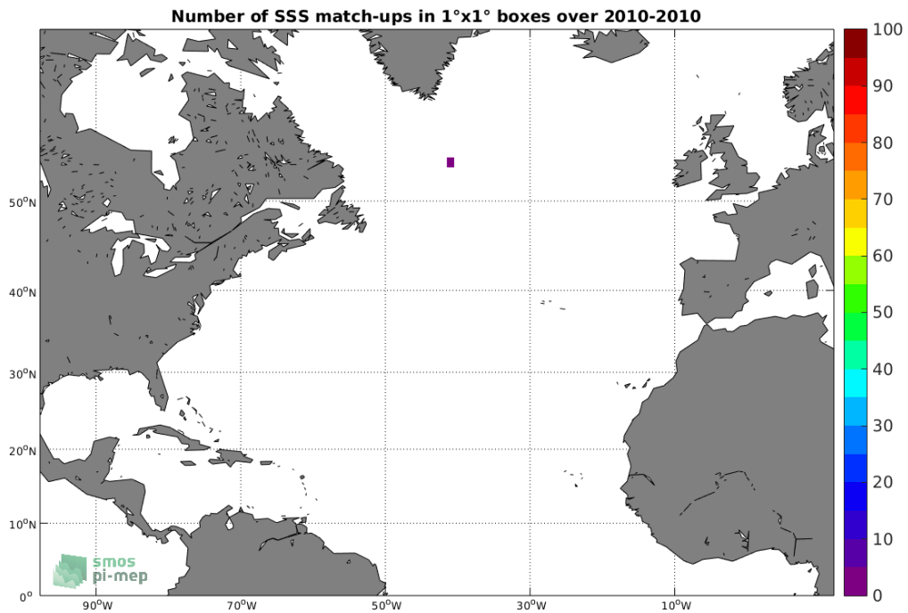
Figure 4: Number of SSS match-ups between Sea mammals SSS and the SMOS-L3-CATDS-CECOS-IFREMER-V2-1DAY-0.5DEG SSS product for the North Atlantic Ocean Pi-MEP region over 1^\circ \times 1^\circ boxes and for the full satellite product period.
