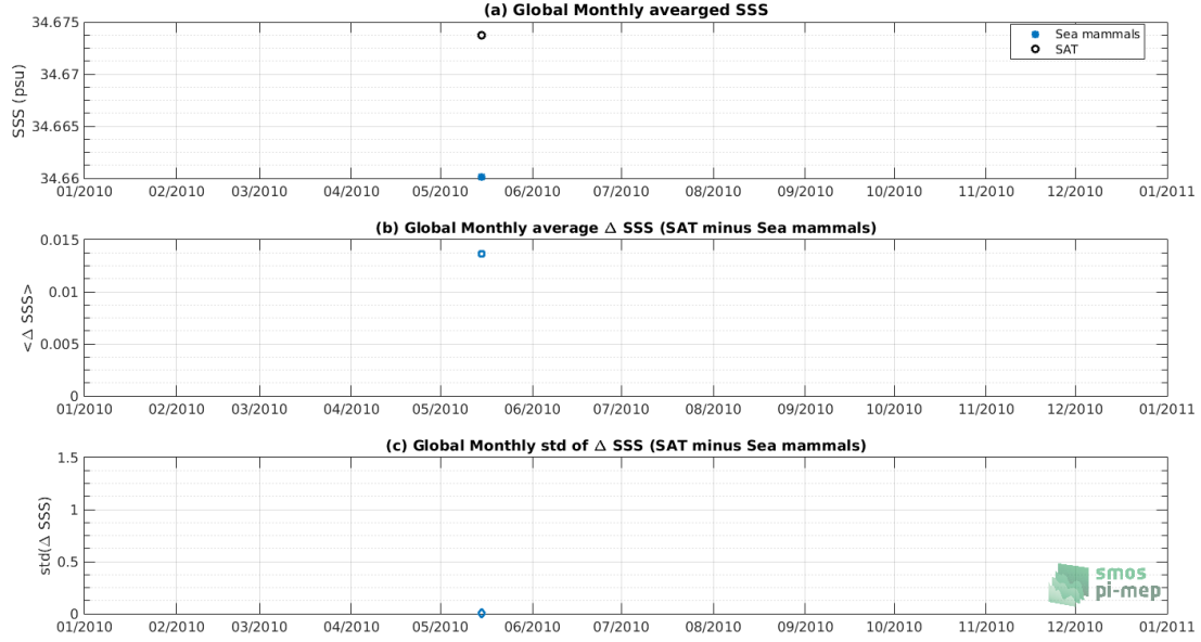
Figure 7: Time series of the monthly averaged mean SSS (top), mean \Delta SSS (Satellite - Sea mammals) and STD of \Delta SSS (Satellite - Sea mammals) over the North Atlantic Ocean Pi-MEP region considering all match-ups collected by the Pi-MEP platform.
