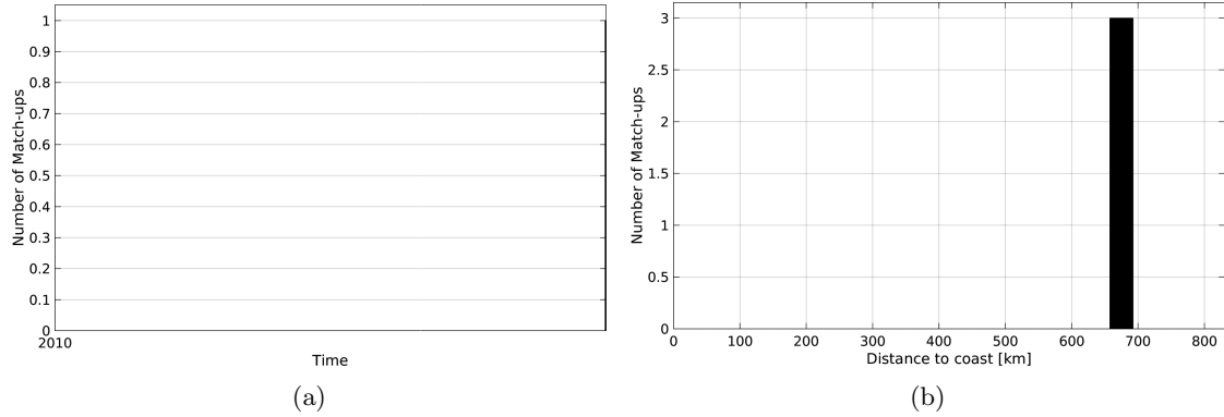
Figure 1: Number of match-ups between Sea mammals and SMOS-L3-CATDS-CECOS-IFREMER-V2-1DAY-0.5deg SSS as a function of time (a) and as function of the distance to coast (b) over the North Atlantic Ocean Pi-MEP region and for the full satellite product period.
