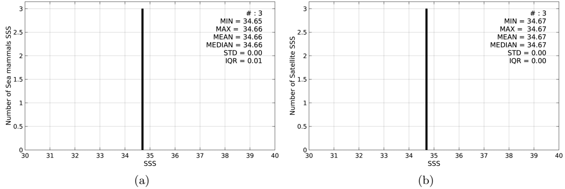
Figure 2: Histograms of SSS from Sea mammals (a) and SMOS-L3-CATDS-CECOS-IFREMER-V2-1DAY-0.5deg (b) considering all match-up pairs per bins of 0.1 over the North Atlantic Ocean Pi-MEP region and for the full satellite product period.
