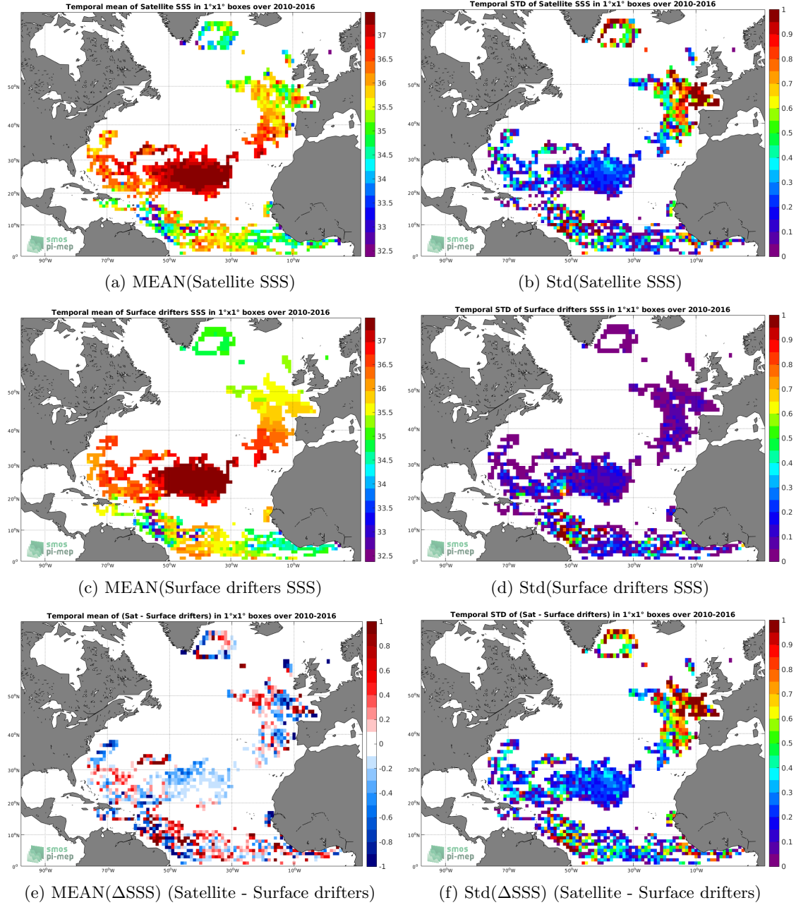
Figure 5: Temporal mean (left) and Std (right) of SSS from SMOS SSS L3 v2 - Daily - 0.5 Deg (CATDS-CECOS-IFREMER) (top), Surface drifters (middle), and of \Delta SSS (Satellite - Surface drifters). Only match-up pairs are used to generate these maps.
