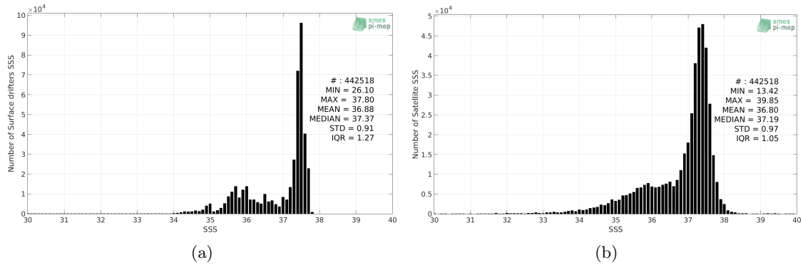
Figure 2: Histograms of SSS from Surface drifters (a) and SMOS SSS L3 v2 - Daily - 0.5 Deg (CATDS-CECOS-IFREMER) (b) considering all match-up pairs per bins of 0.1 over the North Atlantic Ocean Pi-MEP region and for the full satellite product period.
