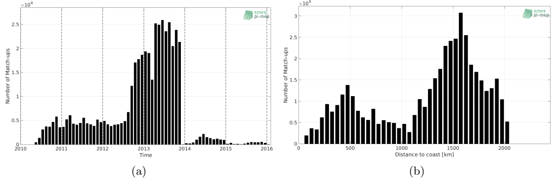
Figure 1: Number of match-ups between Surface drifters and SMOS SSS L3 v2 - Daily - 0.5 Deg (CATDS-CECOS-IFREMER) SSS as a function of time (a) and as function of the distance to coast (b) over the North Atlantic Ocean Pi-MEP region and for the full satellite product period.
