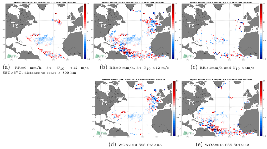
Figure 11: Temporal mean gridded over spatial boxes of size 1^\circ \times 1^\circ of \Delta SSS (SMOS SSS L3 v2 - Daily - 0.5 Deg (CATDS-CECOS-IFREMER) - Surface drifters) for 5 different subdatasets corresponding to:RR=0 mm/h, 3 < U_{10} < 12 m/s, SST >5^\circ\text{C} , distance to coast > 800 km (a), RR=0 mm/h, 3 < U_{10} < 12 m/s (b), RR >1 mm/h and U_{10} < 4 m/s (c), WOA2013 SSS Std <0.2 (d), WOA2013 SSS Std >0.2 (e).
