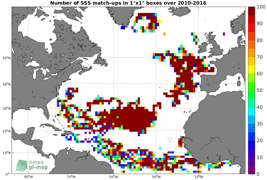
Figure 3: Number of SSS match-ups between Surface drifters SSS and the SMOS SSS L3 v2 - Daily - 0.5 Deg (CATDS-CECOS-IFREMER) SSS product for the North Atlantic Ocean Pi-MEP region over 1^\circ \times 1^\circ boxes and for the full satellite product period.
