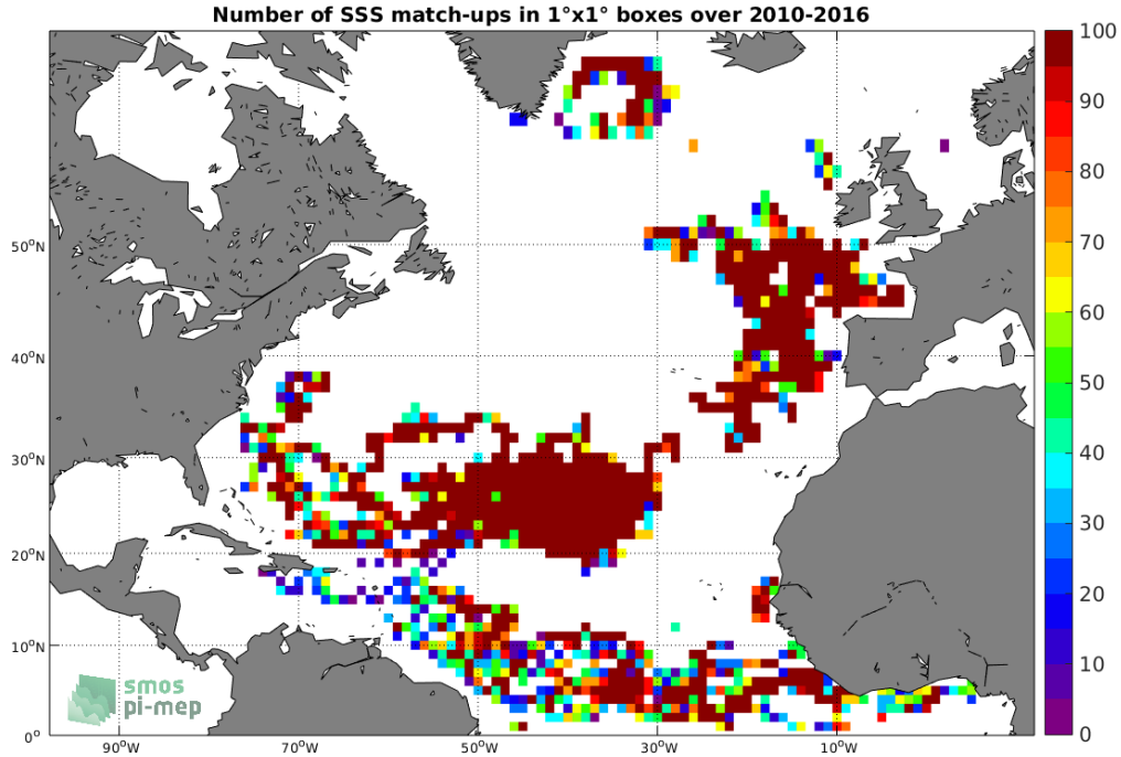
Figure 3: Number of SSS match-ups between Surface drifters SSS and the SMOS L3 v2 - Daily - 0.5 Deg (CATDS-CECOS-IFREMER) SSS product for the North Atlantic Ocean Pi-MEP region over 1^\circ \times 1^\circ boxes and for the full satellite product period.
