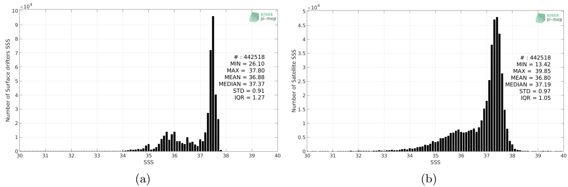
Figure 2: Histograms of SSS from Surface drifters (a) and SMOS L3 v2 - Daily - 0.5 Deg (CATDS-CECOS-IFREMER) (b) considering all match-up pairs per bins of 0.1 over the North Atlantic Ocean Pi-MEP region and for the full satellite product period.
