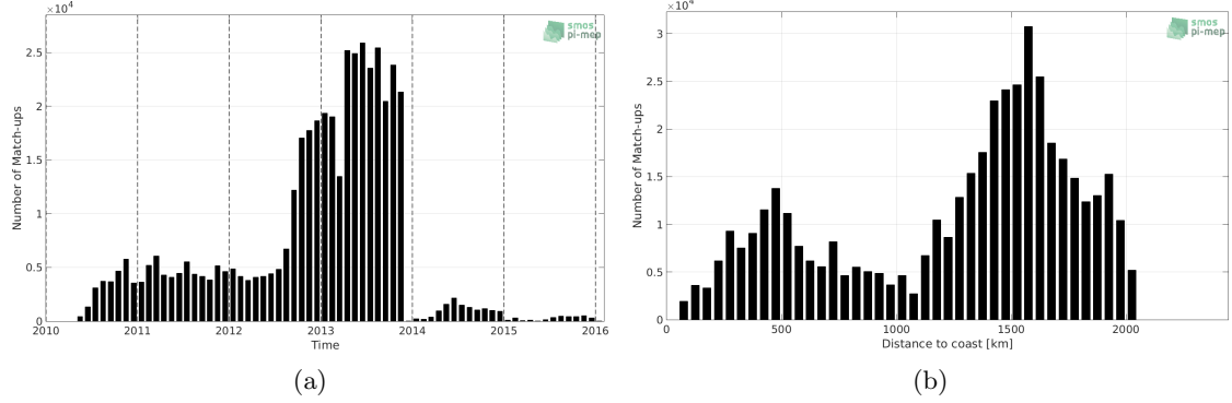
Figure 1: Number of match-ups between Surface drifters and SMOS L3 v2 - Daily - 0.5 Deg (CATDS-CECOS-IFREMER) SSS as a function of time (a) and as function of the distance to coast (b) over the North Atlantic Ocean Pi-MEP region and for the full satellite product period.
