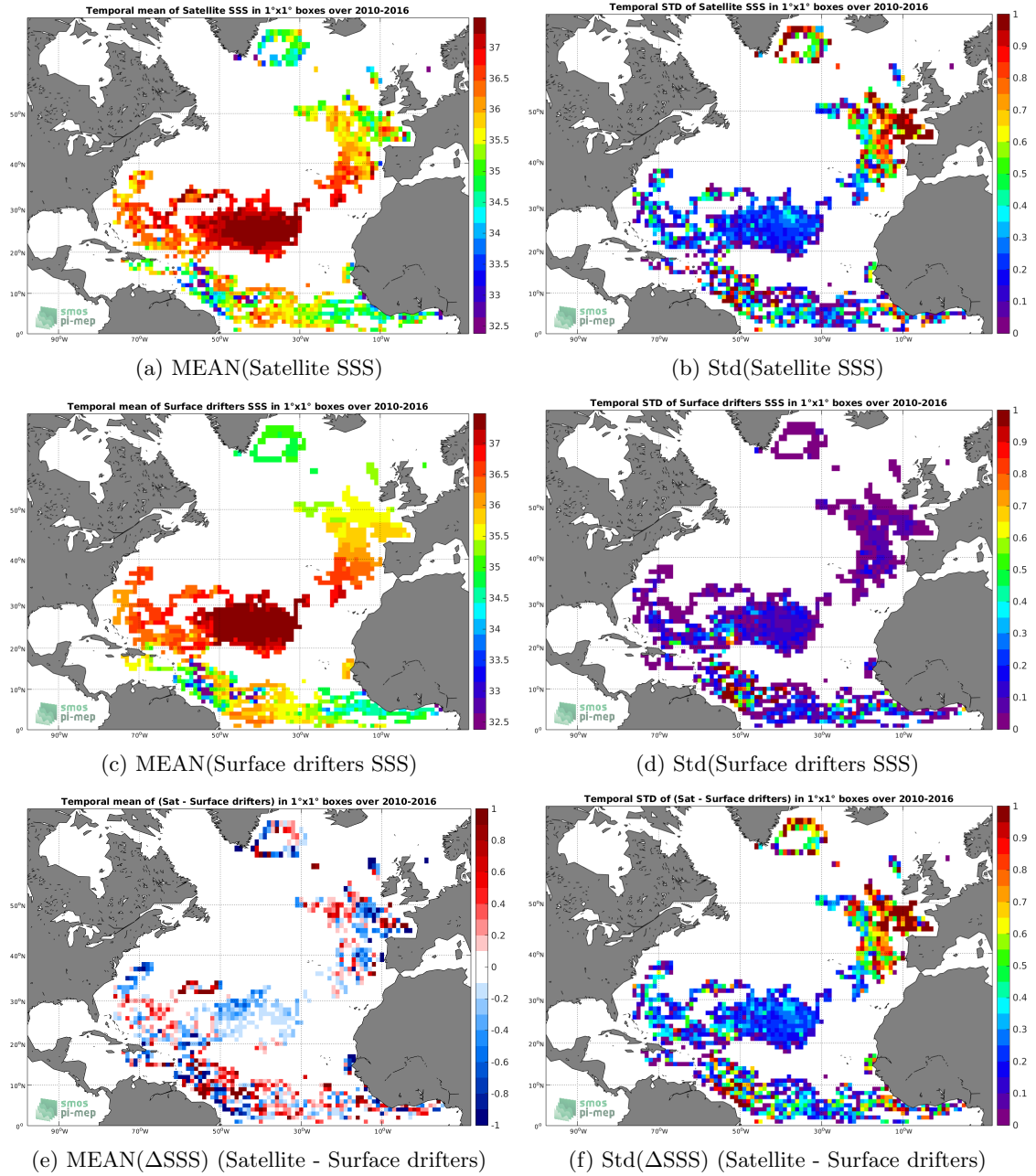
Figure 5: Temporal mean (left) and Std (right) of SSS from SMOS L3 v2 - Daily - 0.5 Deg (CATDS-CECOS-IFREMER) (top), Surface drifters (middle), and of \Delta SSS (Satellite - Surface drifters). Only match-up pairs are used to generate these maps.
