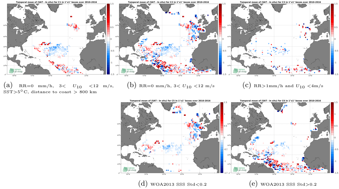
Figure 11: Temporal mean gridded over spatial boxes of size 1^\circ \times 1^\circ of \Delta SSS (SMOS L3 v2 - Daily - 0.5^\circ Deg (CATDS-CECOS-IFREMER) - Surface drifters) for 5 different subdatasets corresponding to: RR=0 mm/h, 3 < U_{10} < 12 m/s, SST > 5^\circ\text{C} , distance to coast > 800 km (a), RR=0 mm/h, 3 < U_{10} < 12 m/s (b), RR > 1 mm/h and U_{10} < 4 m/s (c), WOA2013 SSS Std < 0.2 (d), WOA2013 SSS Std > 0.2 (e).
