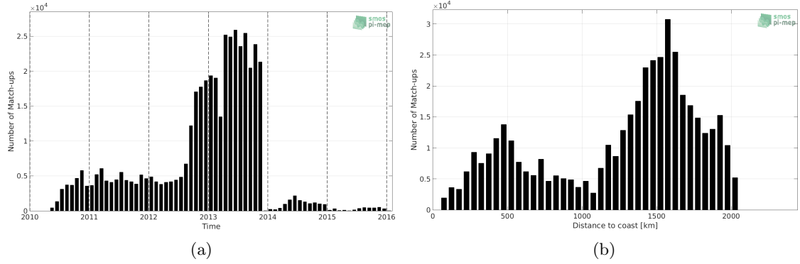
Figure 1: Number of match-ups between Surface drifters and SMOS-L3-CATDS-CECOS-IFREMER-V2-1DAY-0.5DEG SSS as a function of time (a) and as function of the distance to coast (b) over the North Atlantic Ocean Pi-MEP region and for the full satellite product period.
