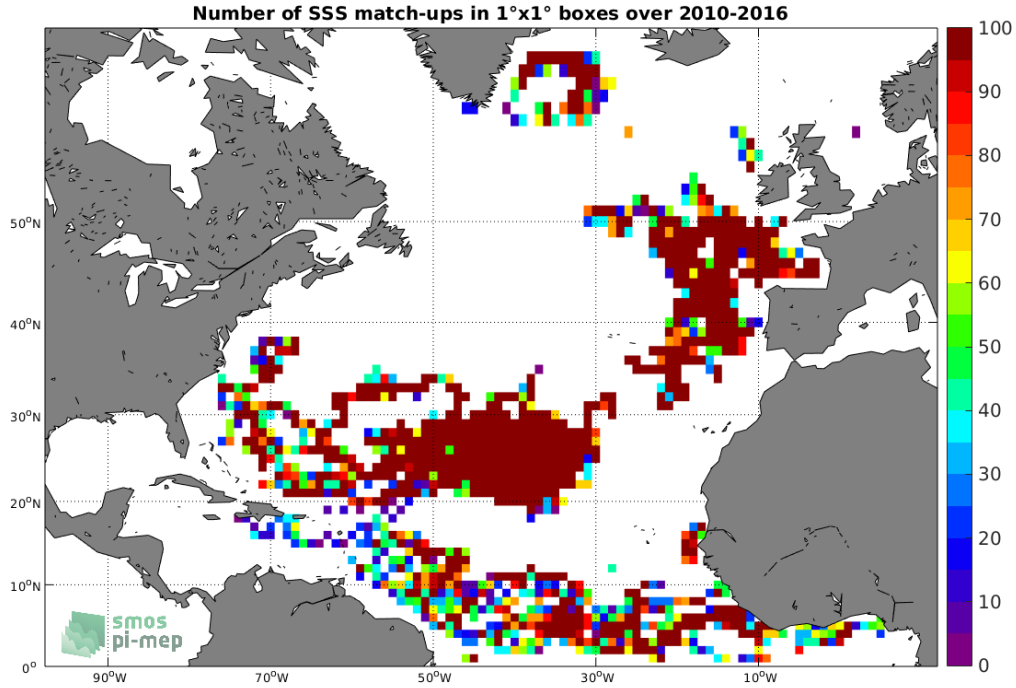
Figure 3: Number of SSS match-ups between Surface drifters SSS and the SMOS-L3-CATDS-CECOS-IFREMER-V2-1DAY-0.5DEG SSS product for the North Atlantic Ocean Pi-MEP region over 1^\circ \times 1^\circ boxes and for the full satellite product period.
