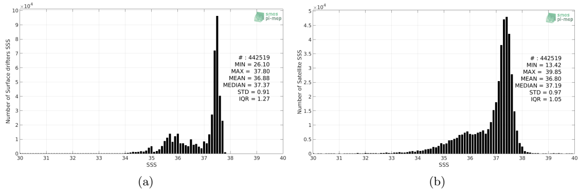
Figure 2: Histograms of SSS from Surface drifters (a) and SMOS-L3-CATDS-CECOS-IFREMER-V2-1DAY-0.5DEG (b) considering all match-up pairs per bins of 0.1 over the North Atlantic Ocean Pi-MEP region and for the full satellite product period.
