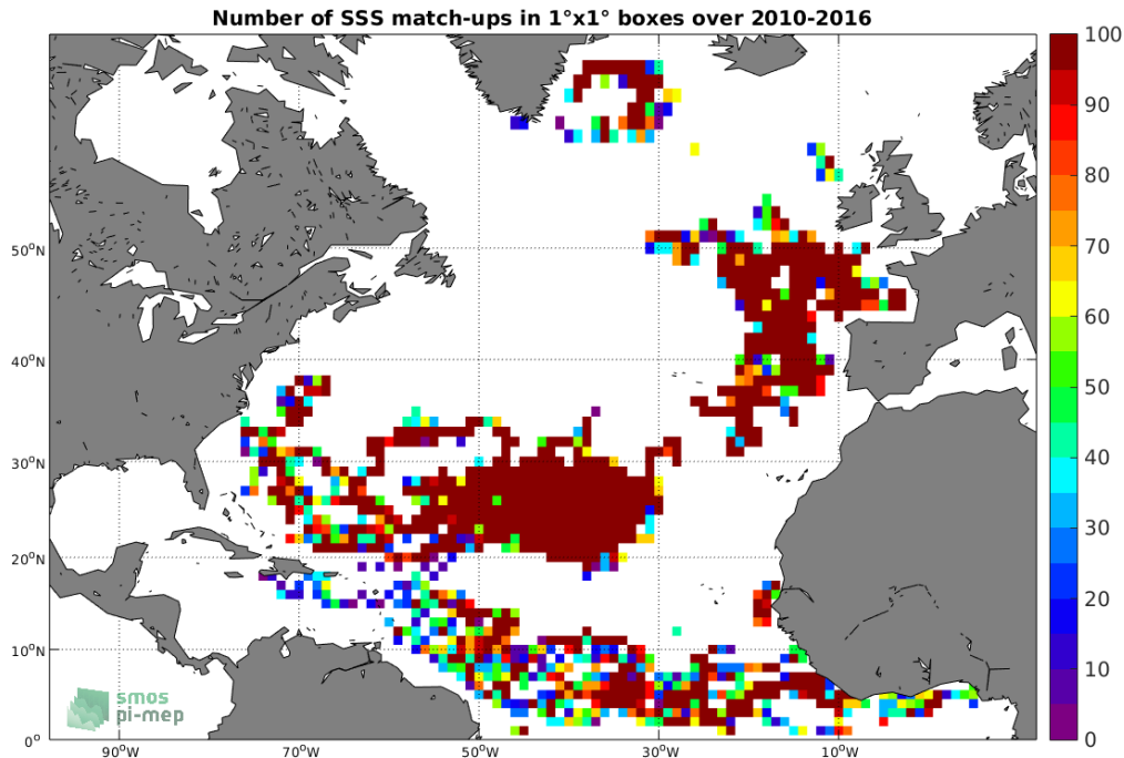
Figure 3: Number of SSS match-ups between Surface drifters SSS and the SMOS-L3-CATDS-CECOS-IFREMER-V2-1DAY-0.5DEG SSS product for the North Atlantic Ocean Pi-MEP region over 1°x1° boxes and for the full satellite product period.
