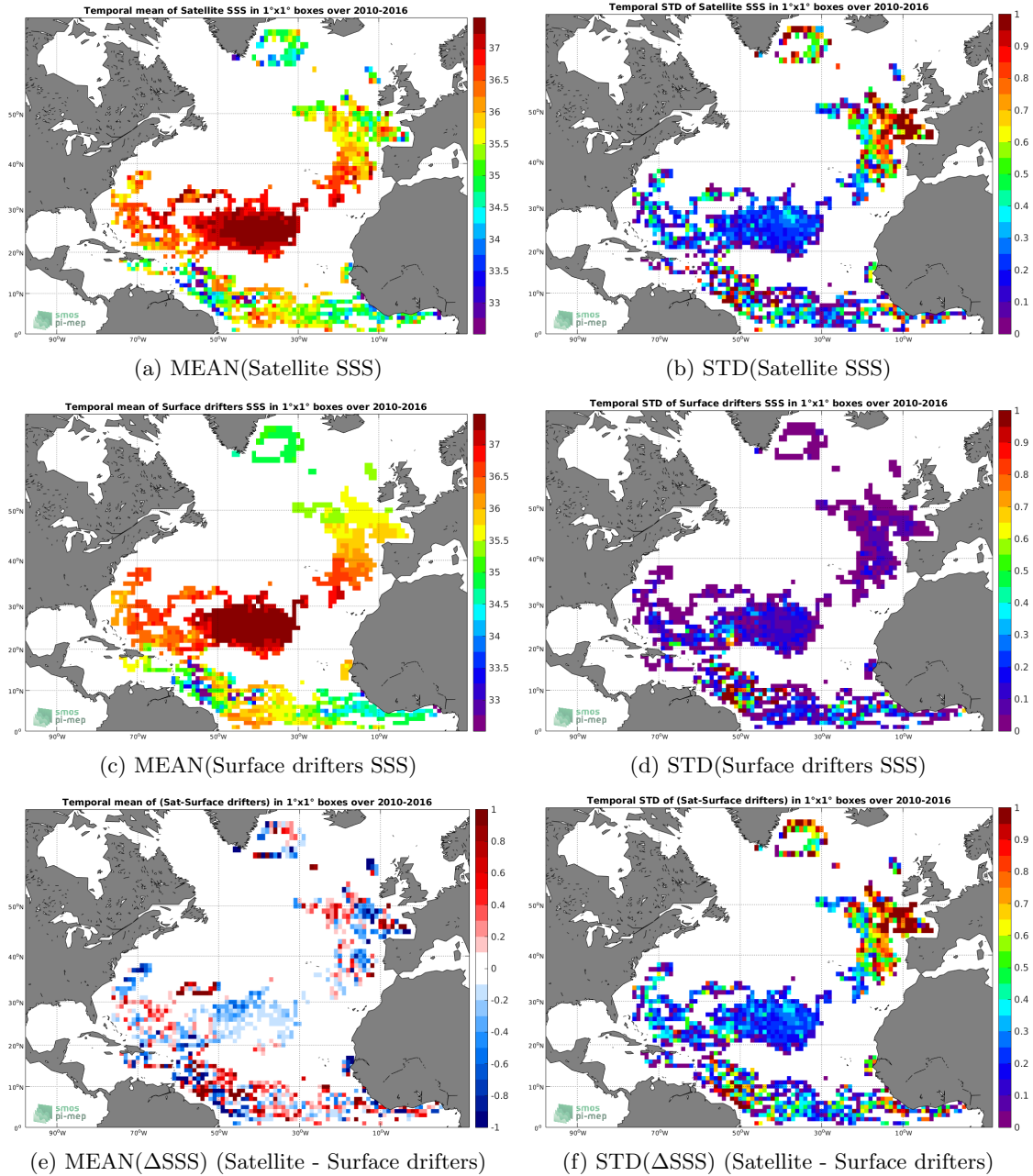
Figure 5: Temporal mean (left) and STD (right) of SSS from SMOS-L3-CATDS-CECOS-IFREMER-V2-1DAY-0.5DEG (top), Surface drifters (middle), and of \Delta SSS (Satellite - Surface drifters). Only match-up pairs are used to generate these maps.
