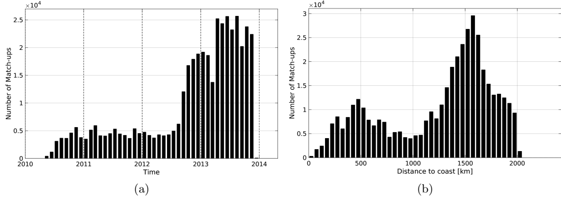
Figure 1: Number of match-ups between Surface drifters and SMOS-L3-CATDS-CECOS-IFREMER-V2-1DAY-0.5deg SSS as a function of time (a) and as function of the distance to coast (b) over the North Atlantic Ocean Pi-MEP region and for the full satellite product period.
