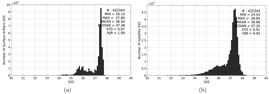
Figure 2: Histograms of SSS from Surface drifters (a) and SMOS-L3-CATDS-CECOS-IFREMER-V2-1DAY-0.5deg (b) considering all match-up pairs per bins of 0.1 over the North Atlantic Ocean Pi-MEP region and for the full satellite product period.
