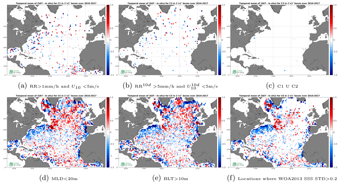
Figure 12: Temporal mean gridded over spatial boxes of size 1^\circ \times 1^\circ of \Delta\text{SSS} (SMOS-L3-CATDS-CECOS-IFREMER-V2-1DAY-0.5DEG - Argo) for 6 different subdatasets corresponding to: \text{RR} > 1\text{mm/h} and U_{10} < 5\text{m/s} (a), \text{RR}^{10d} > 5\text{mm/h} and U_{10}^{10d} < 5\text{m/s} (b), C1 U C2 (c), \text{MLD} < 20\text{m} (d), \text{BLT} > 10\text{m} (e), Locations where WOA2013 SSS STD > 0.2 (f).
