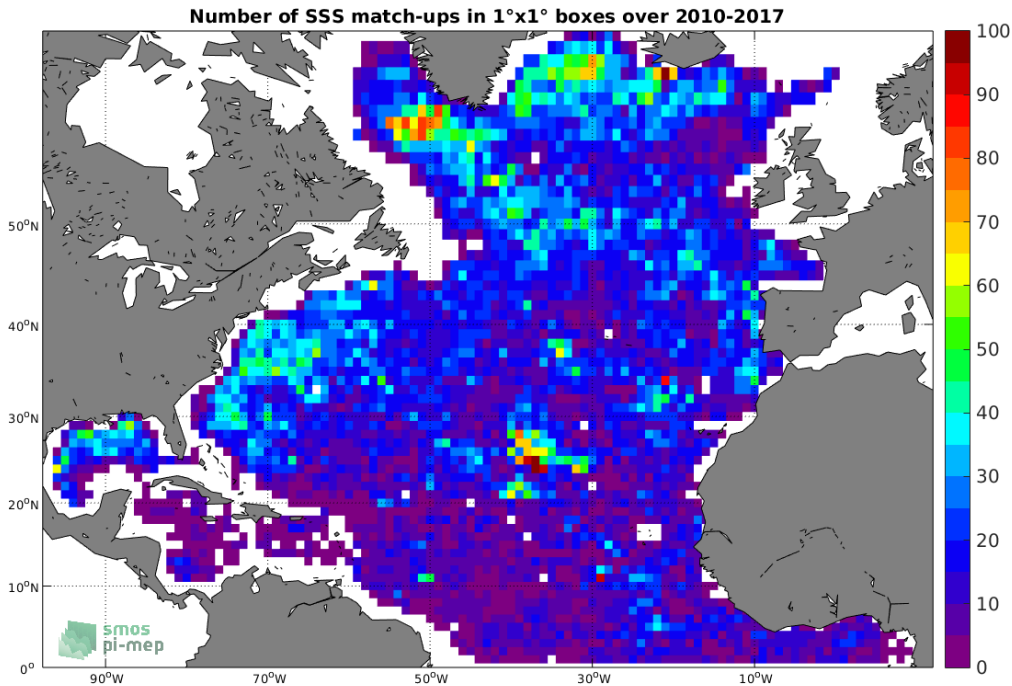
Figure 4: Number of SSS match-ups between Argo SSS and the SMOS-L3-CATDS-CECOS-IFREMER-V2-1DAY-0.5DEG SSS product for the North Atlantic Ocean Pi-MEP region over 1^\circ \times 1^\circ boxes and for the full satellite product period.
