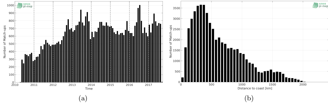
Figure 1: Number of match-ups between Argo and SMOS-L3-CATDS-CECOS-IFREMER-V2-1DAY-0.5DEG SSS as a function of time (a) and as function of the distance to coast (b) over the North Atlantic Ocean Pi-MEP region and for the full satellite product period.
