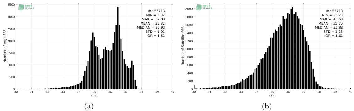
Figure 2: Histograms of SSS from Argo (a) and SMOS-L3-CATDS-CECOS-IFREMER-V2-1DAY-0.5DEG (b) considering all match-up pairs per bins of 0.1 over the North Atlantic Ocean Pi-MEP region and for the full satellite product period.
