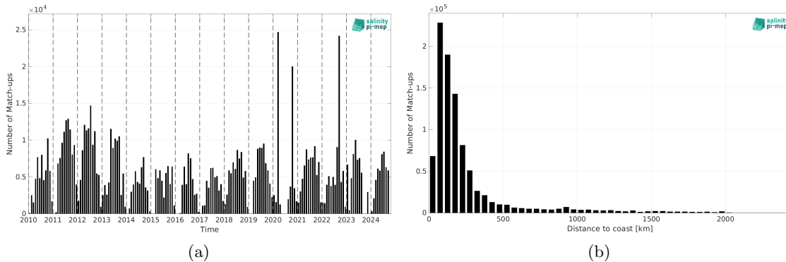
Figure 2: Number of match-ups between TSG (SAMOS) and SMOS SSS L3 v335 - Monthly - 25 km (CATDS-CPDC) SSS as a function of time (a) and as function of the distance to coast (b) over the North Atlantic Ocean Pi-MEP region and for the full satellite product period.
