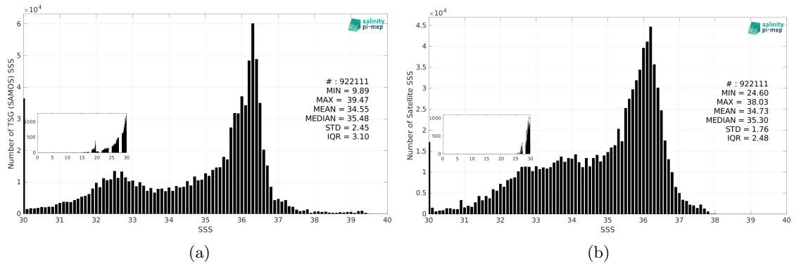
Figure 3: Histograms of SSS from TSG (SAMOS) (a) and SMOS SSS L3 v335 - Monthly - 25 km (CATDS-CPDC) (b) considering all match-up pairs per bins of 0.1 over the North Atlantic Ocean Pi-MEP region and for the full satellite product period.
