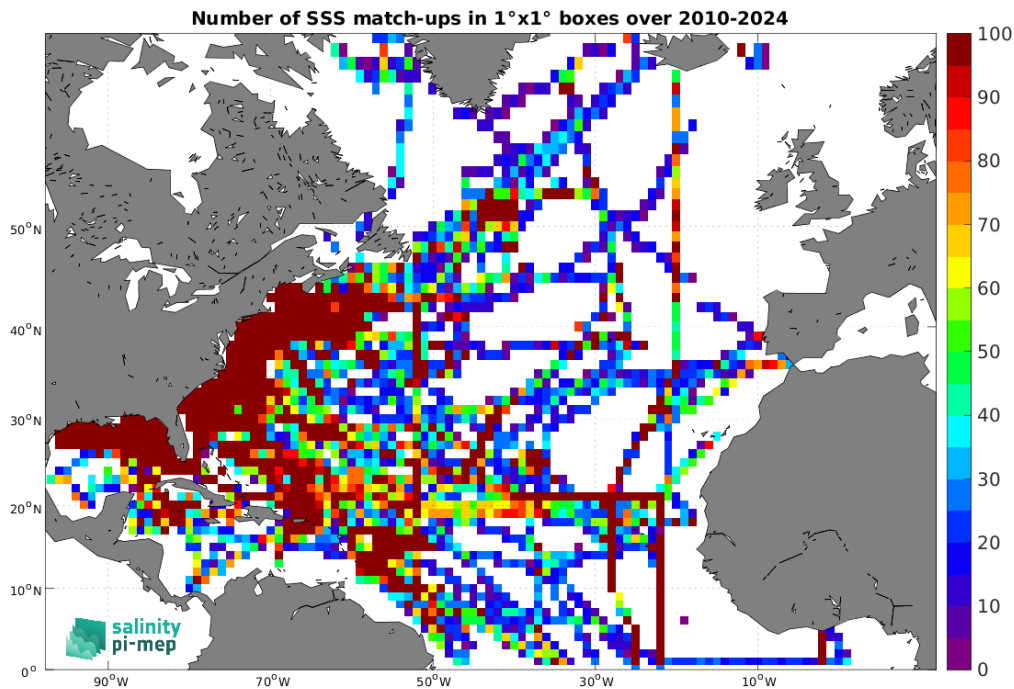
Figure 5: Number of SSS match-ups between TSG (SAMOS) SSS and the SMOS SSS L3 v335 - Monthly - 25 km (CATDS-CPDC) SSS product for the North Atlantic Ocean Pi-MEP region over 1^\circ \times 1^\circ boxes and for the full satellite product period.
